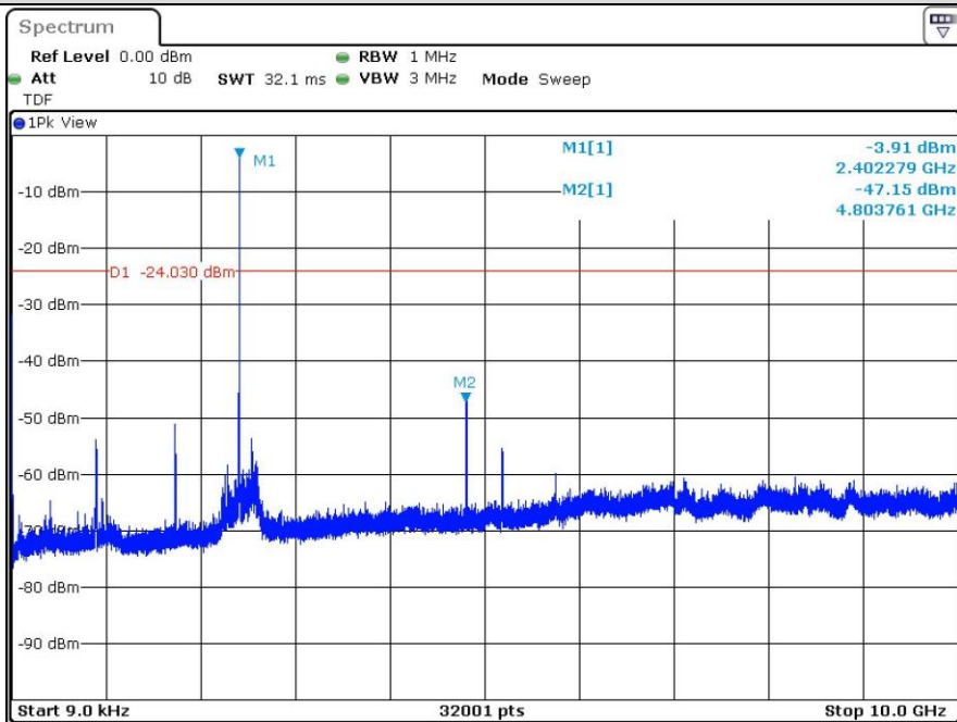
Conducted Spurious emission 9 kHz ~ 10 GHz - 2 402 MHz (1M PHY)
