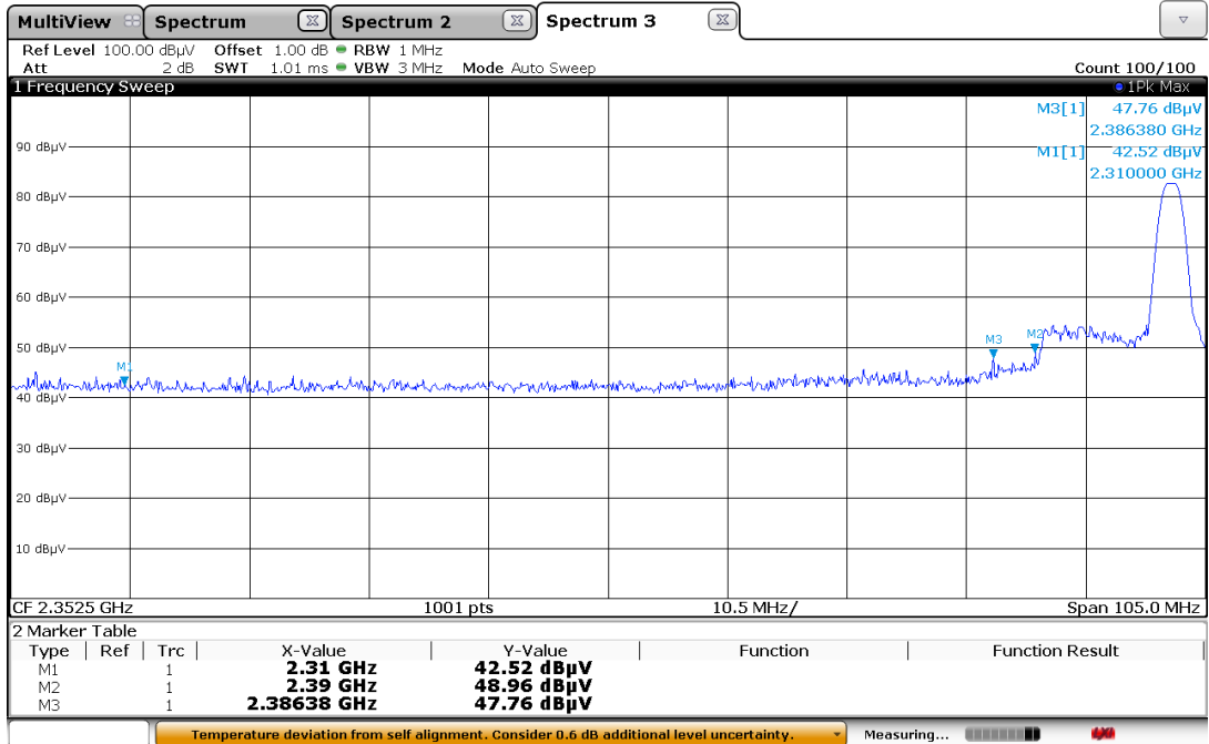
Radiated restricted band edge plot - 2 402 MHz (Peak)
