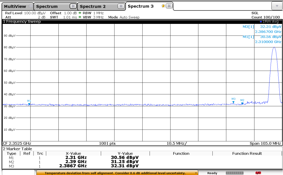
Radiated restricted band edge plot - 2 402 MHz (Average)
