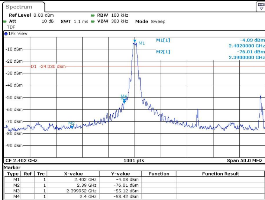
Conducted band edge plot - 2 402 MHz (1M PHY)
