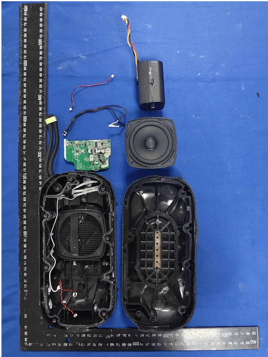
Internal photograph of EUT
