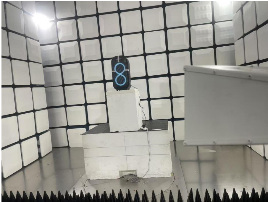
Above 1GHz-BT/2.4G ISM Band
