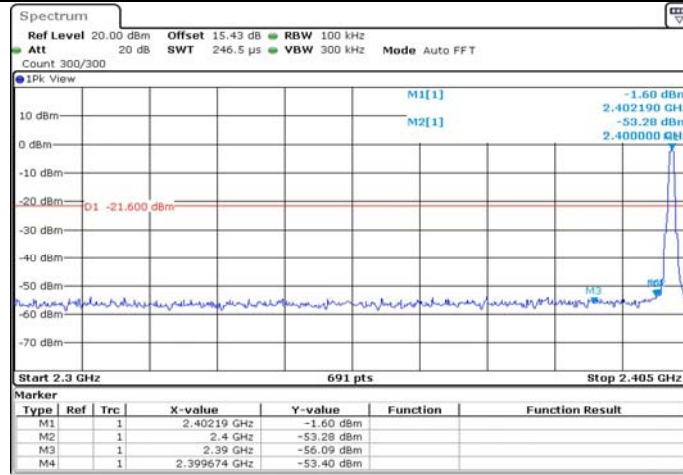
BLE_1M_Ant1_Low_2402
