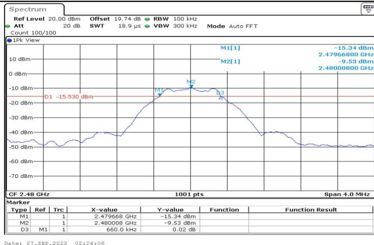
BLE_1M_Ant1_2480
