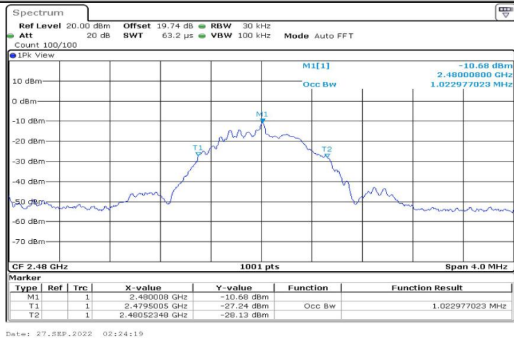
BLE_1M_Ant1_2480
