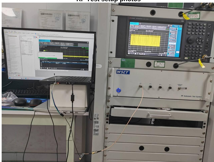
RF Test setup photos
