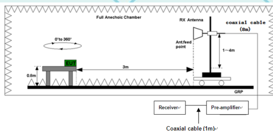
Above 1GHz
