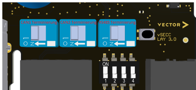
Figure 13: vSECC connector: DIP Switches
