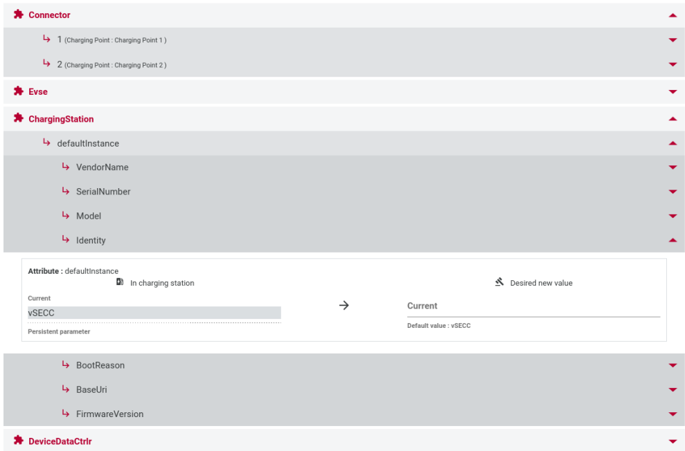
Figure 18: vCharM Charging Station Configuration
