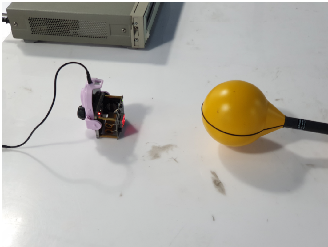
Measurement distance from the EUT
