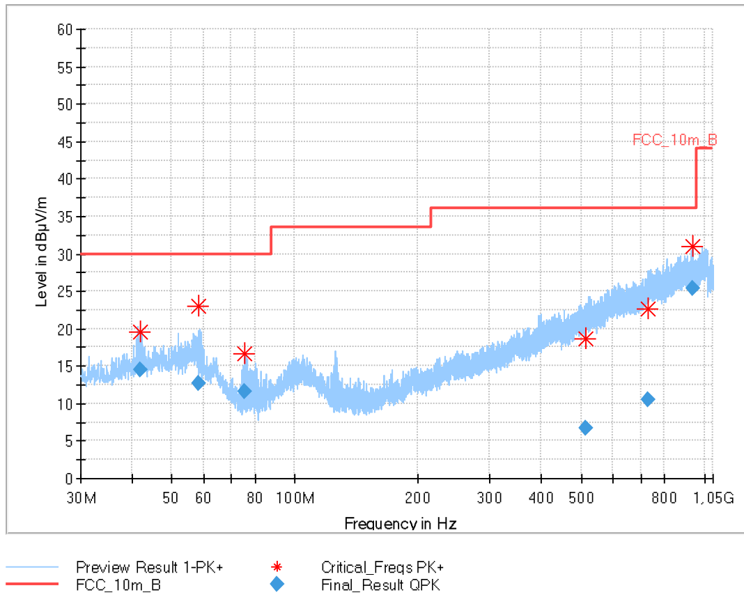
Plot 4: 30 MHz – 1 GHz, vertical and horizontal polarization
