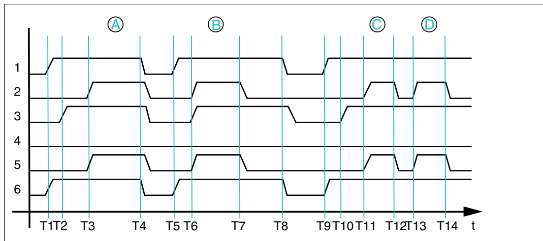
Figure 7.3 Timing sequence of bits in byte 0
