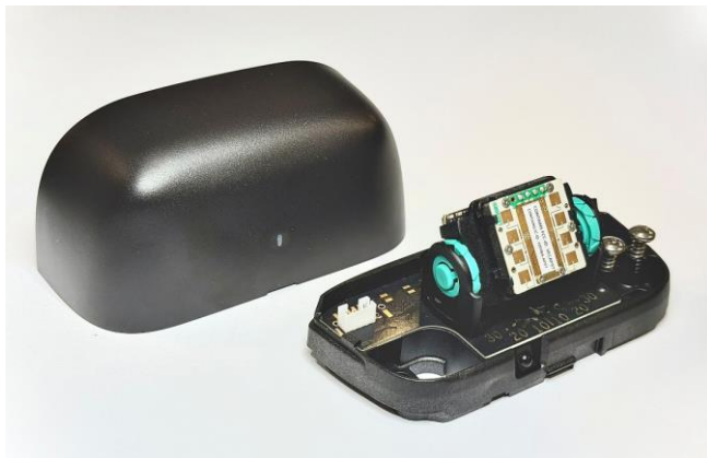
Fig. 2. Radar Cover and Assembly (Left View)
