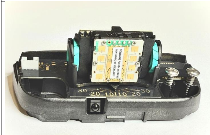
Fig. 6. Racon-D-NA (Front View) fully assembled
