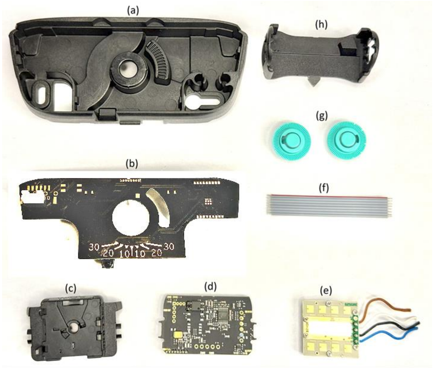
Fig. 8. Racon-D-NA Disassembled (Top View)
