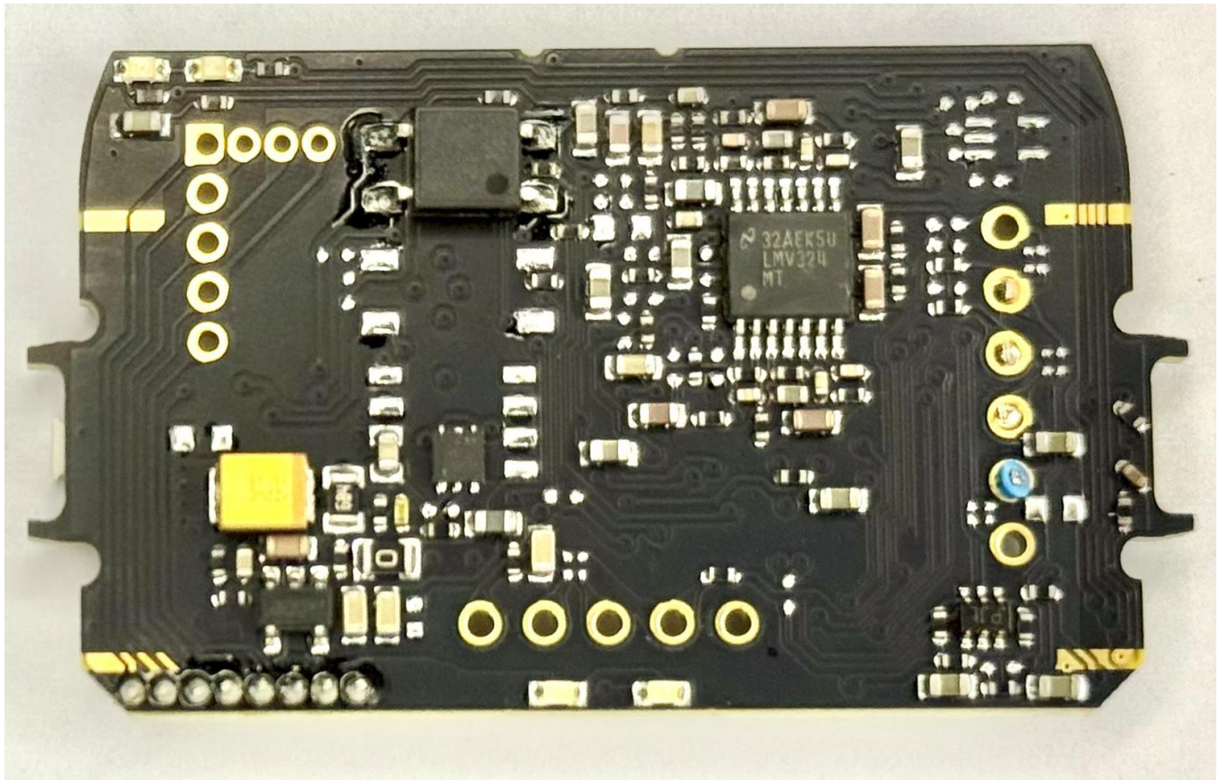
Fig. 10. Racon-D-NA Mainboard (Radar Front Side)
