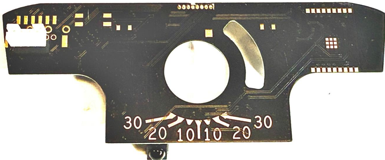
Fig. 12. Racon-D-NA Powerboard (Top)
