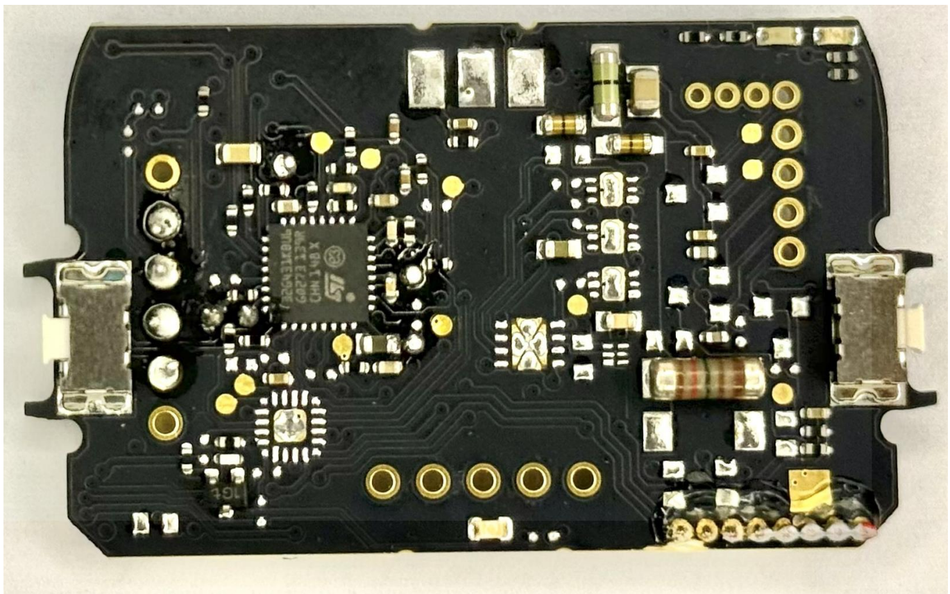
Fig. 11. Racon-D-NA Mainboard (MCU Back Side)
