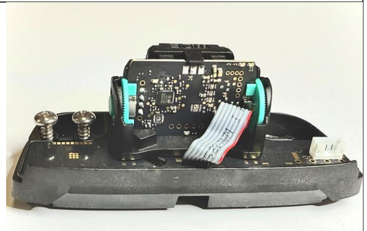
Fig. 7. Racon-D-NA (Back View) fully assembled
