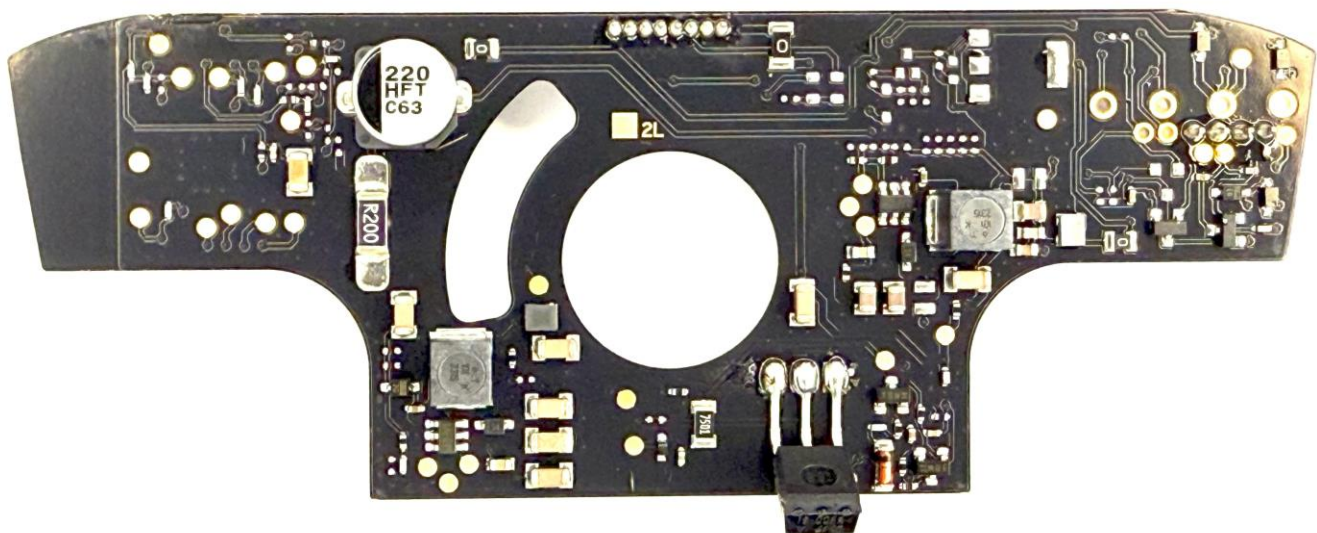
Fig. 13. Racon-D-NA Powerboard (Bottom)
