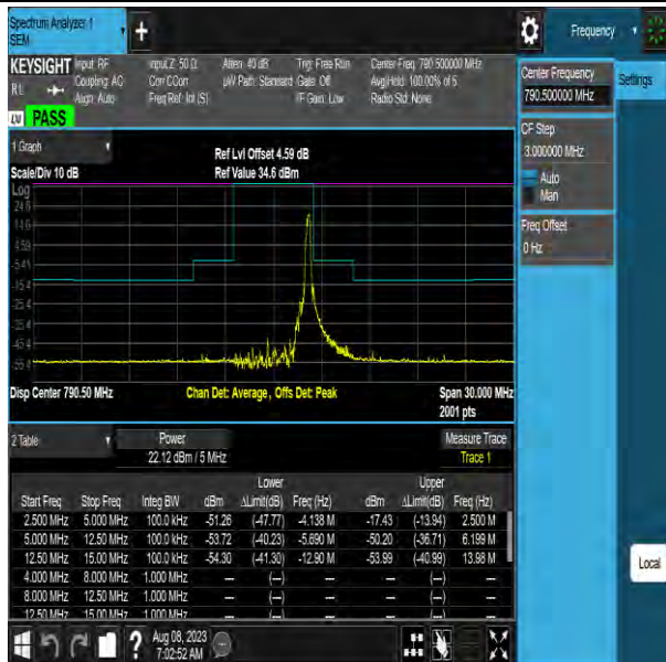
NTNV-Band14-5MHz-64QAM-23305-1RB#24--12.50--5.00-PASS
