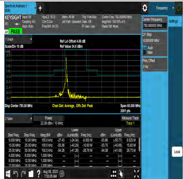
NTNV-Band14-10MHz-64QAM-23330-1RB#0--10.00--5.00-
