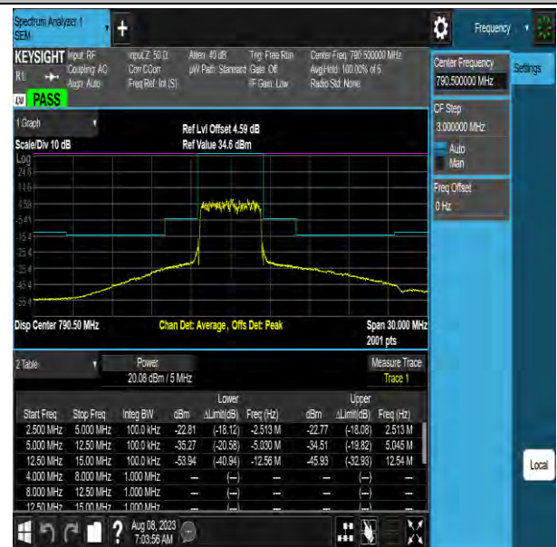
NTNV-Band14-5MHz-64QAM-23305-25RB#0--12.50--5.00-PASS
