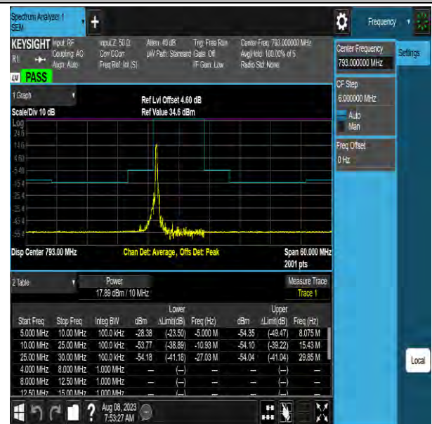
NTNV-Band14-10MHz-64QAM-23330-1RB#0--25.00--10.00-
