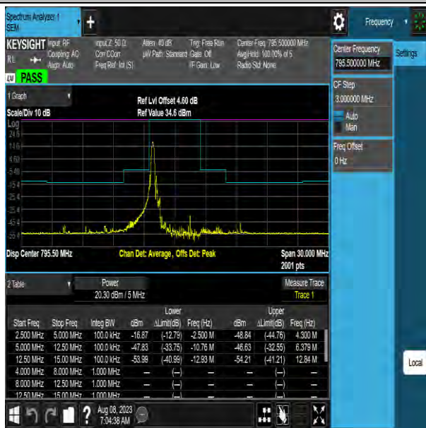
NTNV-Band14-5MHz-16QAM-23355-1RB#0-12.50-15.00-PASS
