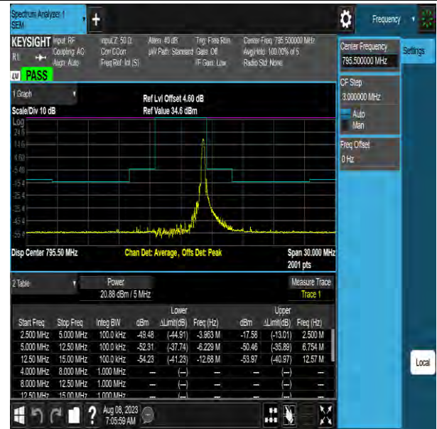
NTNV-Band14-5MHz-64QAM-23355-1RB#24--15.00--12.50-PASS
