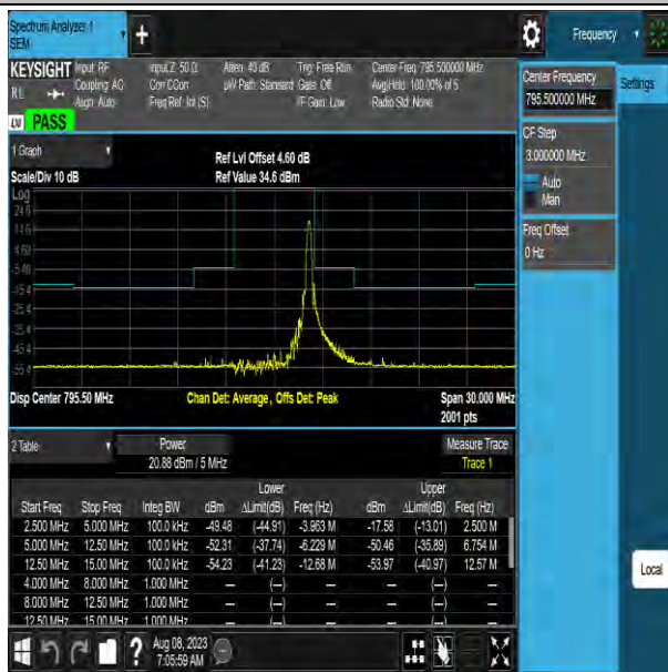
NTNV-Band14-5MHz-64QAM-23355-1RB#24-12.50-15.00-PASS
