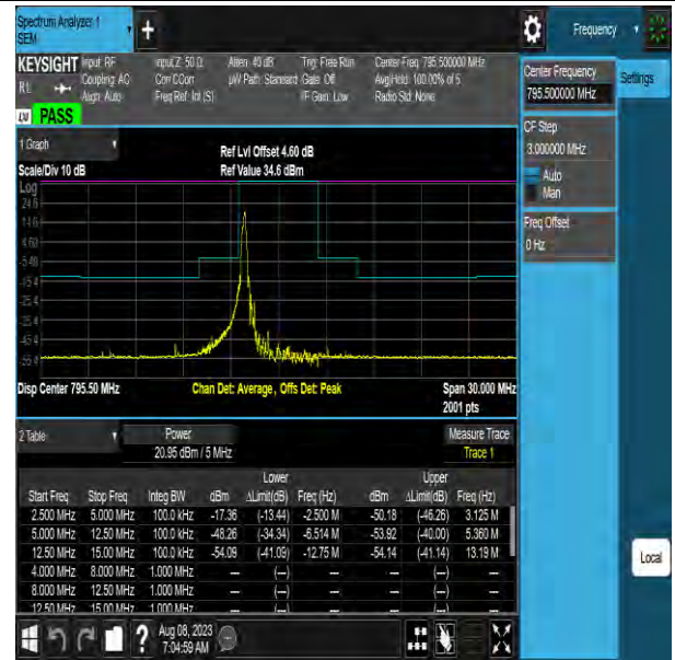
NTNV-Band14-5MHz-64QAM-23355-1RB#0--12.50--5.00-PASS
