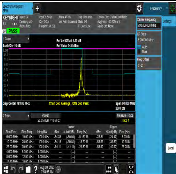
NTNV-Band14-10MHz-64QAM-23330-1RB#49-25.00-30.00- PASS
