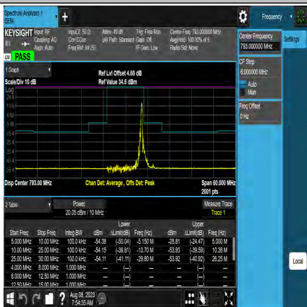
NTNV-Band14-10MHz-64QAM-23330-1RB#49-25.00-30.00- PASS
