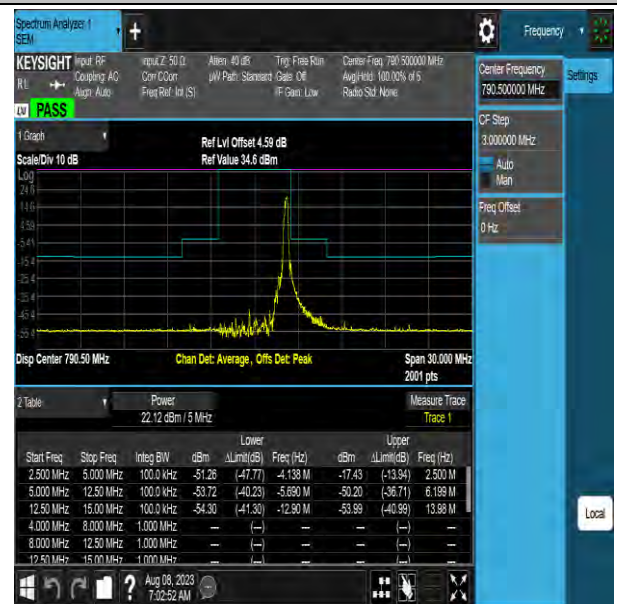
NTNV-Band14-5MHz-QPSK-23305-25RB#0-2.50-5.00-PASS
