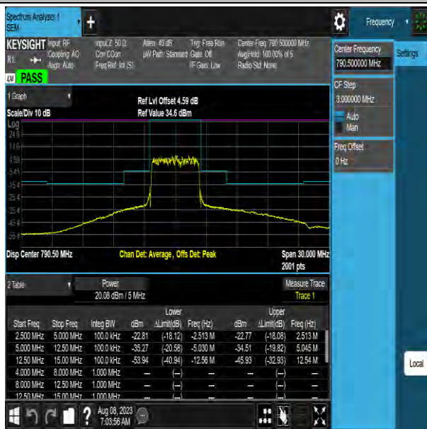
NTNV-Band14-5MHz-64QAM-23305-25RB#0-12.50-15.00-PASS
