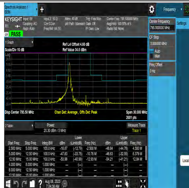
NTNV-Band14-5MHz-16QAM-23355-1RB#0--12.50--5.00-PASS
