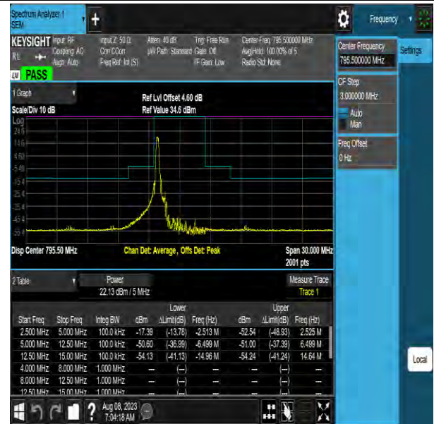
NTNV-Band14-5MHz-QPSK-23355-1RB#0--12.50--5.00-PASS
