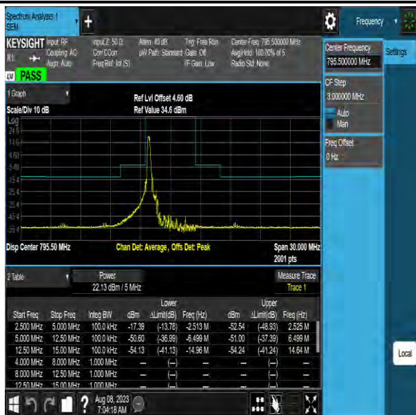
NTNV-Band14-5MHz-QPSK-23355-1RB#0-12.50-15.00-PASS
