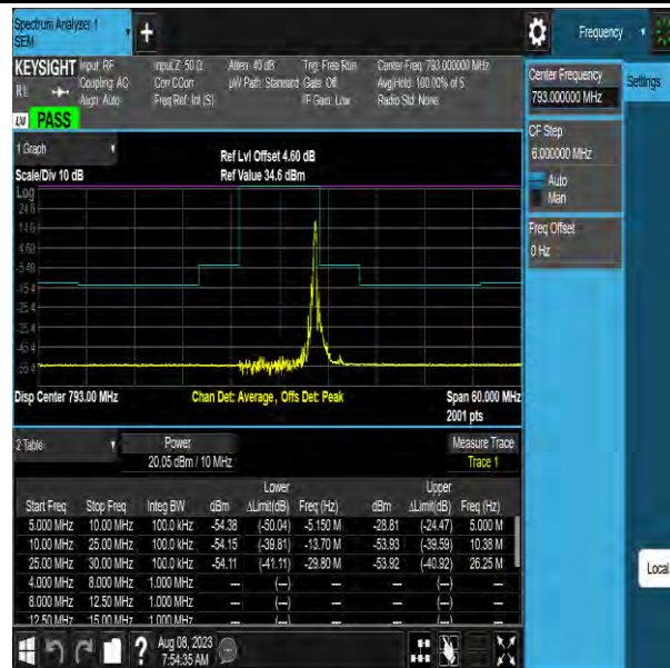
NTNV-Band14-10MHz-QPSK-23330-50RB#0--10.00--5.00- PASS
