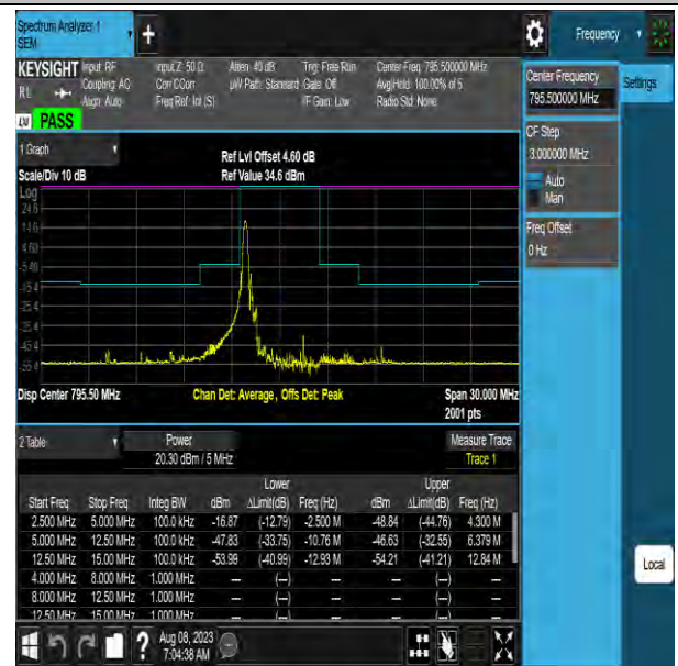
NTNV-Band14-5MHz-64QAM-23355-1RB#0--5.00--2.50-PASS
