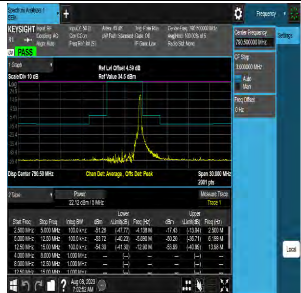
NTNV-Band14-5MHz-64QAM-23305-1RB#24-5.00-12.50-PASS
