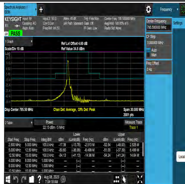
NTNV-Band14-5MHz-16QAM-23355-1RB#0--5.00--2.50-PASS
