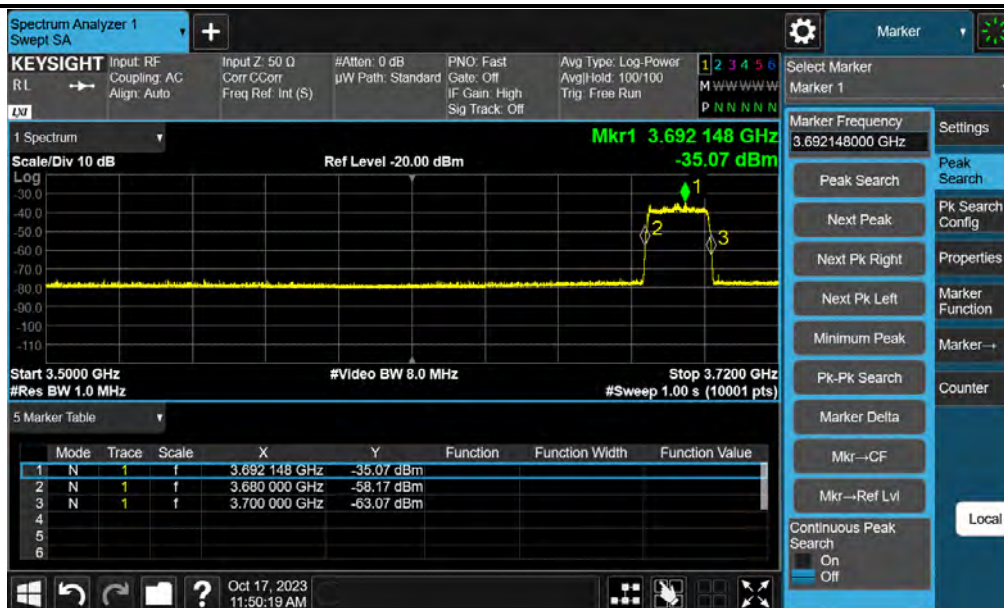
Band48-20MHz-CH56640_Idle With 10s
