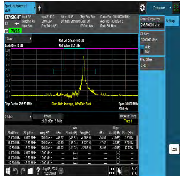
NTNV-Band14-5MHz-64QAM-23355-1RB#24--5.00--2.50-PASS
