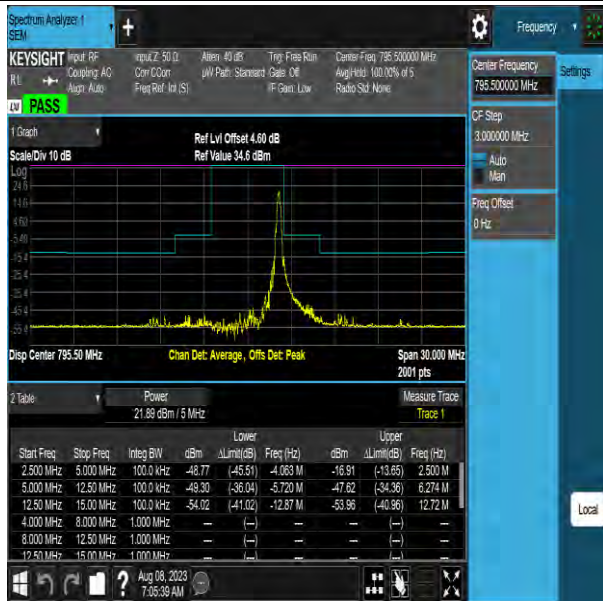
NTNV-Band14-5MHz-16QAM-23355-1RB#24-12.50-15.00- PASS
