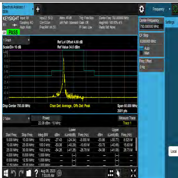
NTNV-Band14-10MHz-64QAM-23330-1RB#0-5.00-10.00-PASS
