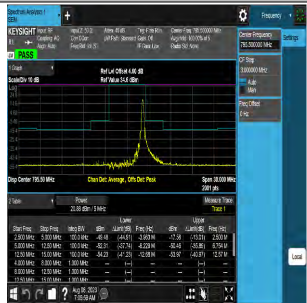
NTNV-Band14-5MHz-64QAM-23355-1RB#24--15.00--12.50-PASS
