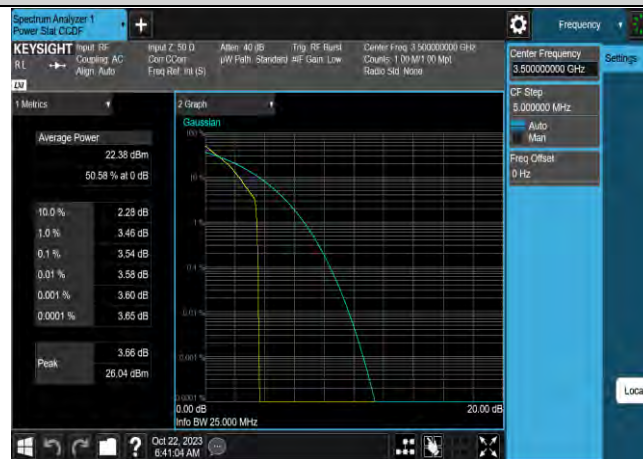
Band42-20MHz-QPSK-42590-100RB#0
