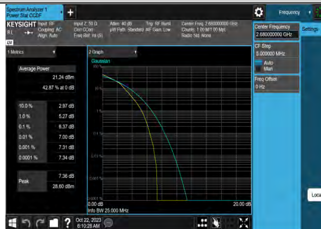
Band41-20MHz-16QAM-41490-100RB#0
