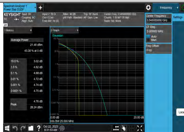
Band42-10MHz-16QAM-43040-50RB#0
