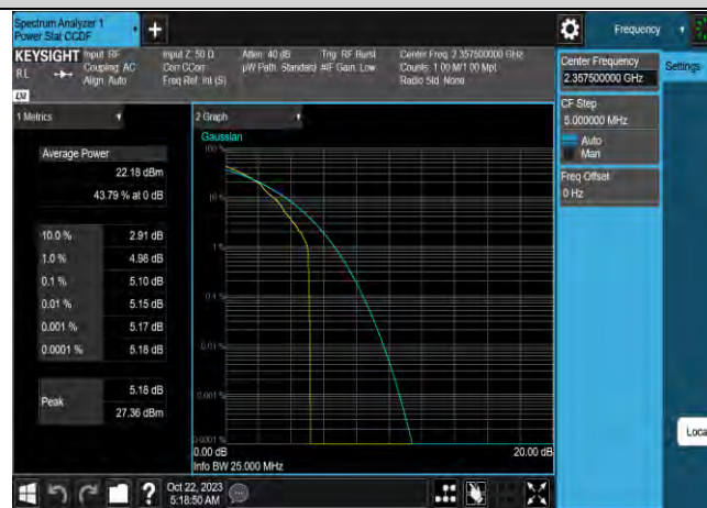
Band40-5MHz-16QAM-39225-25RB#0
