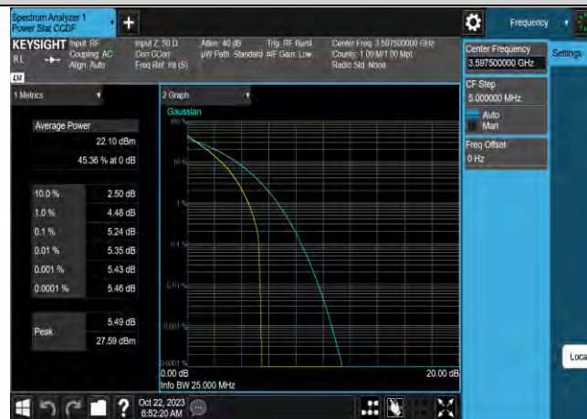
Band42-5MHz-64QAM-43115-1RB#0
