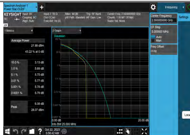
Band41-10MHz-64QAM-40620-50RB#0
