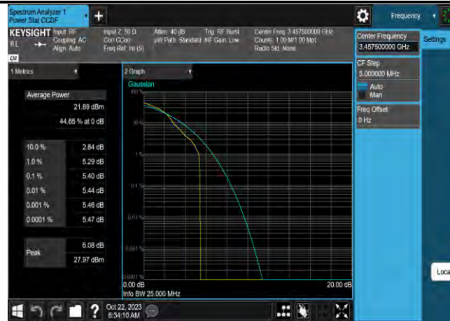
Band42-15MHz-64QAM-42165-75RB#0
