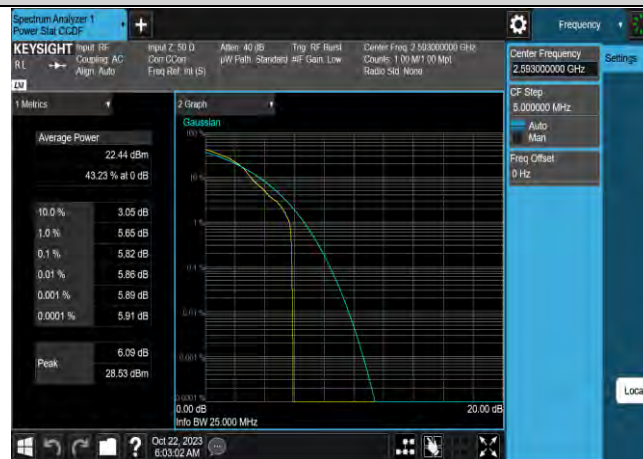
Band41-15MHz-64QAM-40620-75RB#0
