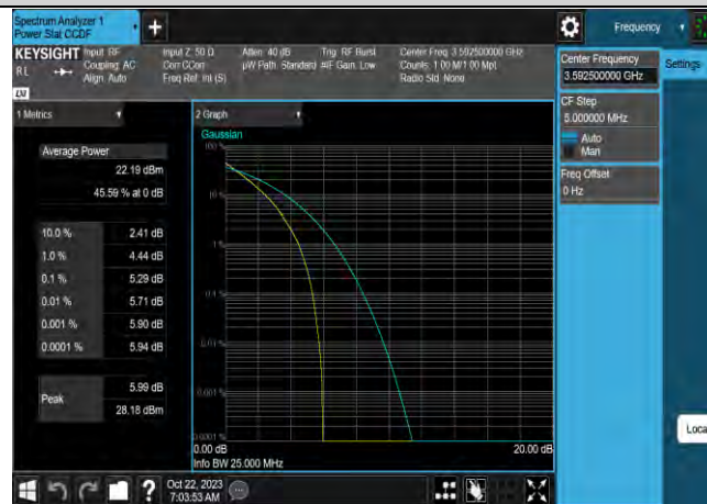
Band42-15MHz-64QAM-43165-1RB#0
