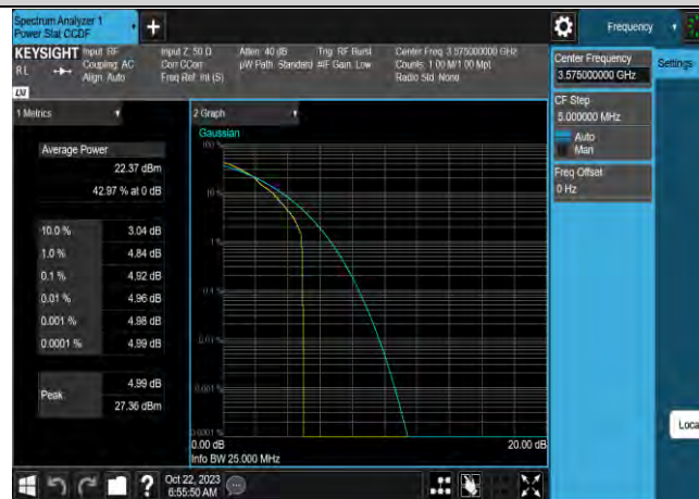
Band42-10MHz-16QAM-43340-50RB#0
