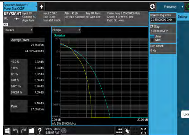
Band40-5MHz-16QAM-39225-1RB#0
