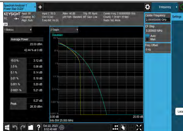
Band41-15MHz-16QAM-40620-75RB#0
