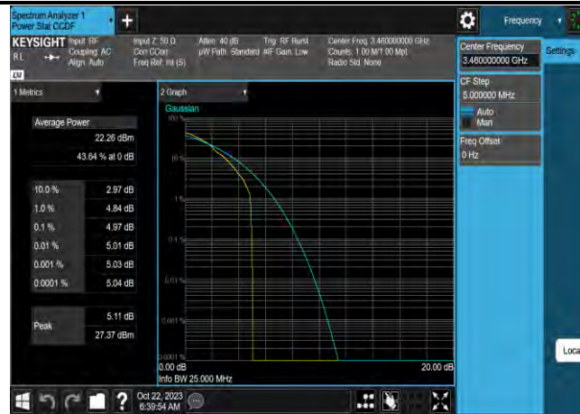
Band42-20MHz-16QAM-42190-100RB#0
