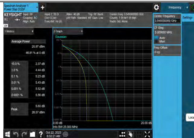
Band42-10MHz-64QAM-42140-1RB#0
