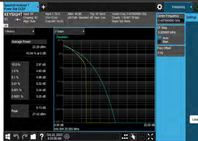
Band42-15MHz-16QAM-42165-75RB#0
