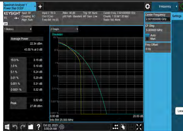
Band41-10MHz-16QAM-39700-50RB#0
