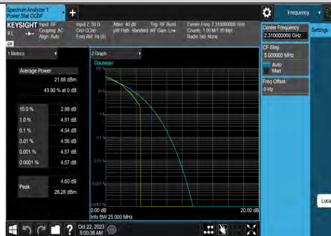
Band40-5MHz-16QAM-38750-25RB#0
