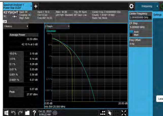
Band41-20MHz-16QAM-40620-100RB#0
