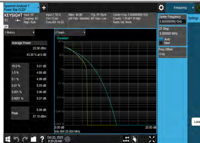
Band42-10MHz-16QAM-42590-50RB#0
