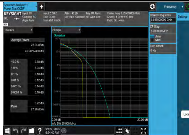
Band42-10MHz-64QAM-43140-50RB#0
