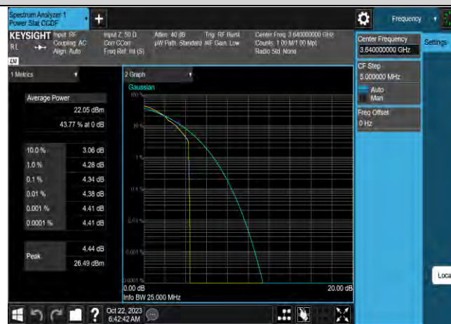
Band42-20MHz-16QAM-43990-100RB#0
