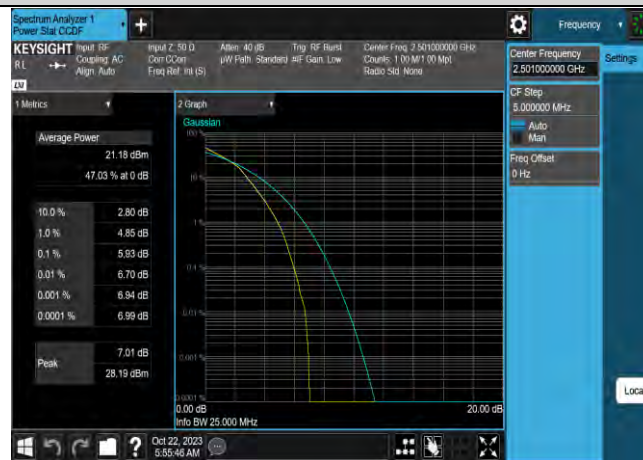
Band41-10MHz-16QAM-40620-1RB#0
