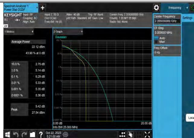
Band40-10MHz-64QAM-39200-50RB#0
