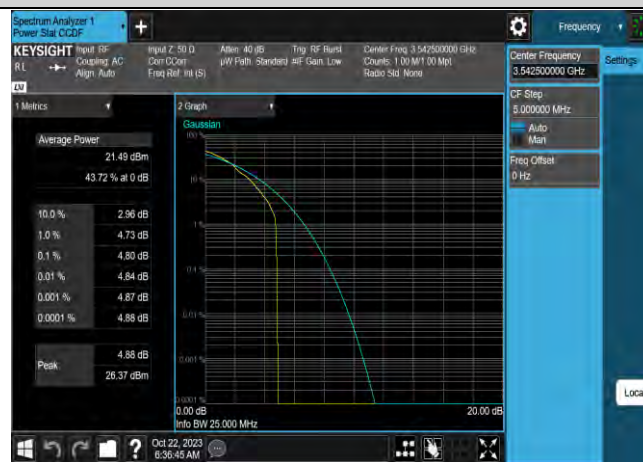
Band42-15MHz-16QAM-43015-75RB#0
