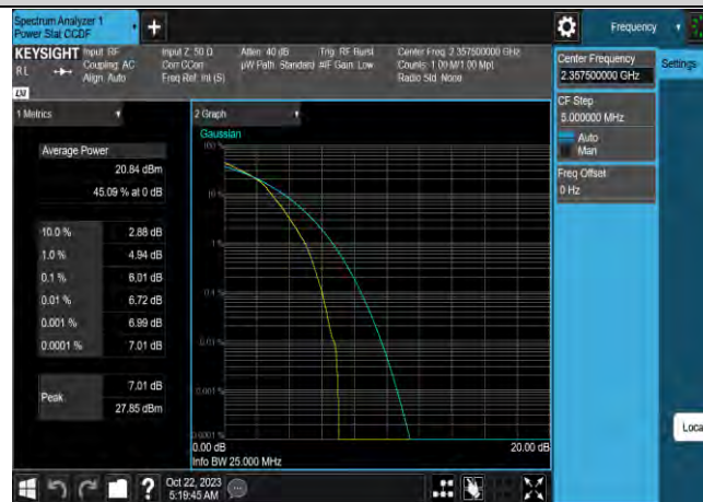
Band40-5MHz-64QAM-39225-25RB#0
