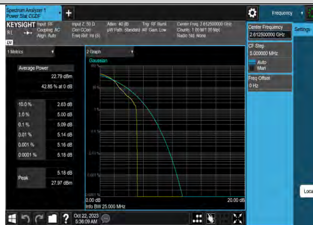
Band38-15MHz-64QAM-38175-75RB#0
