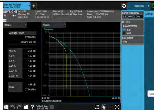
Band42-20MHz-16QAM-42590-100RB#0
