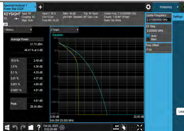
Band40-5MHz-QPSK-38775-25RB#0
