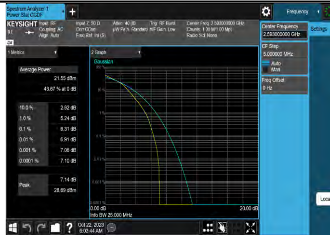
Band41-15MHz-64QAM-41515-1RB#0
