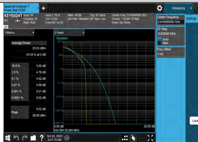
Band38-20MHz-16QAM-38150-100RB#0
