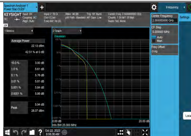
Band41-20MHz-64QAM-40620-100RB#0
