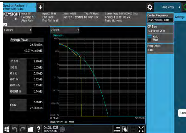
Band41-5MHz-64QAM-41565-25RB#0
