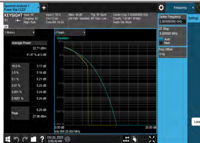
Band41-5MHz-16QAM-40620-25RB#0
