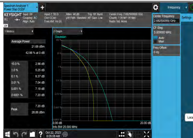
Band41-15MHz-16QAM-39725-1RB#0
