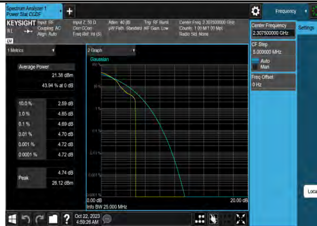
Band40-5MHz-64QAM-38725-25RB#0
