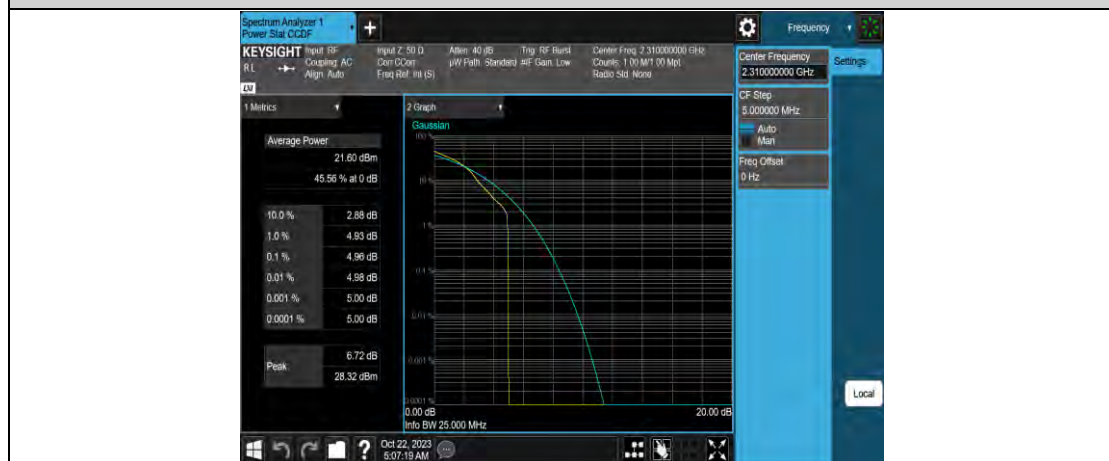
Band40-10MHz-64QAM-38750-50RB#0
