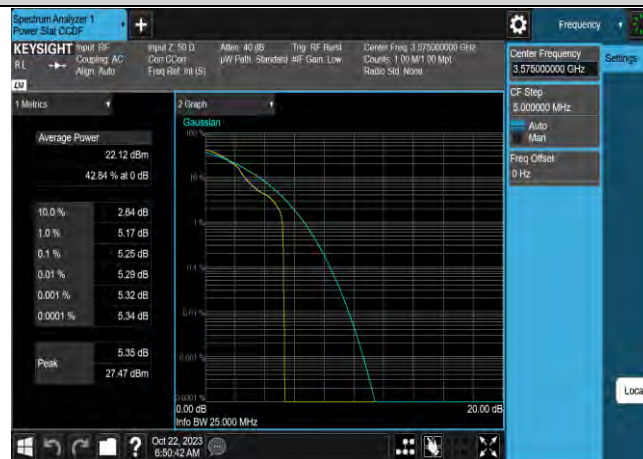
Band42-5MHz-64QAM-43340-25RB#0
