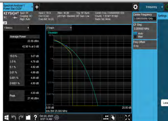
Band42-10MHz-16QAM-43540-50RB#0
