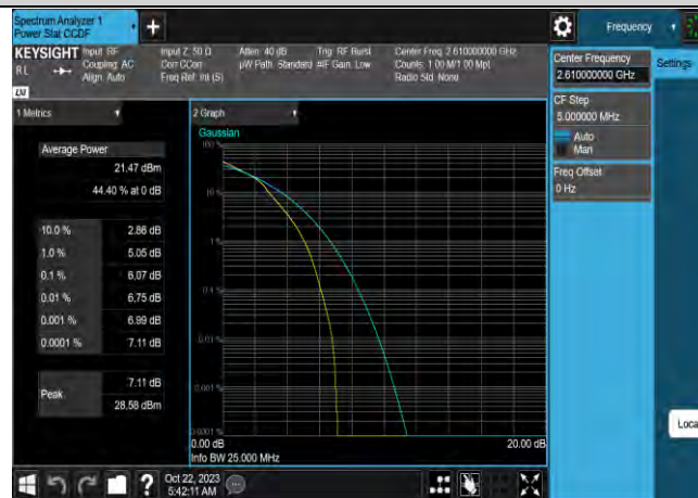
Band38-20MHz-16QAM-37850-1RB#0
