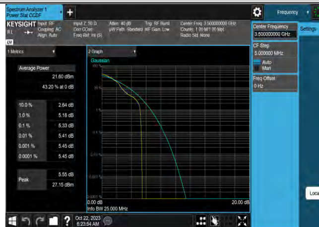
Band42-5MHz-64QAM-42590-25RB#0
