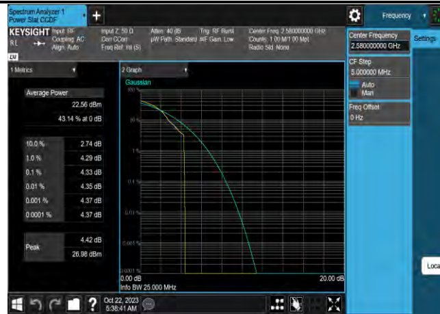
Band38-20MHz-64QAM-37850-100RB#0
