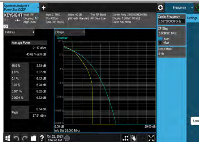
Band42-5MHz-16QAM-43115-1RB#0
