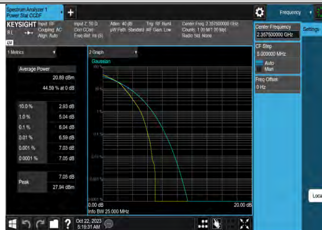
Band40-5MHz-16QAM-39225-25RB#0
