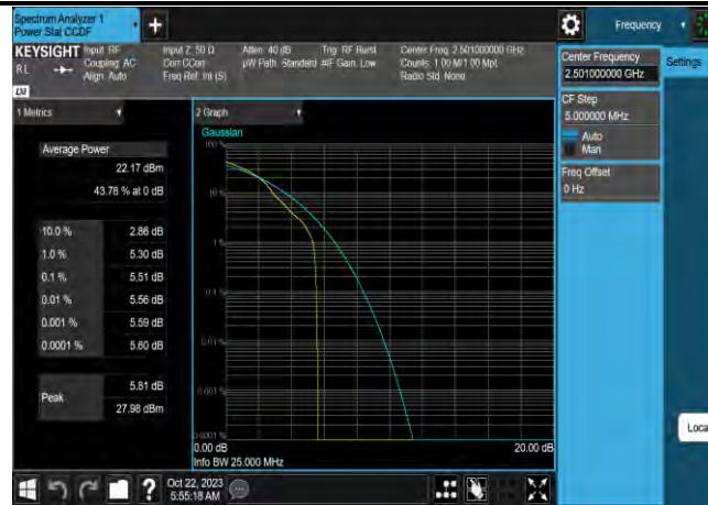
Band41-10MHz-64QAM-39700-50RB#0
