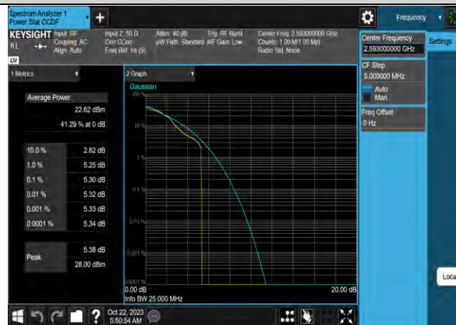
Band41-5MHz-64QAM-40620-25RB#0
