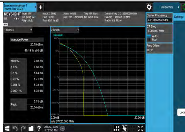
Band40-5MHz-64QAM-38775-25RB#0
