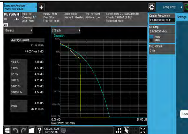
Band40-5MHz-64QAM-38750-25RB#0
