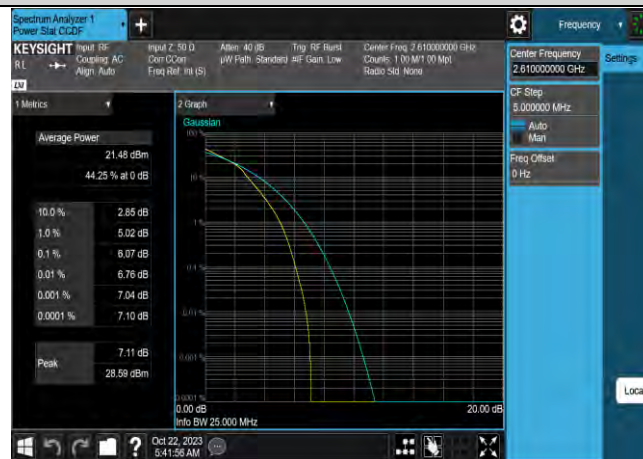
Band38-20MHz-16QAM-38150-100RB#0
