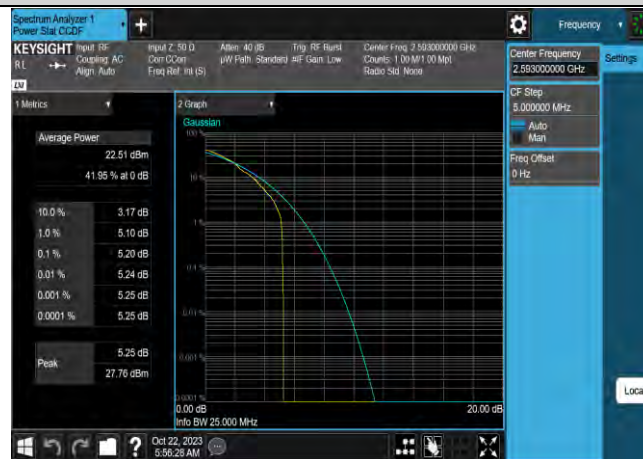
Band41-10MHz-16QAM-40620-50RB#0
