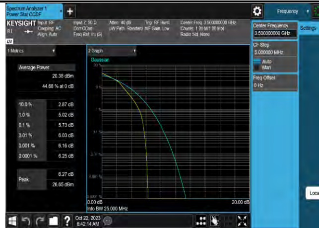
Band42-20MHz-64QAM-43990-1RB#0
