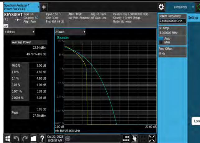
Band41-20MHz-16QAM-39750-100RB#0
