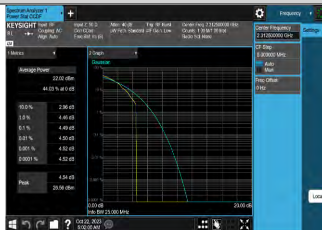
Band40-5MHz-16QAM-38775-25RB#0
