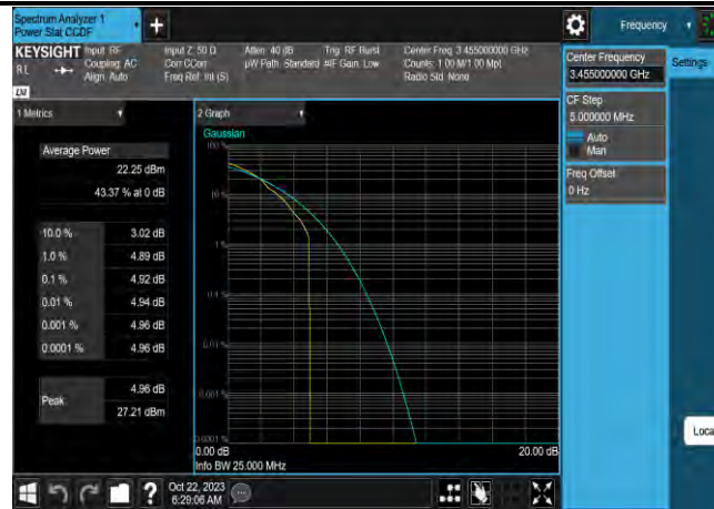
Band42-10MHz-16QAM-42140-50RB#0
