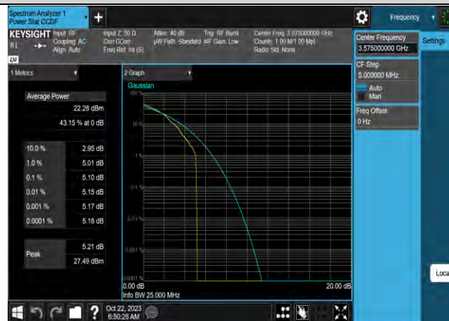
Band42-5MHz-16QAM-43340-25RB#0
