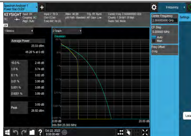
Band41-20MHz-QPSK-40620-100RB#0
