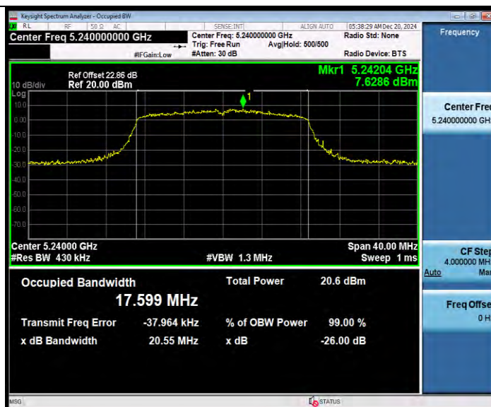
11N20MIMO Ant8 5240
