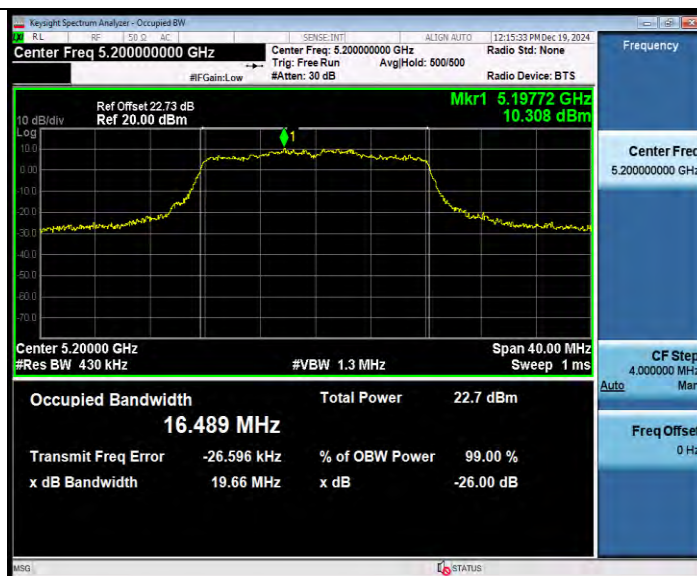
11A-CDD Ant8 5200
