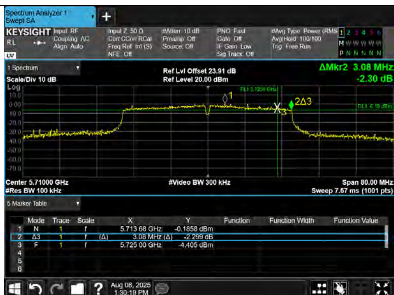
11N40MIMO-Ant8-5710-UNII-3-PASS
