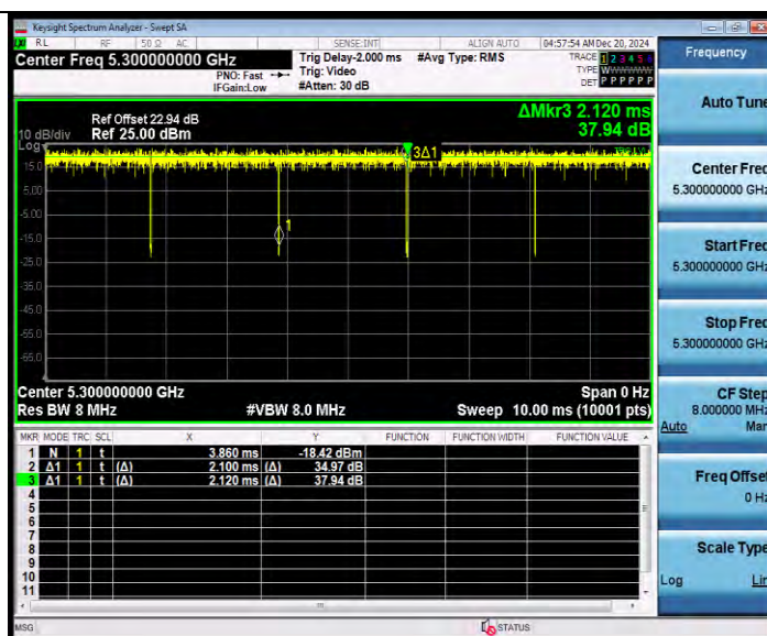
11A-CDD Ant8 5300
