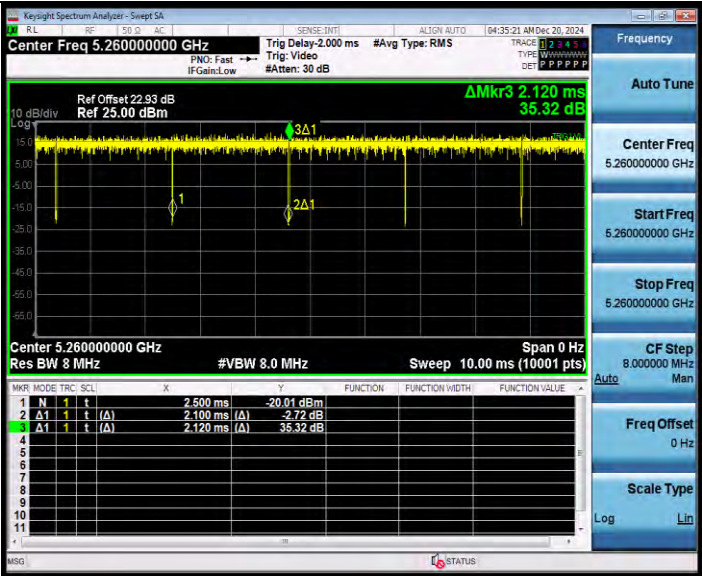
11A-CDD Ant8 5260
