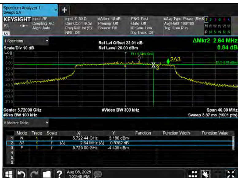
11N20MIMO-Ant8-5720-UNII-3-PASS
