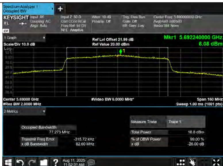
11AX80MIMO Ant8 5690
