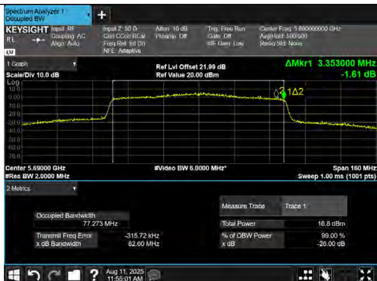
11AX80MIMO Ant8 5690 UNII-3
