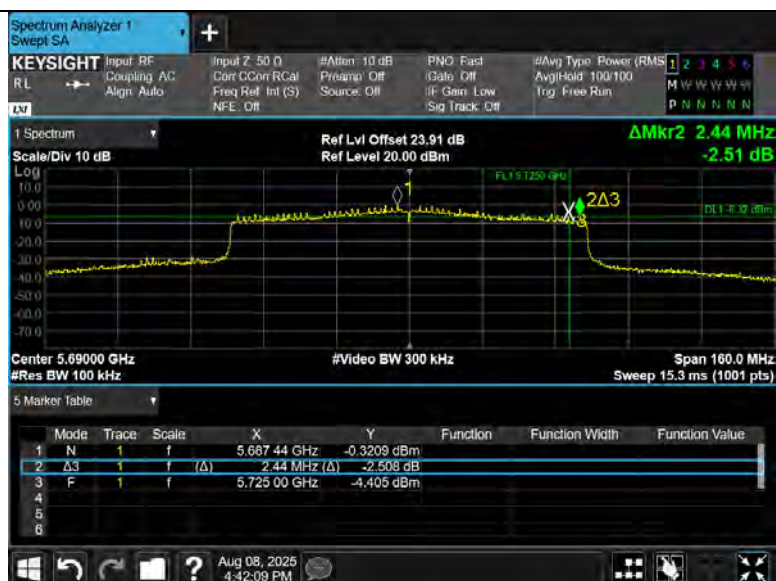
11AX80MIMO-Ant8-5690-UNII-3-PASS
