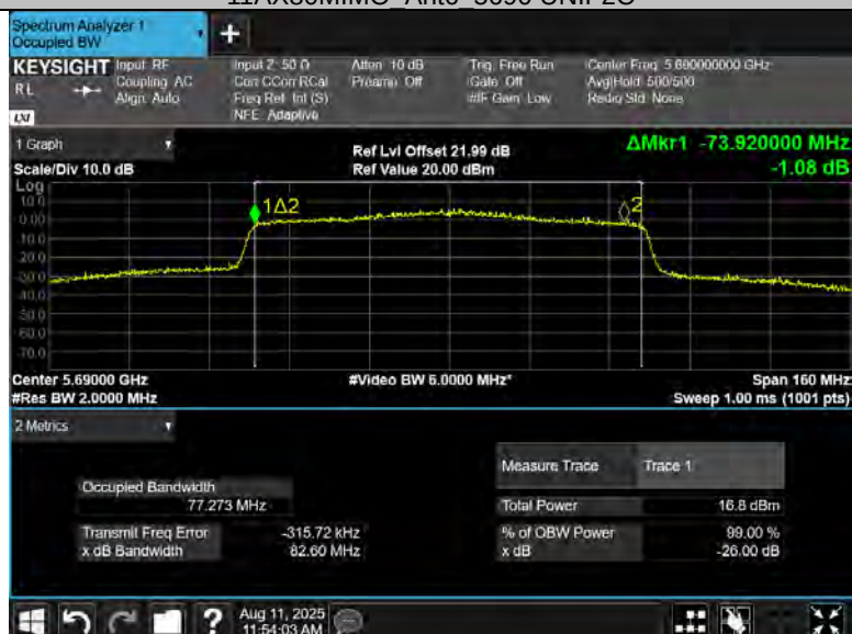
11AX80MIMO Ant8 5690 UNII-2C
