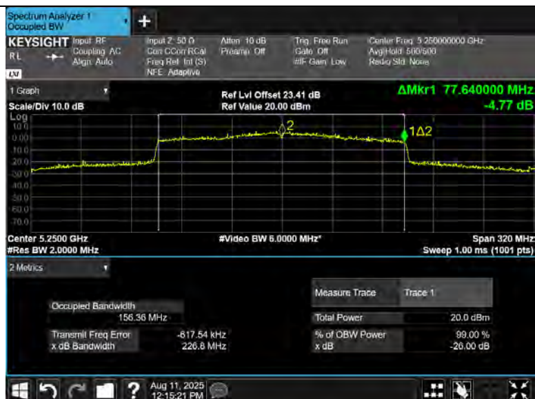
11AX160MIMO Ant8 5250 UNII-2A
