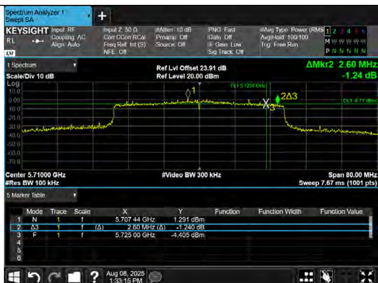
11AX40MIMO-Ant8-5710-UNII-3-PASS
