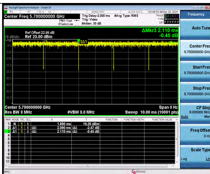
11A-CDD Ant8 5700
