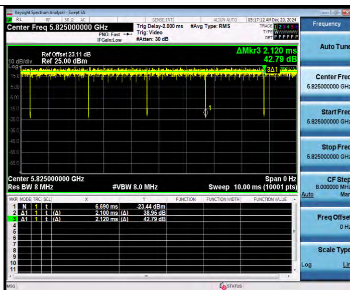
11A-CDD Ant8 5825
