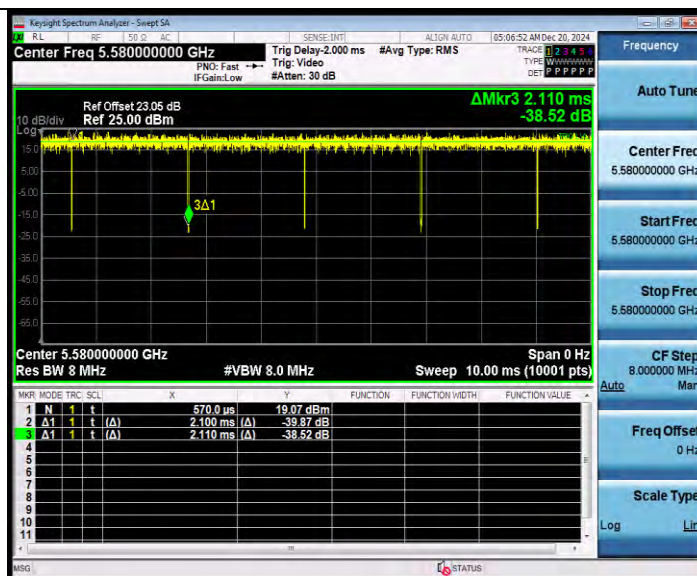
11A-CDD Ant8 5580
