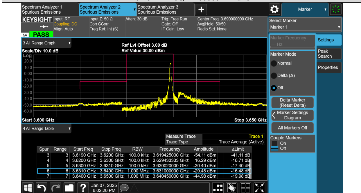
Band48-10MHz-16QAM-55990-50RB#0
