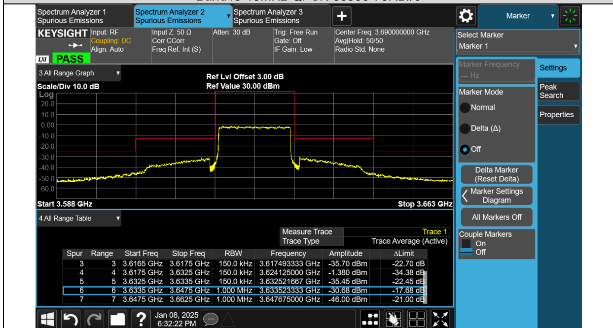
Band48-15MHz-QPSK-56665-1RB#0
