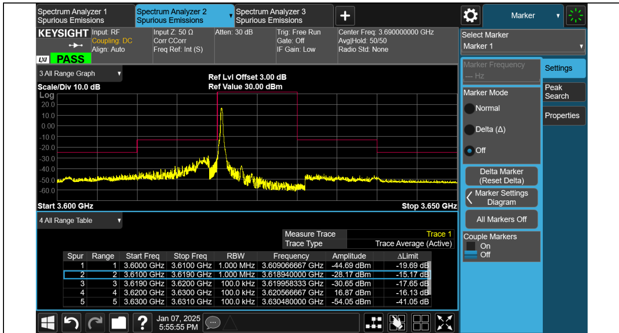
Band48-10MHz-16QAM-55990-1RB#49
