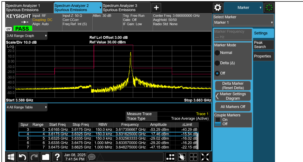
Band48-15MHz-QPSK-55990-75RB#0
