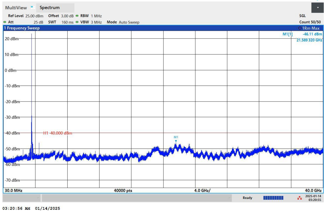
Band48-5MHz-QPSK-55990-1RB#0-Range:30~40000MHz
