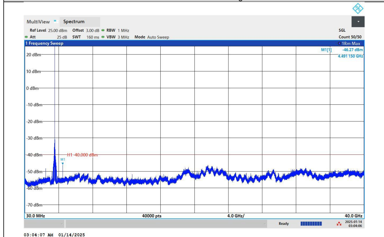
Band48-10MHz-QPSK-55990-1RB#0-Range:30~40000MHz
