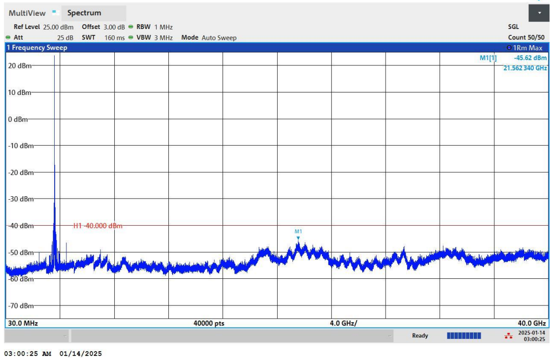
Band48-10MHz-QPSK-56690-1RB#0-Range:30~40000MHz
