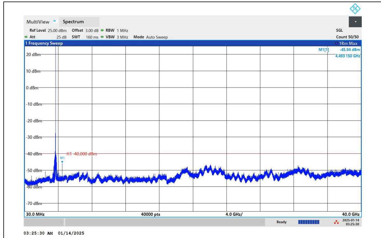
Band48-10MHz-QPSK-55290-1RB#0-Range:30~40000MHz
