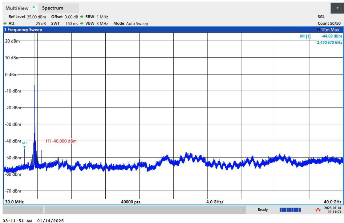
Band48-15MHz-QPSK-55315-1RB#0-Range:30~40000MHz
