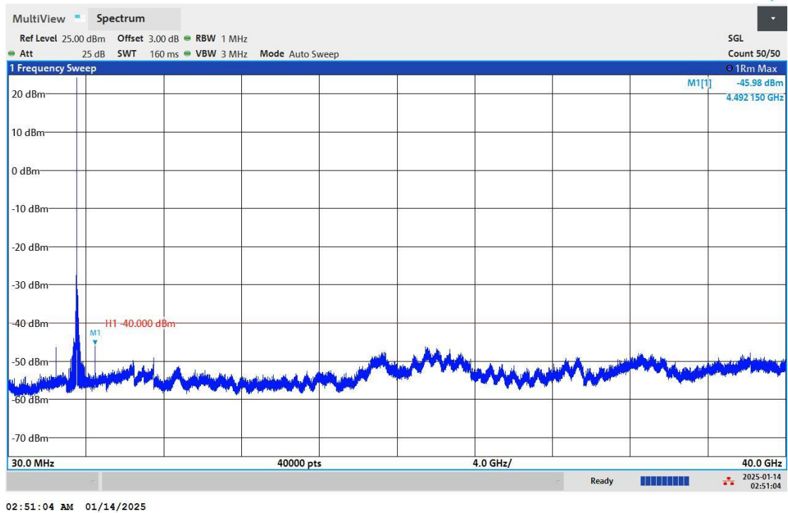
Band48-15MHz-QPSK-55990-1RB#0-Range:30~40000MHz
