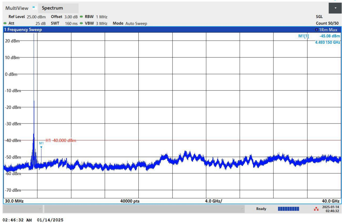
Band48-15MHz-QPSK-56665-1RB#0-Range:30~40000MHz
