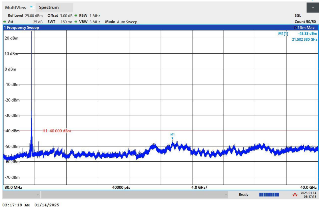
Band48-5MHz-QPSK-56715-1RB#0-Range:30~40000MHz
