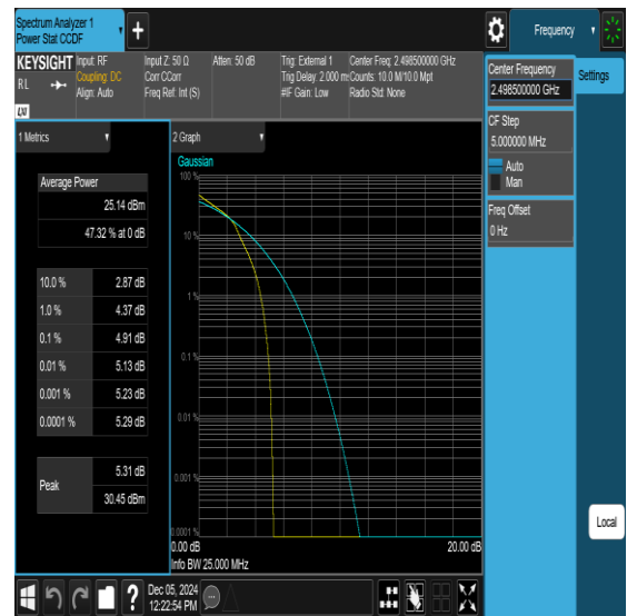
Band41-5MHz-16QAM-39675-25RB#0-PASS
