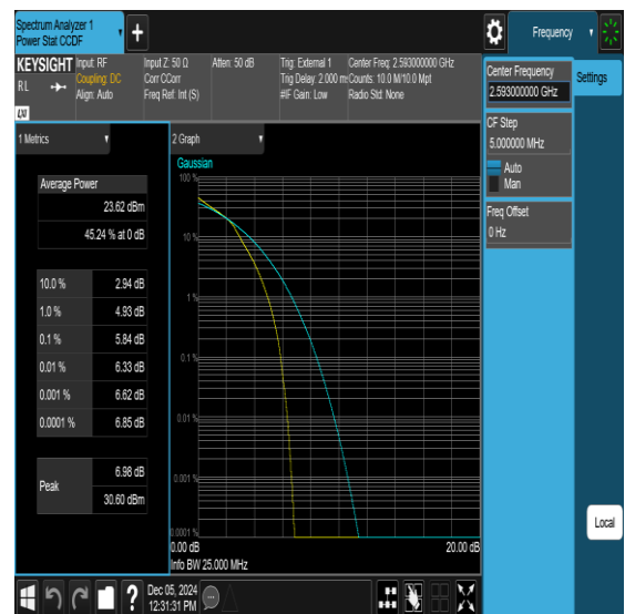
Band41-15MHz-16QAM-40620-75RB#0-PASS
