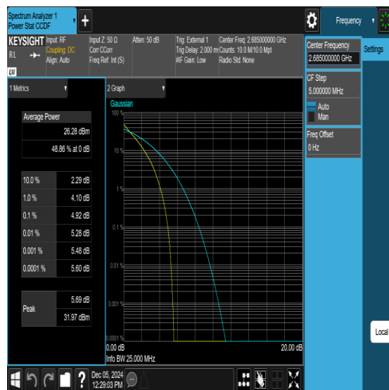
Band41-10MHz-QPSK-41540-50RB#0-PASS
