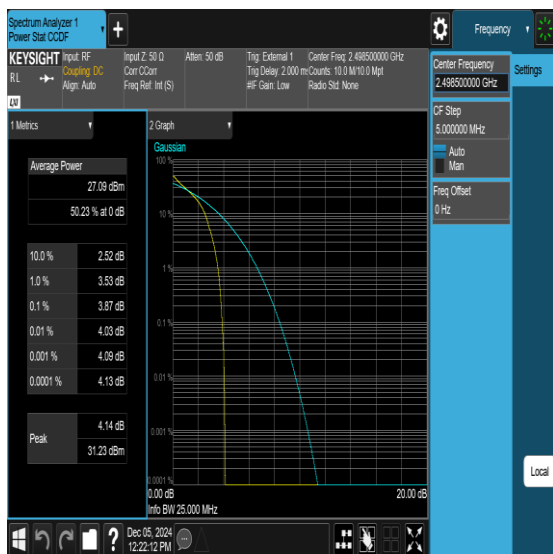
Band41-5MHz-QPSK-40620-1RB#0-PASS
