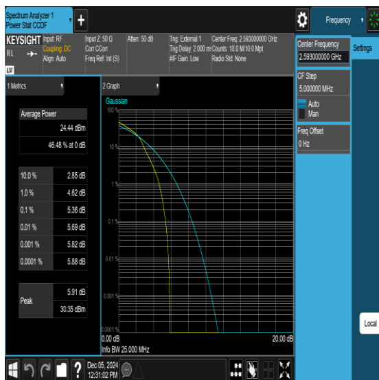
Band41-15MHz-16QAM-40620-1RB#0-PASS
