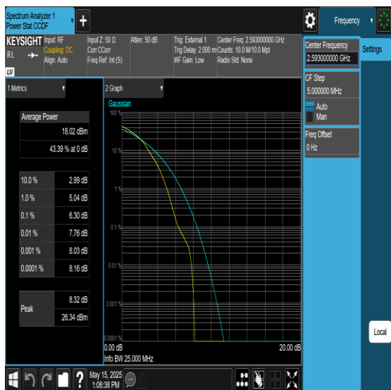
Band41-10MHz-256QAM-40620-1RB#0-PASS
