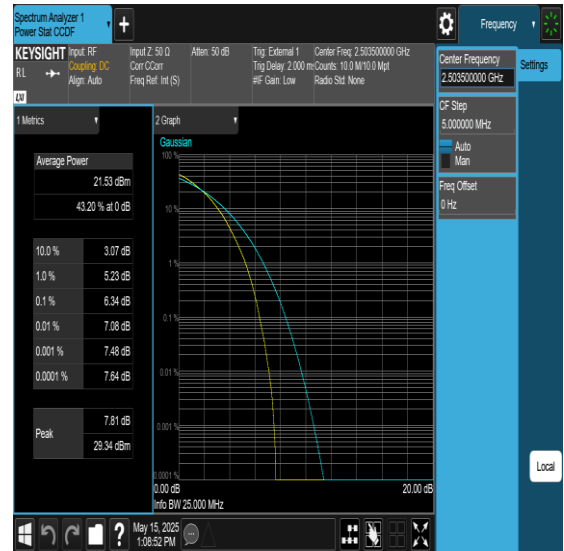
Band41-15MHz-64QAM-40620-75RB#0-PASS
