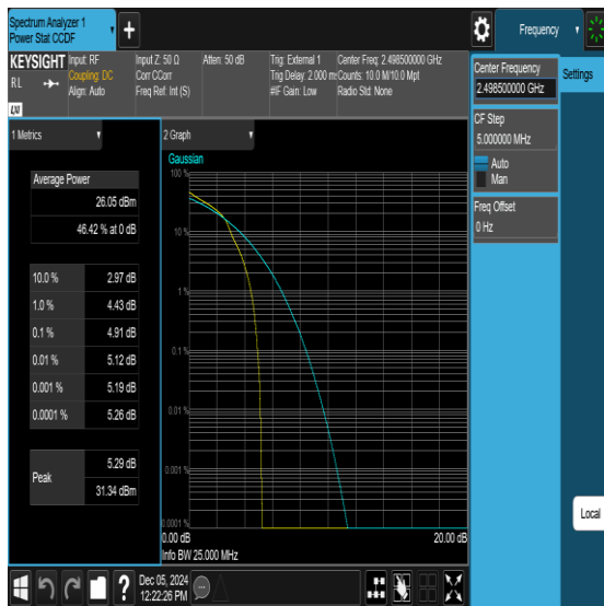
Band41-5MHz-16QAM-39675-1RB#0-PASS
