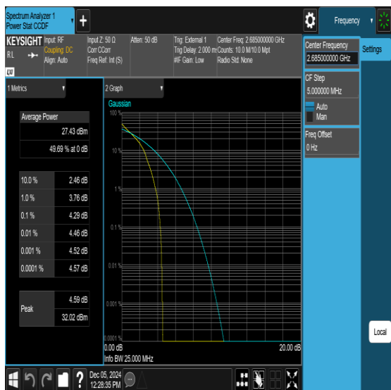
Band41-10MHz-QPSK-41540-1RB#0-PASS
