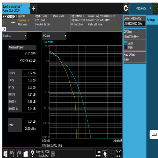
Band41-5MHz-64QAM-40620-1RB#0-PASS
