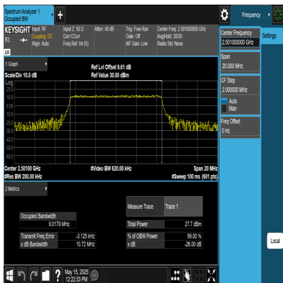
Band41-10MHz-256QAM-39700-50RB#0-PASS
