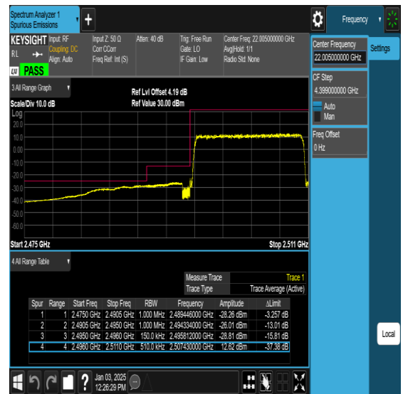
Band41-15MHz-QPSK-39725-75RB#0-PASS
