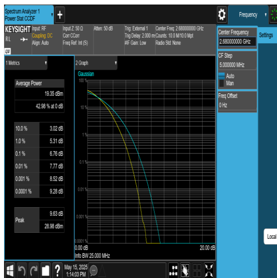
Band41-20MHz-256QAM-41490-100RB#0-PASS
