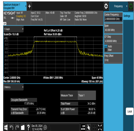
Band41-20MHz-16QAM-41490-100RB#0-PASS
