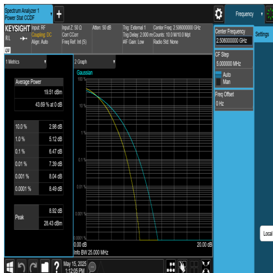
Band41-20MHz-256QAM-40620-100RB#0-PASS
