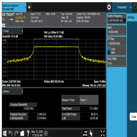
Band41-5MHz-256QAM-41565-25RB#0-PASS
