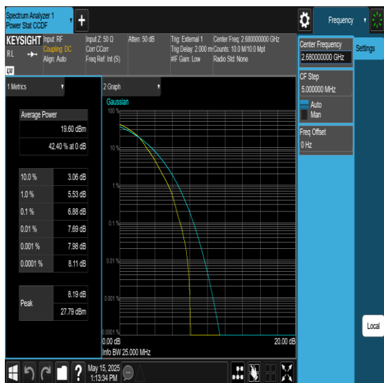
Band41-20MHz-256QAM-41490-1RB#0-PASS
