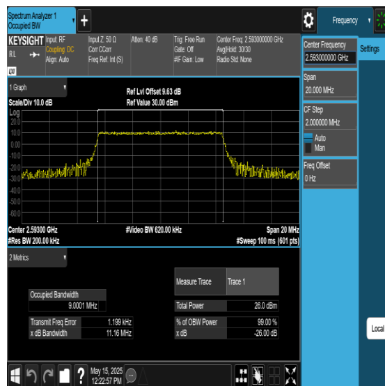
Band41-10MHz-256QAM-40620-50RB#0-PASS
