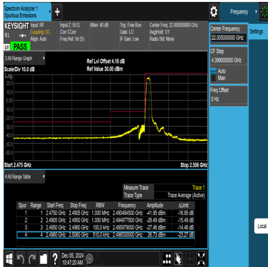
Band41-10MHz-QPSK-41540-1RB#49-PASS
