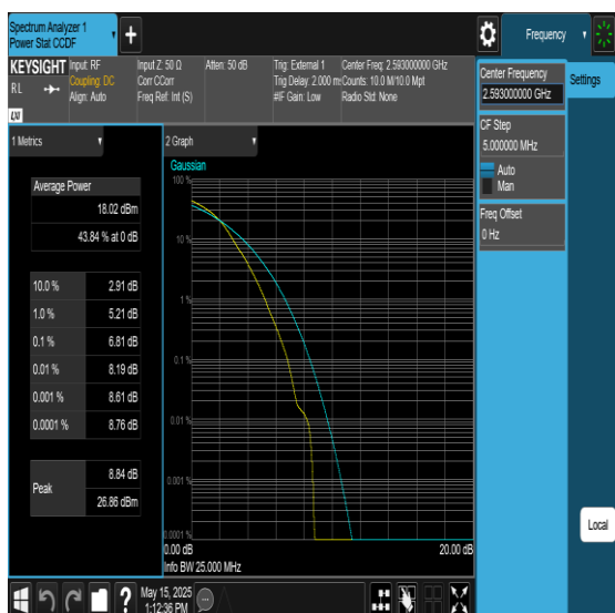
Band41-20MHz-256QAM-41490-1RB#0-PASS
