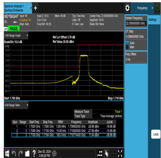
Band66-1.4MHz-QPSK-132665-6RB#0-PASS
