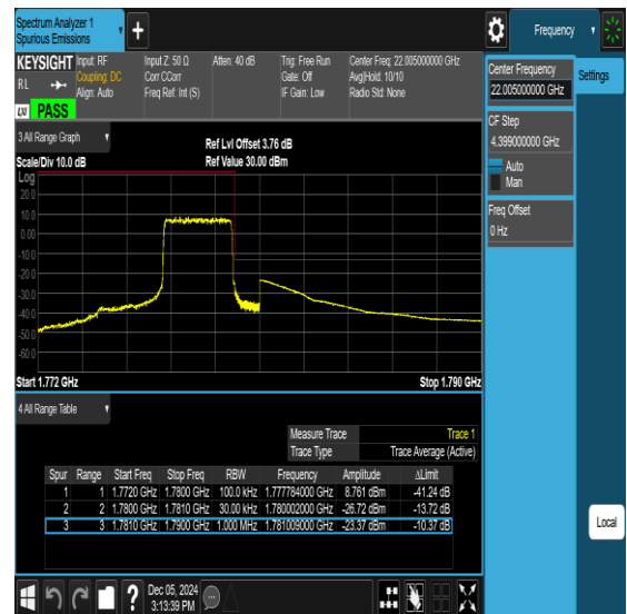
Band66-3MHz-QPSK-132657-15RB#0-PASS
