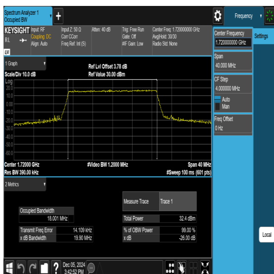
Band66-20MHz-QPSK-132072-100RB#0-PASS
