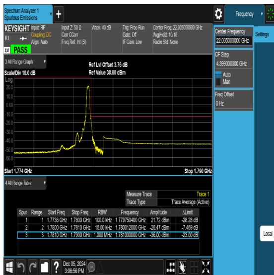
Band66-1.4MHz-64QAM-131979-1RB#0-PASS
