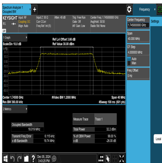
Band66-20MHz-16QAM-132322-100RB#0-PASS
