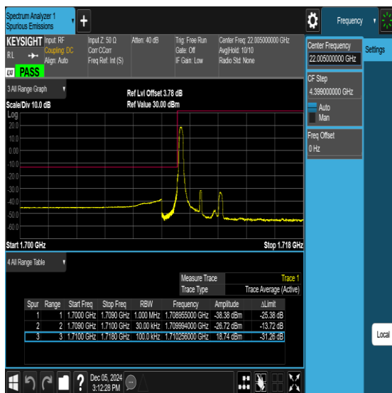
Band66-3MHz-16QAM-131987-1RB#0-PASS
