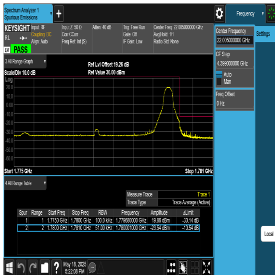
Band66-5MHz-64QAM-132647-1RB#24-PASS
