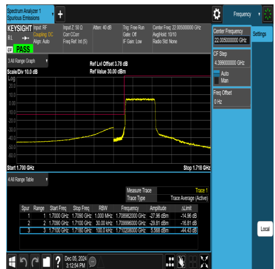
Band66-3MHz-16QAM-131987-15RB#0-PASS
