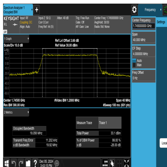
Band66-20MHz-QPSK-132322-100RB#0-PASS
