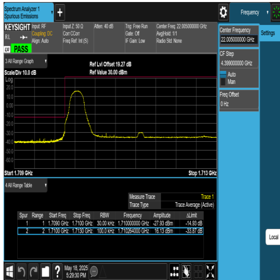
Band66-3MHz-256QAM-132657-1RB#14-PASS
