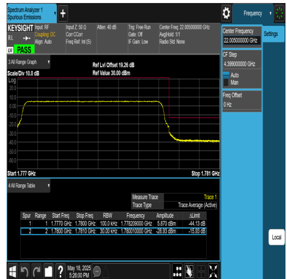
Band66-3MHz-16QAM-131987-15RB#0-PASS
