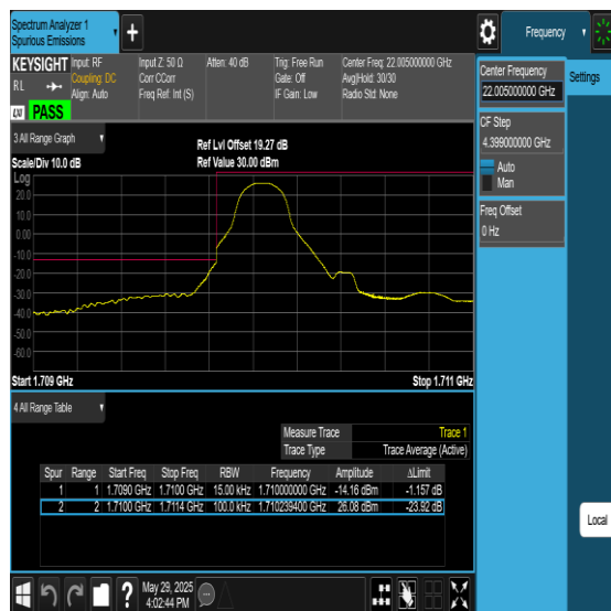
Band66-1.4MHz-256QAM-131979-1RB#0-PASS
