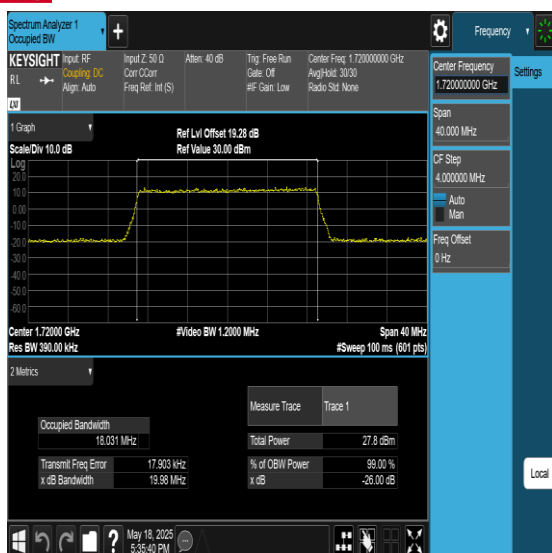
Band66-20MHz-256QAM-132572-100RB#0-PASS
