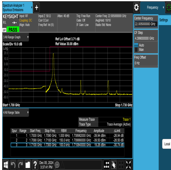
Band66-15MHz-QPSK-132597-1RB#74-PASS
