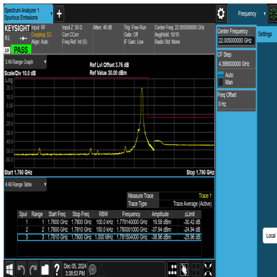
Band66-15MHz-16QAM-132597-1RB#74-PASS
