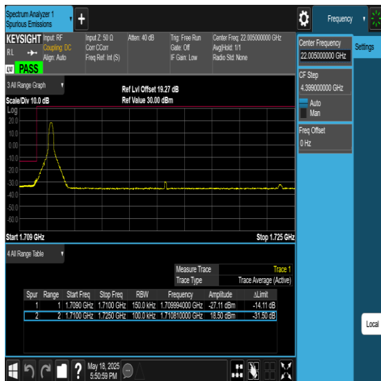
Band66-15MHz-64QAM-132047-1RB#0-PASS
