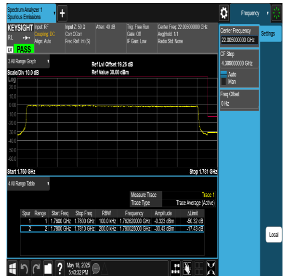
Band66-20MHz-256QAM-132072-100RB#0-PASS
