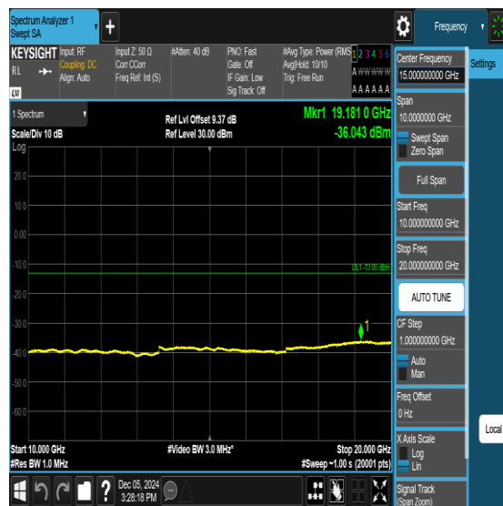
Band66-10MHz-QPSK-132022-1RB#0-10000~20000-PASS
