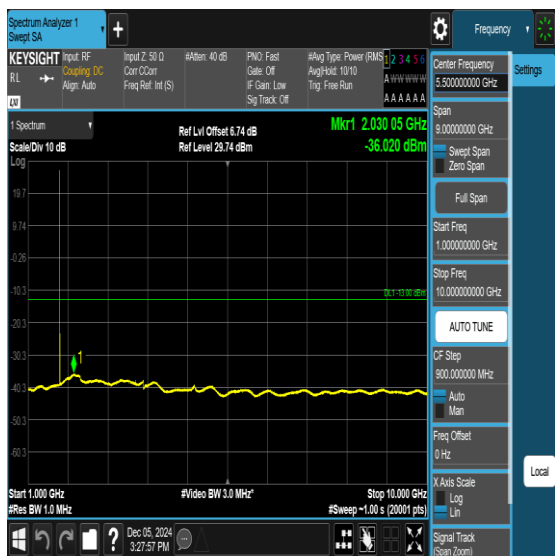
Band66-10MHz-QPSK-132022-1RB#0-1000~10000-PASS
