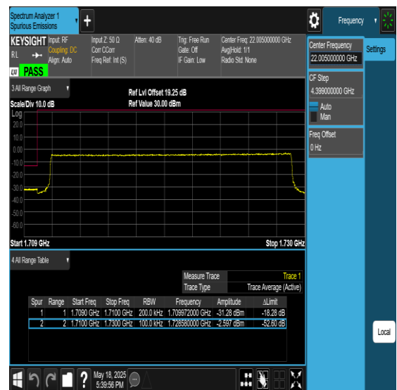
Band66-20MHz-256QAM-132072-100RB#0-PASS
