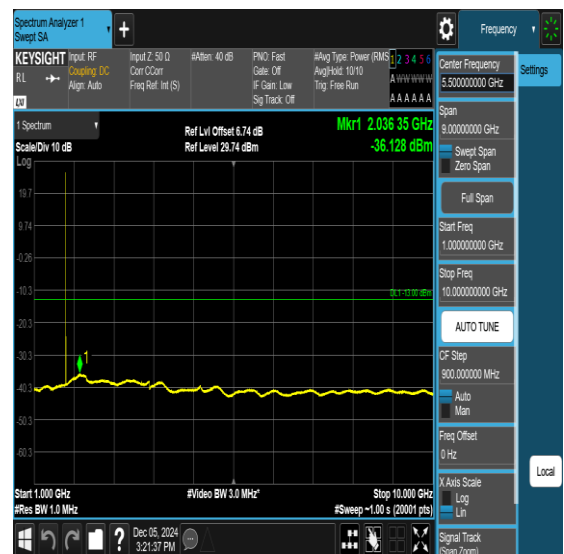
Band66-5MHz-QPSK-131997-1RB#0-1000~10000-PASS
