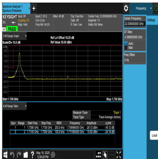
Band66-20MHz-256QAM-132072-1RB#0-PASS
