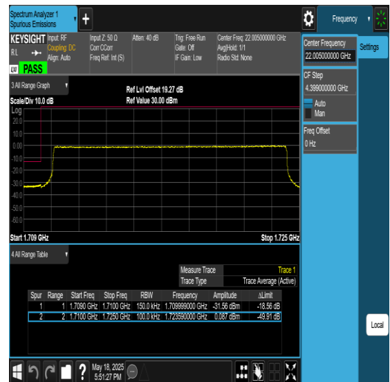
Band66-15MHz-64QAM-132047-75RB#0-PASS
