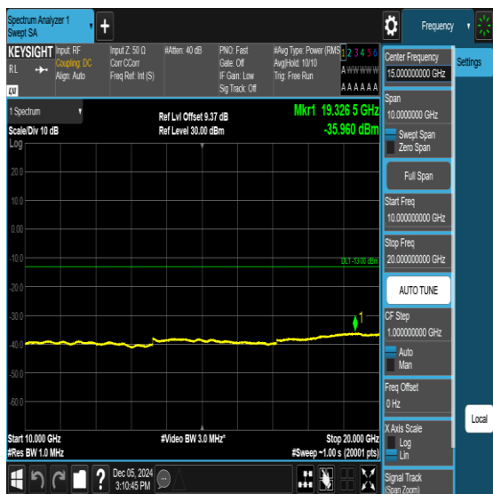
Band66-1.4MHz-QPSK-132665-1RB#0-10000~20000-PASS
