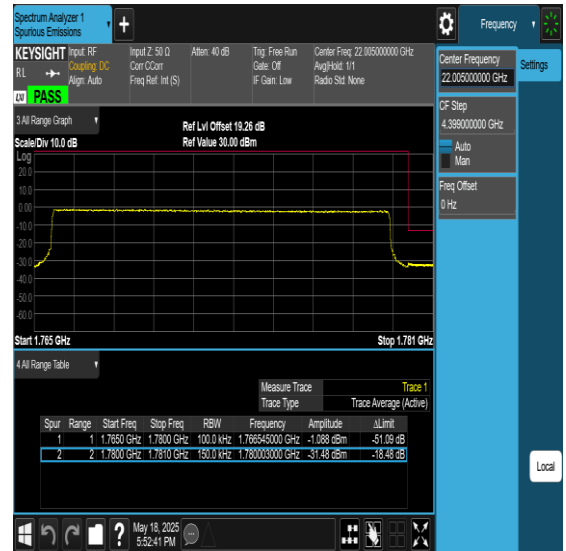
Band66-15MHz-16QAM-132047-75RB#0-PASS
