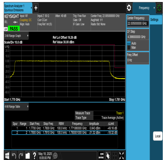
Band66-10MHz-256QAM-132622-50RB#0-PASS
