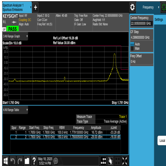
Band66-15MHz-16QAM-132047-1RB#0-PASS
