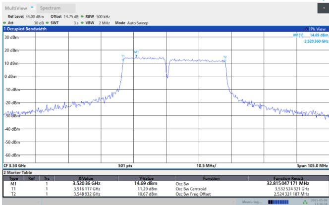
42-42-15MHz-20MHz-16QAM-16QAM-42493-42664-75RB#0-100RB#0
