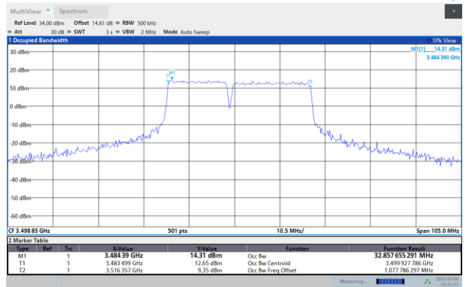
42-42-15MHz-20MHz-16QAM-16QAM-42168-42339-75RB#0-100RB#0
