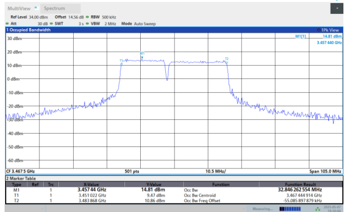
42-42-15MHz-20MHz-16QAM-16QAM-42819-42990-75RB#0-100RB#0
