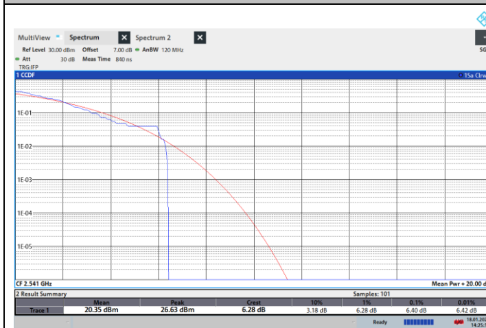
NTN-N41-PC2-30-90-L-CP-QPSK-Outer_Full-PASS
