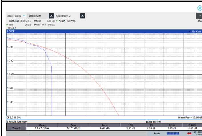
NTNV-N41-PC2-30-30-L-CP-256QPSK-Outer_Full-PASS
