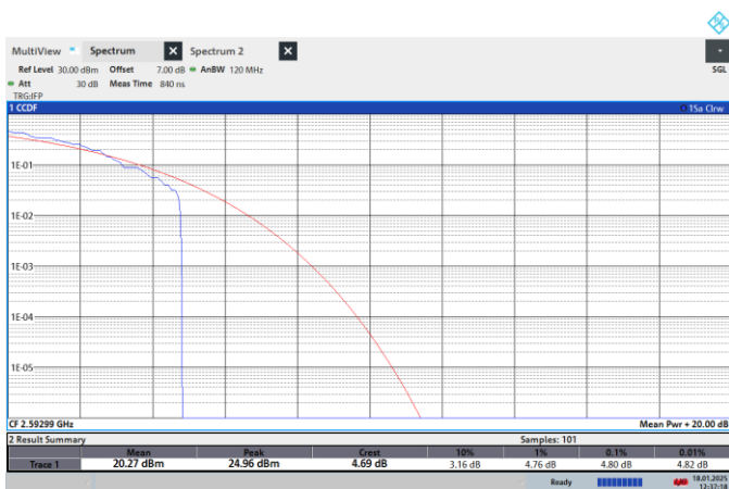
NTNV-N41-PC2-30-40-M-CP-QPSK-Outer_Full-PASS
