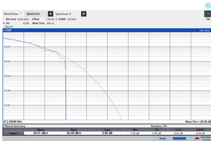
NTNV-N41-PC2-30-30-M-CP-QPSK-Outer_Full-PASS
