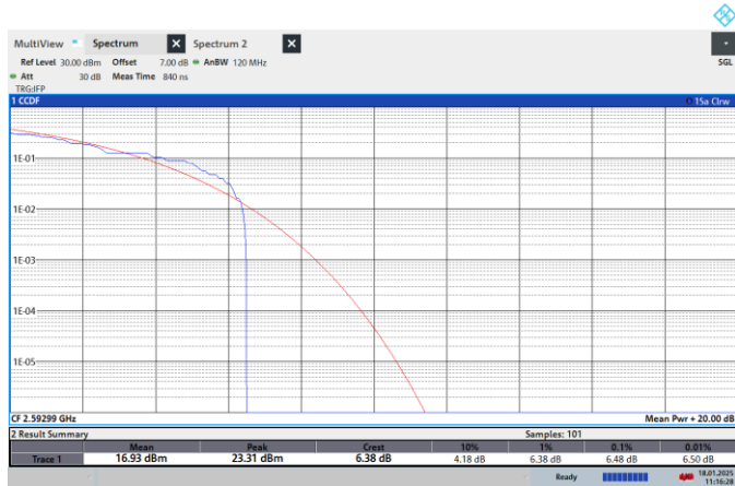
NTNV-N41-PC2-30-20-M-CP-256QPSK-Outer_Full-PASS
