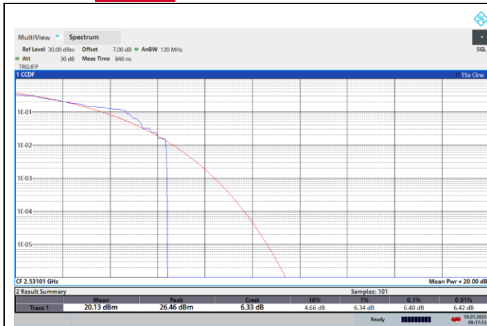
NTNV-N41-PC2-30-70-L-CP-16QPSK-Outer_Full-PASS
