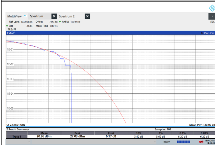
NTNV-N41-PC2-30-100-L-CP-QPSK-Outer_Full-PASS
