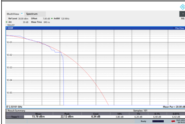
NTNV-N41-PC2-30-70-L-CP-256QPSK-Outer_Full-PASS
