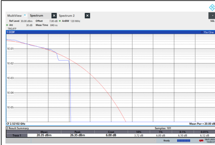
NTNV-N41-PC2-30-50-L-CP-QPSK-Outer_Full-PASS
