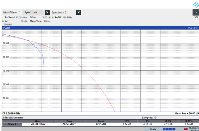
NTN-N41-PC2-30-20-M-CP-64QPSK-Outer_Full-PASS
