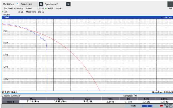
NTN-N41-PC2-30-20-M-CP-QPSK-Outer_Full-PASS
