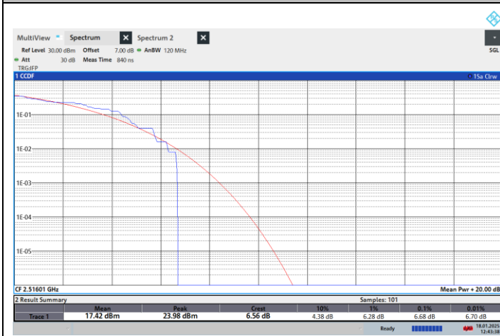
NTNV-N41-PC2-30-40-L-CP-256QPSK-Outer_Full-PASS
