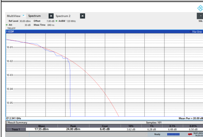
NTNV-N41-PC2-30-90-L-CP-256QPSK-Outer_Full-PASS
