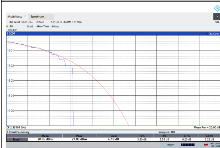
NTNV-N41-PC2-30-70-L-CP-QPSK-Outer_Full-PASS
