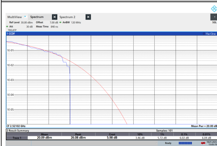
NTNV-N41-PC2-30-50-L-CP-16QPSK-Outer_Full-PASS
