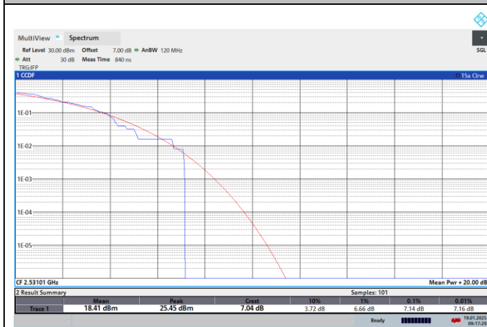
NTNV-N41-PC2-30-70-L-CP-64QPSK-Outer_Full-PASS
