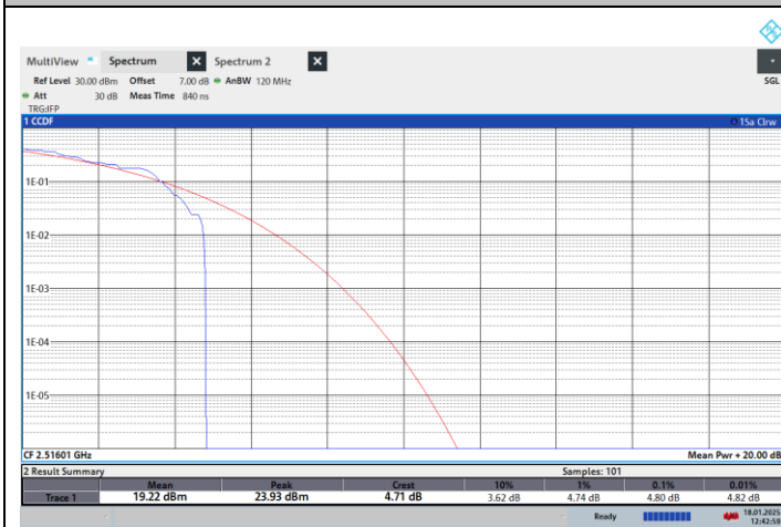
NTNV-N41-PC2-30-40-L-CP-64QPSK-Outer_Full-PASS
