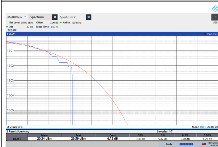
NTN-N41-PC2-30-60-L-CP-QPSK-Outer_Full-PASS
