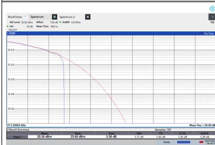
NTNV-N41-PC2-30-80-L-CP-16QPSK-Outer_Full-PASS
