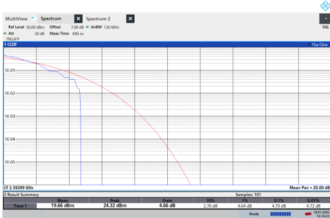
NTNV-N41-PC2-30-30-M-CP-64QPSK-Outer_Full-PASS
