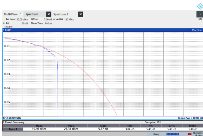
NTNV-N41-PC2-30-30-M-CP-16QPSK-Outer_Full-PASS
