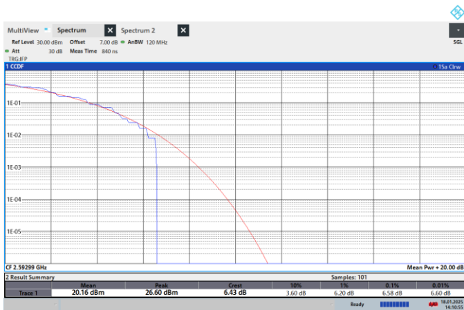
NTN-N41-PC2-30-80-M-CP-16QPSK-Outer_Full-PASS
