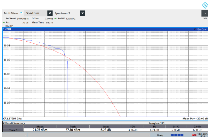
NTNV-N41-PC2-30-20-H-CP-QPSK-Outer_Full-PASS
