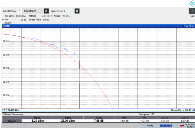
NTNV-N41-PC2-30-50-H-CP-256QPSK-Outer_Full-PASS
