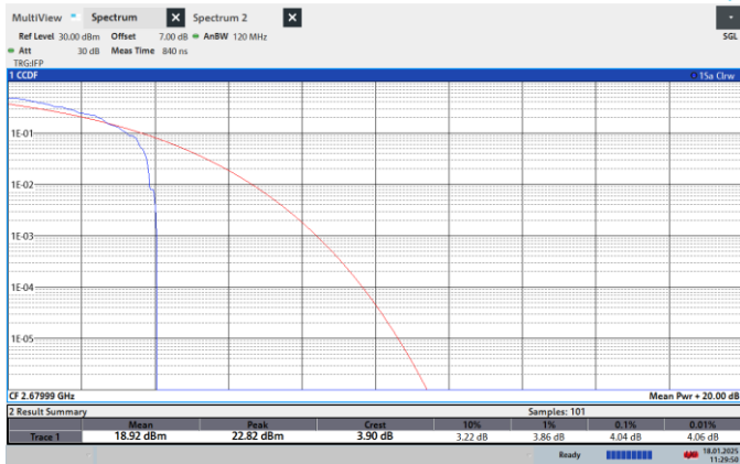
NTNV-N41-PC2-30-20-H-CP-256QPSK-Outter_Full-PASS
