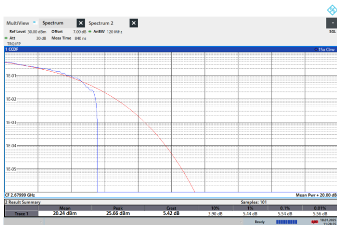
NTNV-N41-PC2-30-20-H-CP-16QPSK-Outer_Full-PASS
