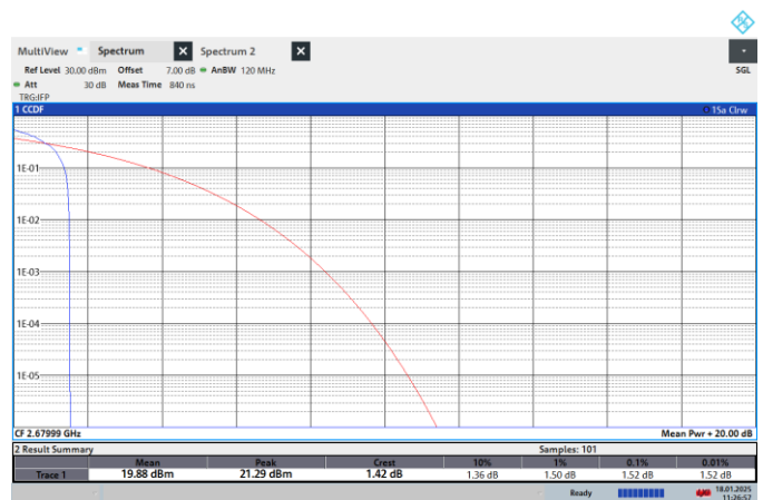
NTNV-N41-PC2-30-20-H-CP-16QPSK-Edge_1RB_Left-PASS
