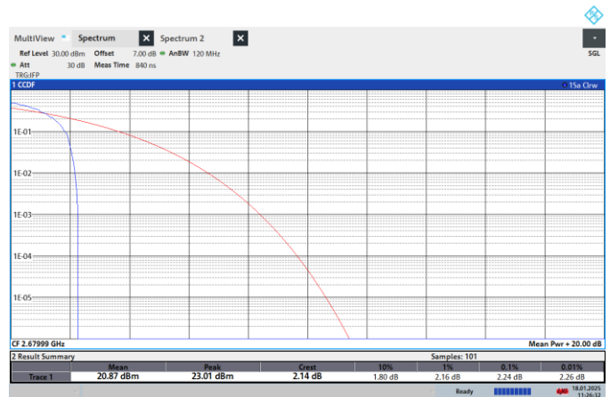
NTNV-N41-PC2-30-20-H-CP-QPSK-Edge_1RB_Left-PASS
