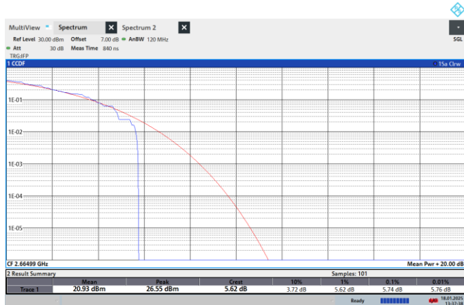
NTNV-N41-PC2-30-50-H-CP-QPSK-Outer_Full-PASS
