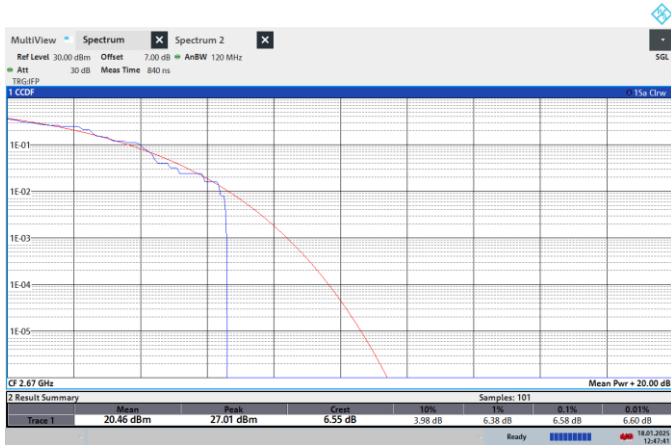
NTNV-N41-PC2-30-40-H-CP-16QPSK-Outer_Full-PASS
