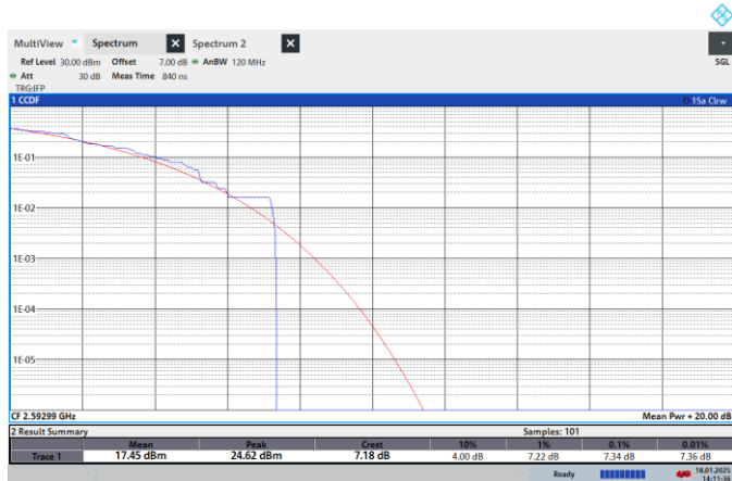
NTNV-N41-PC2-30-80-M-CP-256QPSK-Outer_Full-PASS
