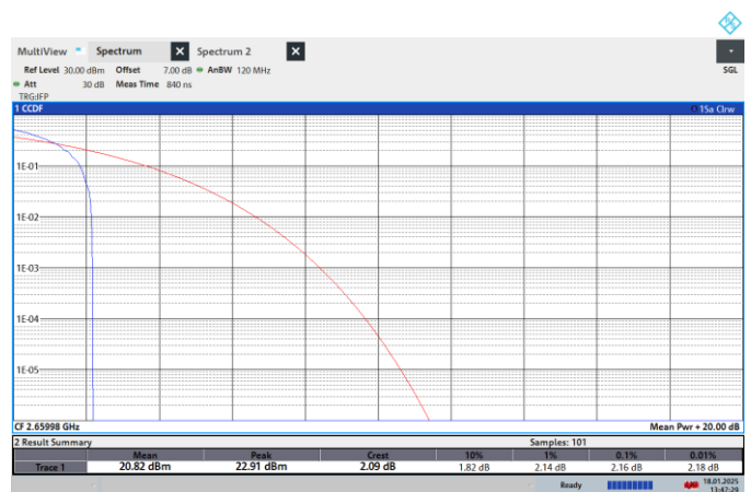
NTNV-N41-PC2-30-60-H-CP-16QPSK-Edge_1RB_Left-PASS
