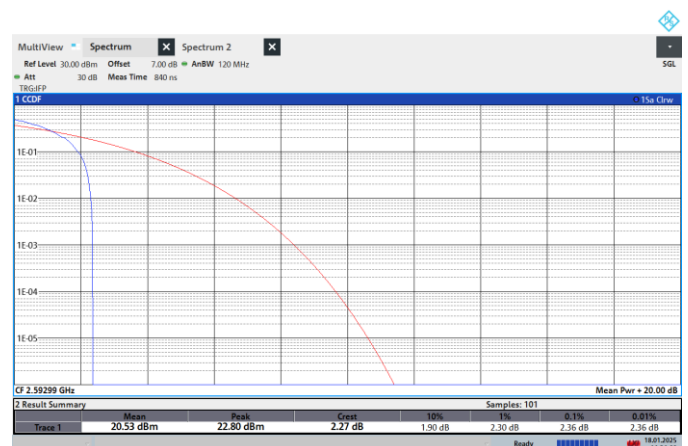
NTNV-N41-PC2-30-100-M-CP-QPSK-Edge_1RB_Left-PASS
