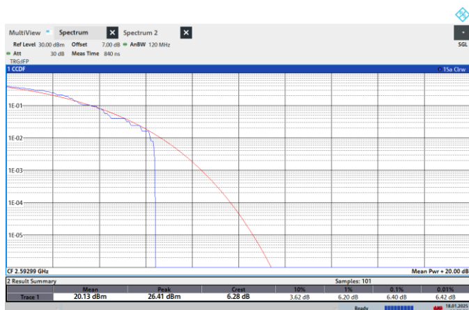
NTNV-N41-PC2-30-100-M-CP-QPSK-Outer_Full-PASS
