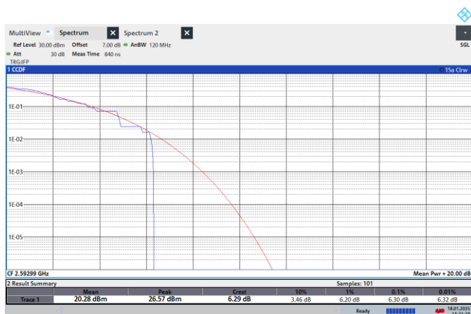
NTNV-N41-PC2-30-90-M-CP-16QPSK-Outer_Full-PASS
