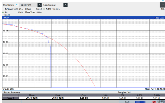
NTNV-N41-PC2-30-40-H-CP-QPSK-Outer_Full-PASS
