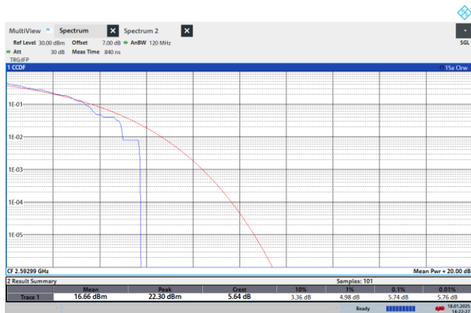
NTNV-N41-PC2-30-90-M-CP-256QPSK-Outer_Full-PASS
