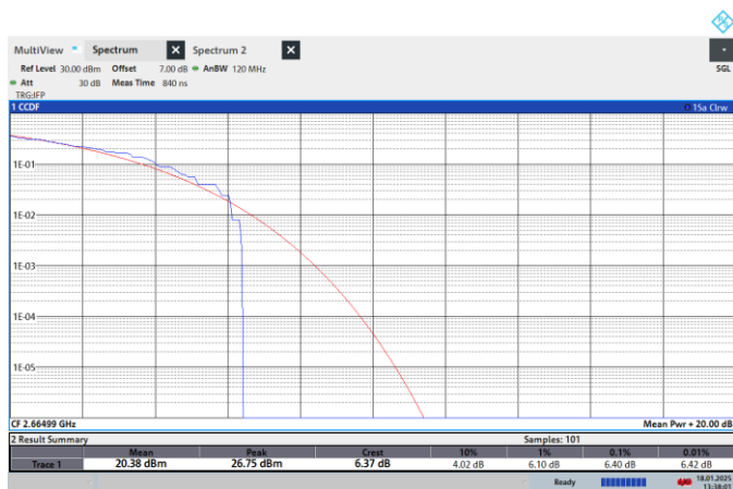
NTNV-N41-PC2-30-50-H-CP-16QPSK-Outer_Full-PASS
