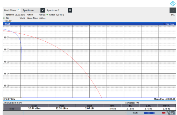
NTNV-N41-PC2-30-40-H-CP-16QPSK-Edge_1RB_Left-PASS
