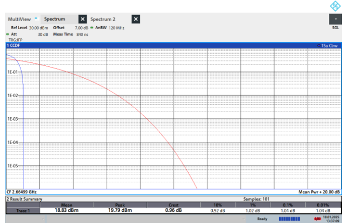
NTNV-N41-PC2-30-50-H-CP-256QPSK-Edge_1RB_Left-PASS
