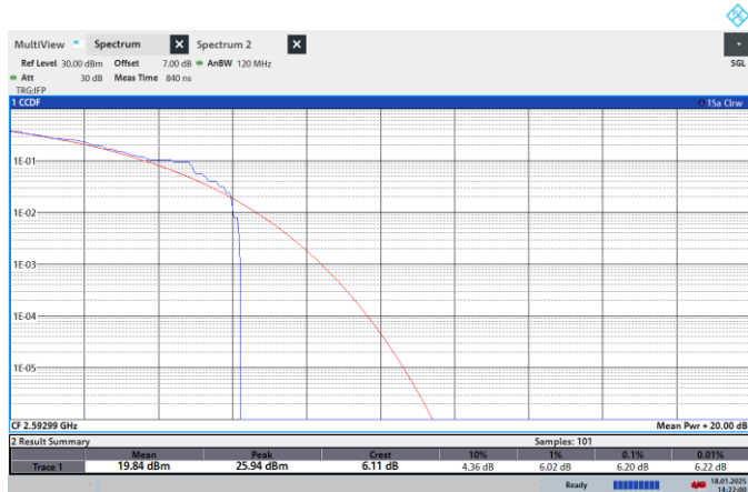
NTNV-N41-PC2-30-90-M-CP-64QPSK-Outer_Full-PASS
