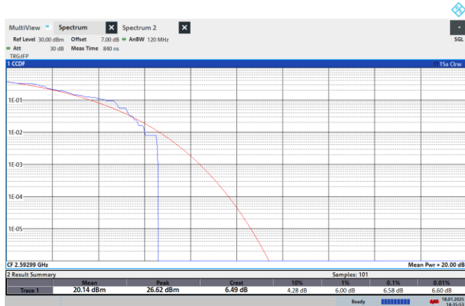
NTNV-N41-PC2-30-100-M-CP-16QPSK-Outer_Full-PASS
