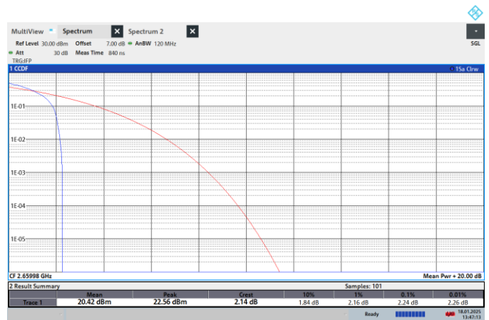
NTNV-N41-PC2-30-60-H-CP-QPSK-Edge_1RB_Left-PASS
