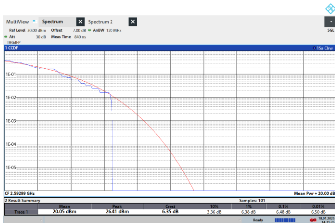
NTNV-N41-PC2-30-90-M-CP-QPSK-Outer_Full-PASS
