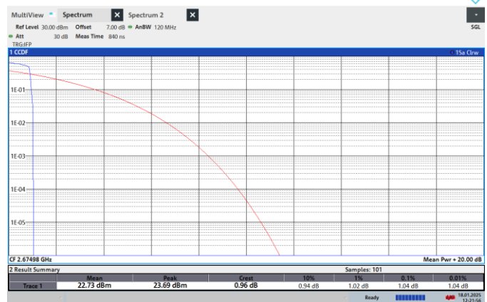
NTNV-N41-PC2-30-30-H-CP-QPSK-Edge_1RB_Left-PASS
