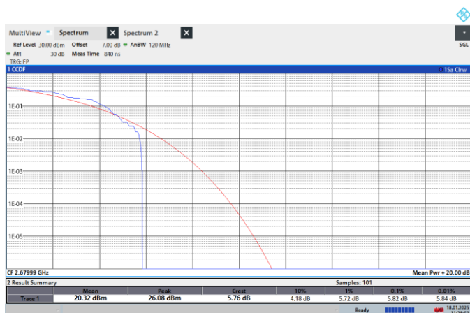
NTNV-N41-PC2-30-20-H-CP-64QPSK-Outer_Full-PASS
