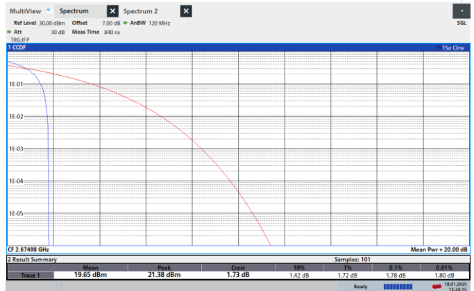
NTNV-N41-PC2-30-30-H-CP-64QPSK-Edge_1RB_Left-PASS
