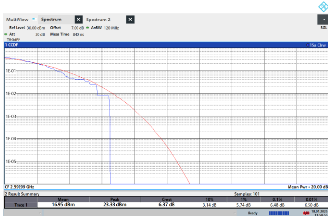
NTNV-N41-PC2-30-50-M-CP-256QPSK-Outer_Full-PASS
