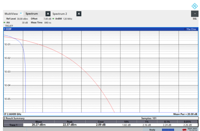
NTNV-N41-PC2-30-50-H-CP-64QPSK-Edge_1RB_Left-PASS
