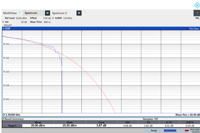
NTNV-N41-PC2-30-70-M-CP-64QPSK-Outer_Full-PASS
