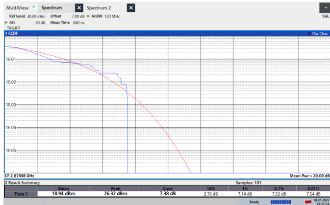
NTNV-N41-PC2-30-30-H-CP-64QPSK-Outer_Full-PASS
