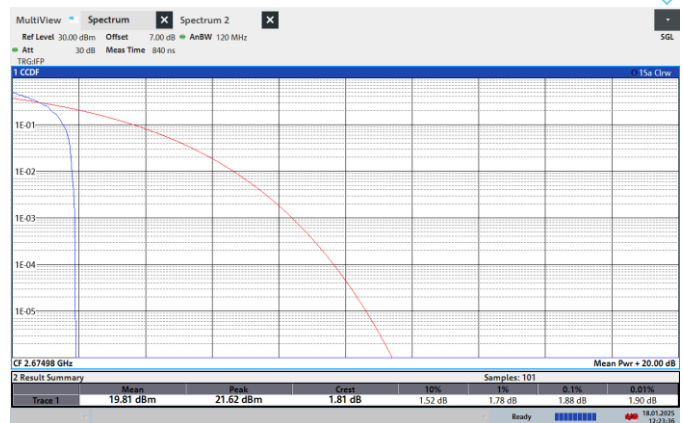
NTNV-N41-PC2-30-30-H-CP-16QPSK-Edge_1RB_Left-PASS
