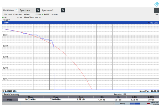
NTNV-N41-PC2-30-100-M-CP-64QPSK-Outer_Full-PASS
