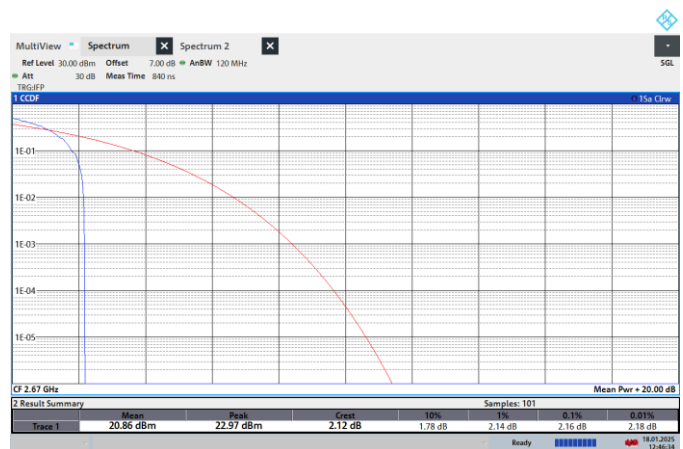
NTNV-N41-PC2-30-40-H-CP-64QPSK-Edge_1RB_Left-PASS
