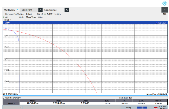
NTNV-N41-PC2-30-50-H-CP-QPSK-Edge_1RB_Left-PASS
