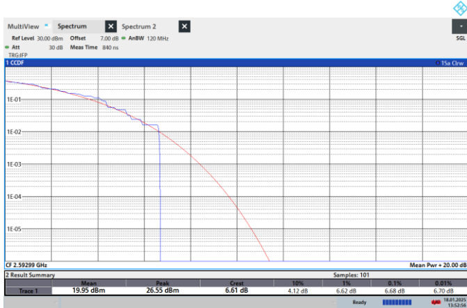
NTNV-N41-PC2-30-70-M-CP-16QPSK-Outer_Full-PASS
