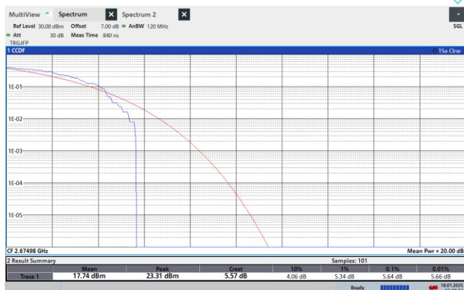
NTNV-N41-PC2-30-30-H-CP-256QPSK-Outer_Full-PASS
