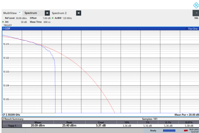
NTN-N41-PC2-30-50-M-CP-16QPSK-Outer_Full-PASS
