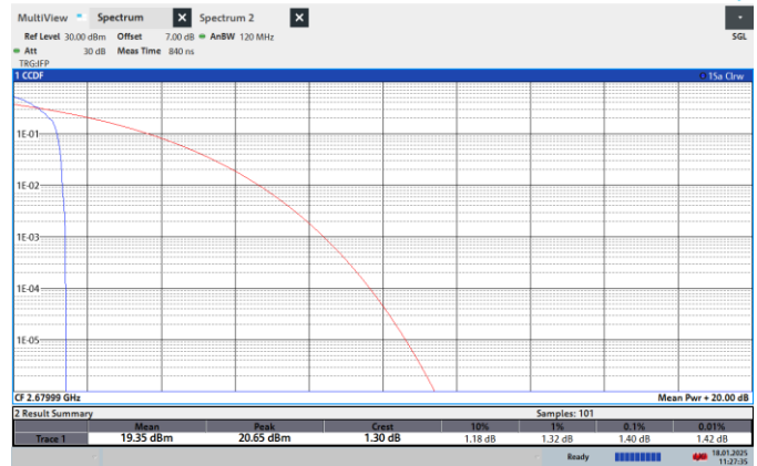
NTNV-N41-PC2-30-20-H-CP-256QPSK-Edge_1RB_Left-PASS
