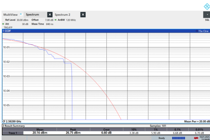
NTN-N41-PC2-30-50-M-CP-64QPSK-Outer_Full-PASS
