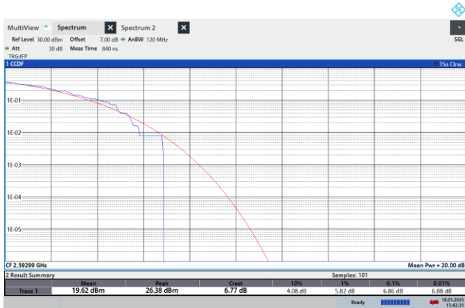
NTNV-N41-PC2-30-60-M-CP-64QPSK-Outer_Full-PASS
