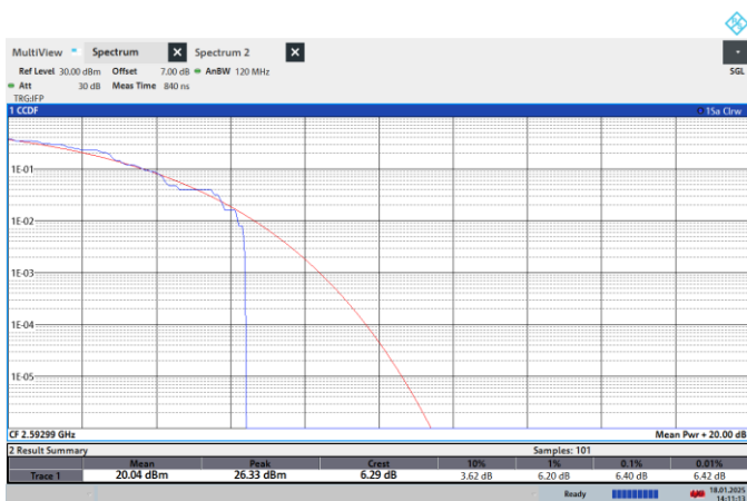
NTN-N41-PC2-30-80-M-CP-64QPSK-Outer_Full-PASS
