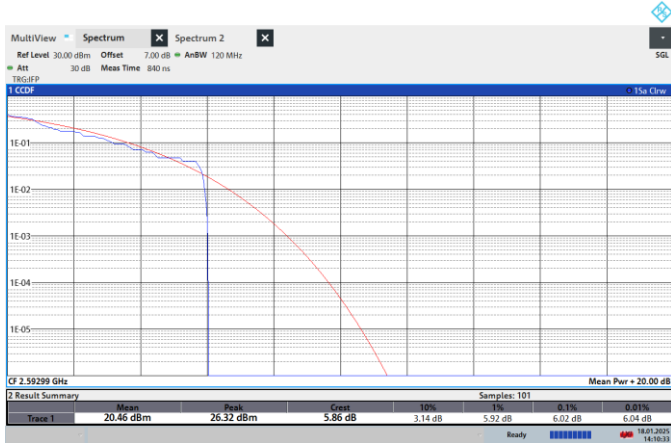
NTN-N41-PC2-30-80-M-CP-QPSK-Outer_Full-PASS
