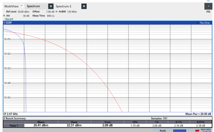
NTNV-N41-PC2-30-40-H-CP-QPSK-Edge_1RB_Left-PASS
