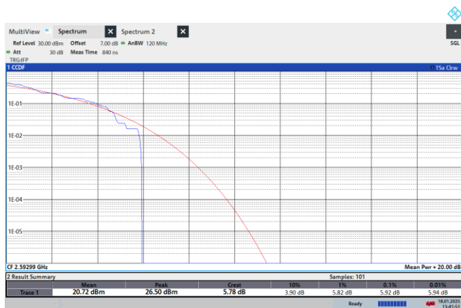
NTNV-N41-PC2-30-60-M-CP-QPSK-Outer_Full-PASS
