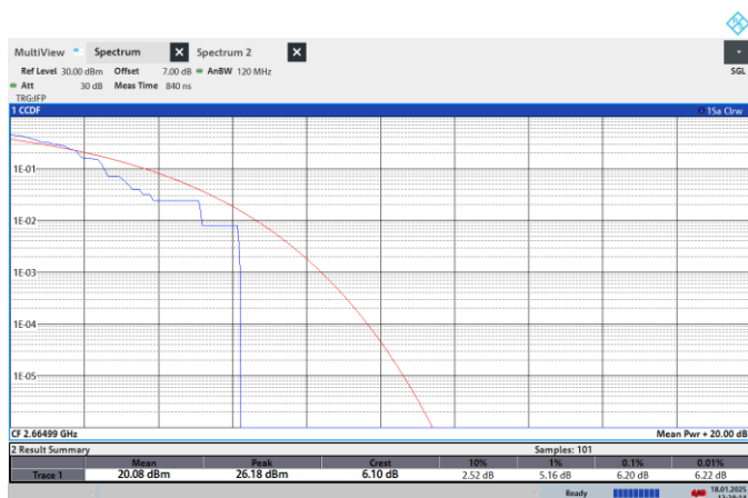
NTNV-N41-PC2-30-50-H-CP-64QPSK-Outer_Full-PASS
