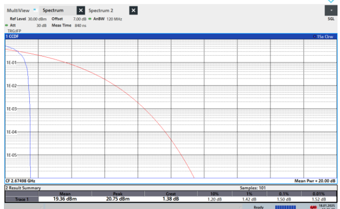
NTNV-N41-PC2-30-30-H-CP-256QPSK-Edge_1RB_Left-PASS
