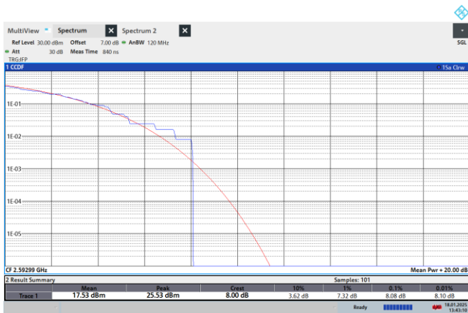
NTNV-N41-PC2-30-60-M-CP-256QPSK-Outer_Full-PASS
