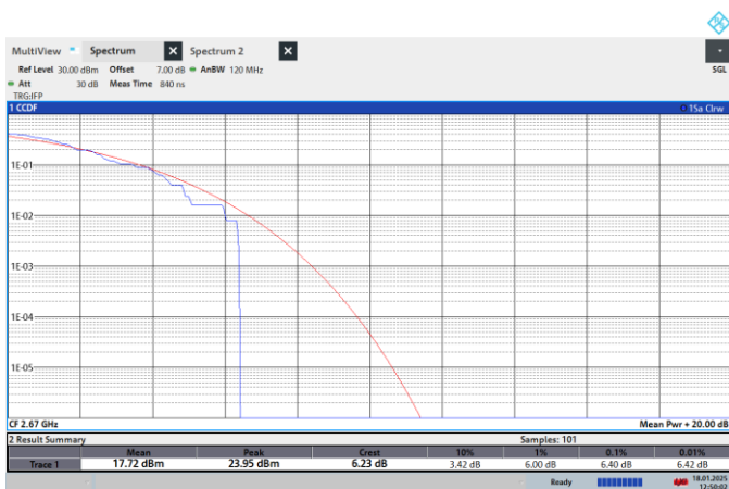
NTNV-N41-PC2-30-40-H-CP-256QPSK-Outer_Full-PASS
