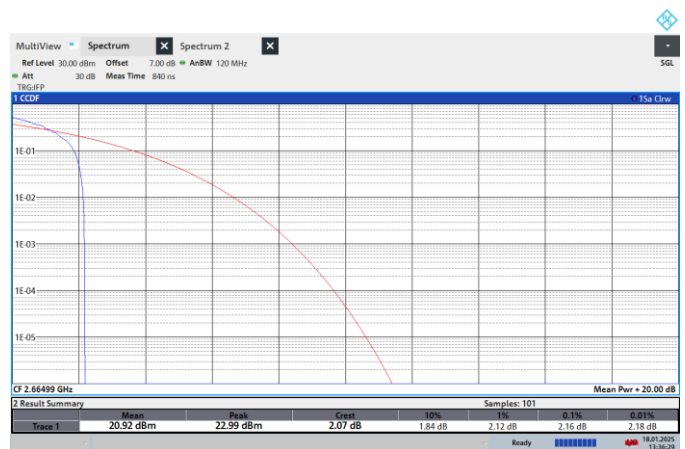
NTNV-N41-PC2-30-50-H-CP-16QPSK-Edge_1RB_Left-PASS
