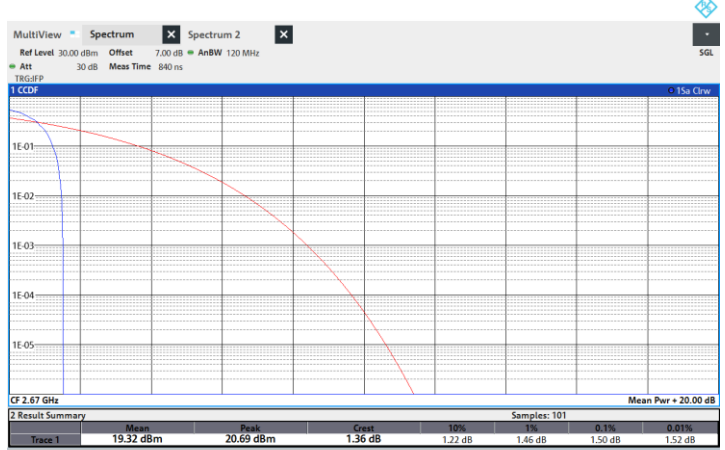
NTNV-N41-PC2-30-40-H-CP-256QPSK-Edge_1RB_Left-PASS
