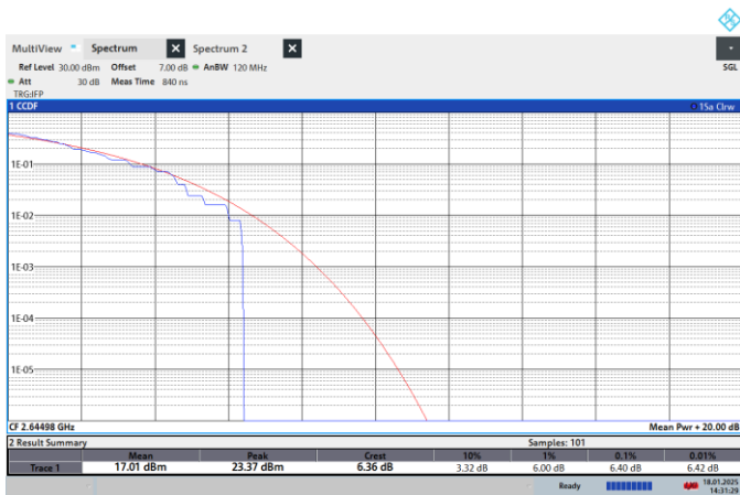
NTNV-N41-PC2-30-90-H-CP-256QPSK-Outer_Full-PASS
