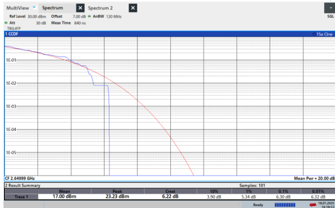
NTNV-N41-PC2-30-80-H-CP-256QPSK-Outer_Full-PASS
