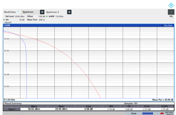
NTNV-N41-PC2-30-100-H-CP-QPSK-Edge_1RB_Left-PASS
