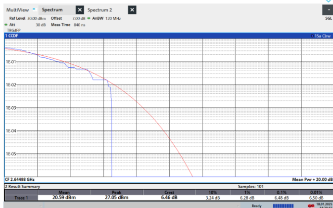
NTNV-N41-PC2-30-90-H-CP-16QPSK-Outer_Full-PASS
