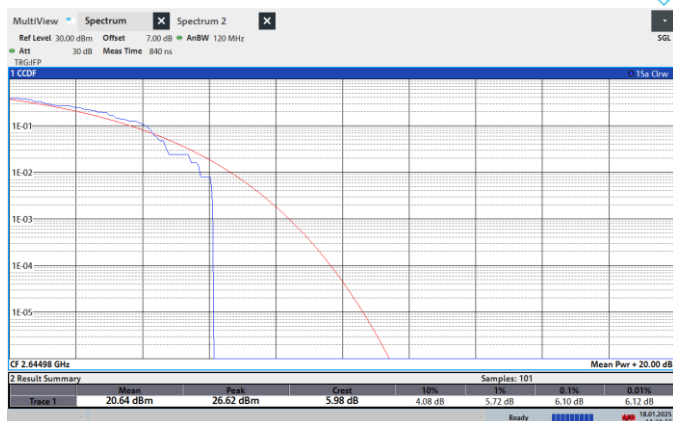
NTNV-N41-PC2-30-90-H-CP-QPSK-Outer_Full-PASS
