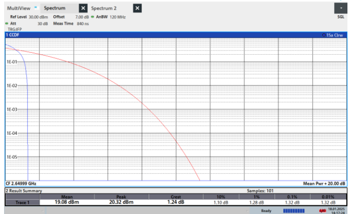
NTNV-N41-PC2-30-80-H-CP-256QPSK-Edge_1RB_Left-PASS
