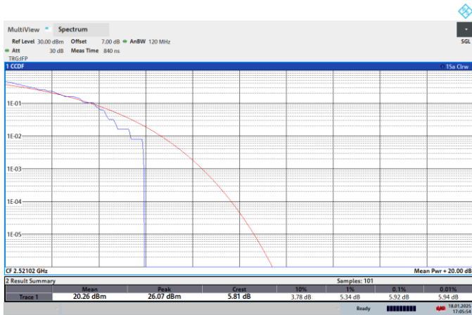
NTNV-N41-PC2-30-50-L-CP-64QPSK-Outer_Full-PASS
