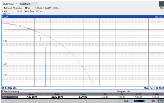
NTNV-N41-PC2-30-50-L-CP-256QPSK-Outer_Full-PASS
