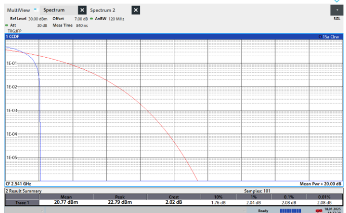
NTNV-N41-PC2-30-90-H-CP-16QPSK-Edge_1RB_Left-PASS
