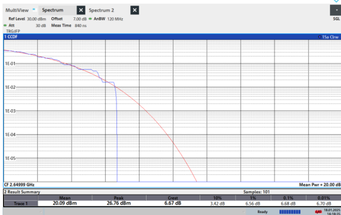
NTNV-N41-PC2-30-80-H-CP-64QPSK-Outer_Full-PASS
