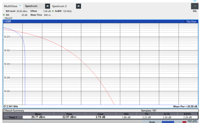
NTNV-N41-PC2-30-90-H-CP-QPSK-Edge_1RB_Left-PASS
