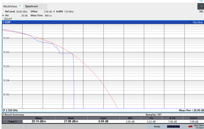
NTNV-N41-PC2-30-60-L-CP-QPSK-Outer_Full-PASS
