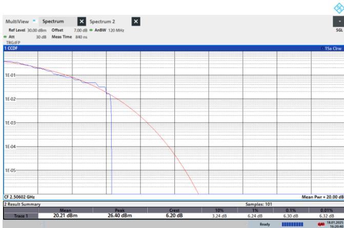
NTNV-N41-PC2-30-20-L-CP-QPSK-Outer_Full-PASS
