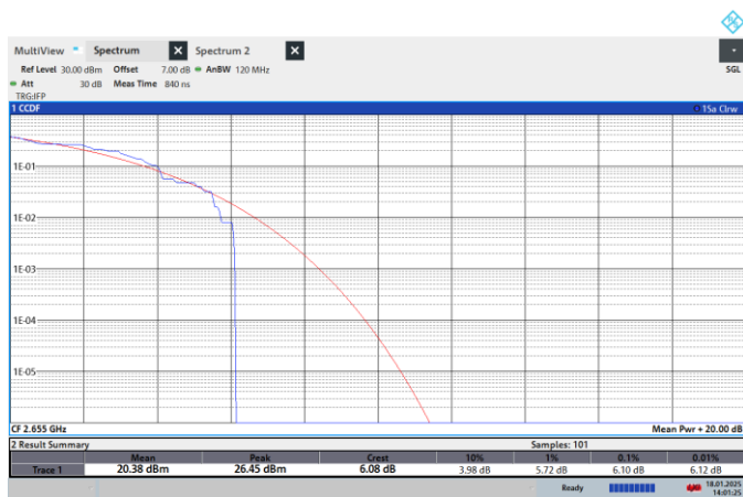
NTNV-N41-PC2-30-70-H-CP-64QPSK-Outer_Full-PASS
