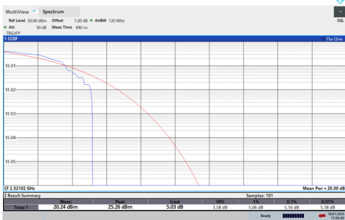
NTNV-N41-PC2-30-50-L-CP-16QPSK-Outer_Full-PASS
