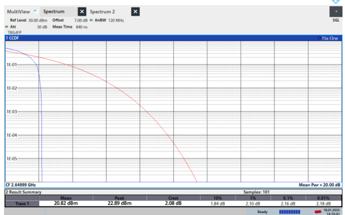
NTNV-N41-PC2-30-80-H-CP-16QPSK-Edge_1RB_Left-PASS
