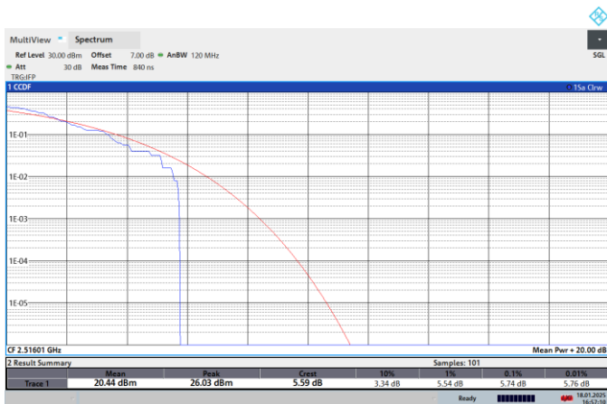
NTNV-N41-PC2-30-40-L-CP-QPSK-Outer_Full-PASS
