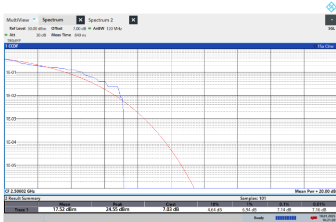
NTNV-N41-PC2-30-20-L-CP-256QPSK-Outer_Full-PASS
