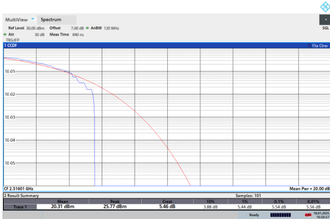
NTNV-N41-PC2-30-40-L-CP-16QPSK-Outer_Full-PASS
