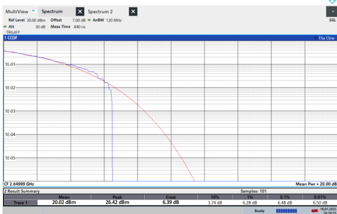
NTNV-N41-PC2-30-80-H-CP-16QPSK-Outer_Full-PASS
