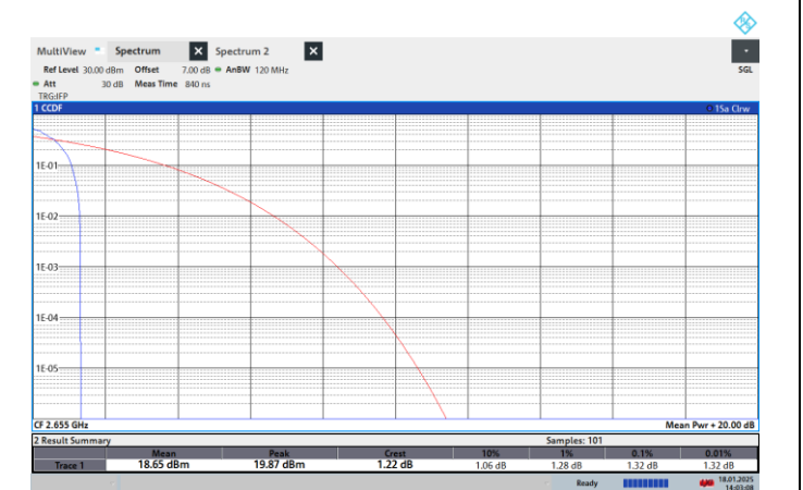
NTNV-N41-PC2-30-70-H-CP-256QPSK-Edge_1RB_Left-PASS
