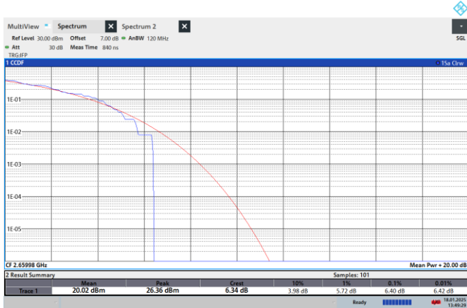
NTNV-N41-PC2-30-60-H-CP-64QPSK-Outer_Full-PASS
