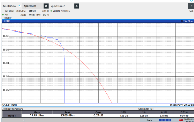
NTNV-N41-PC2-30-30-L-CP-256QPSK-Outer_Full-PASS
