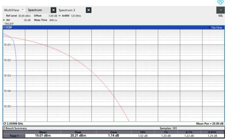
NTNV-N41-PC2-30-60-H-CP-256QPSK-Edge_1RB_Left-PASS
