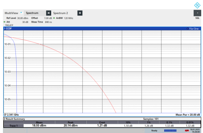
NTNV-N41-PC2-30-90-H-CP-256QPSK-Edge_1RB_Left-PASS
