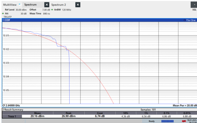
NTNV-N41-PC2-30-80-H-CP-QPSK-Outer_Full-PASS
