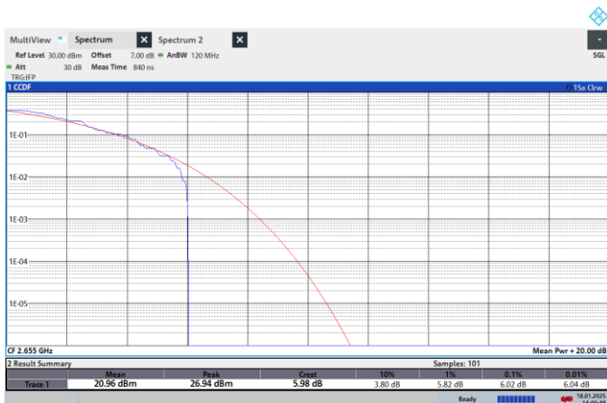
NTNV-N41-PC2-30-70-H-CP-QPSK-Outer_Full-PASS
