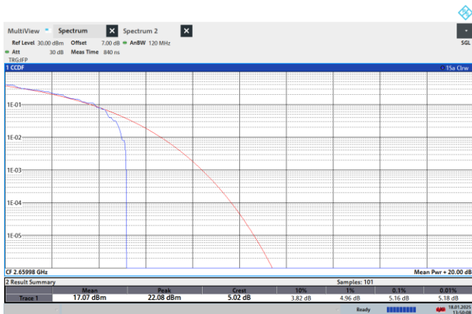
NTNV-N41-PC2-30-60-H-CP-256QPSK-Outer_Full-PASS
