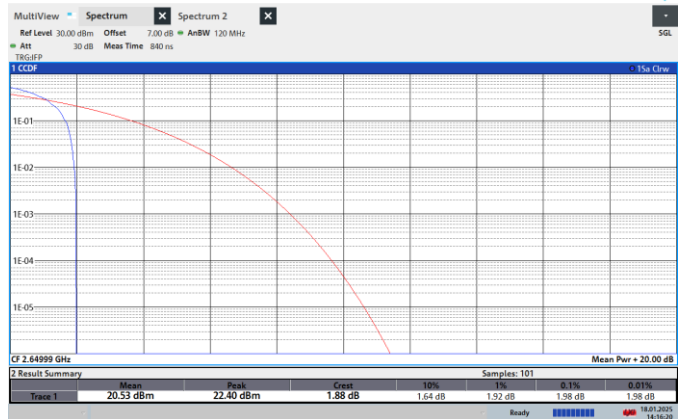
NTNV-N41-PC2-30-80-H-CP-QPSK-Edge_1RB_Left-PASS
