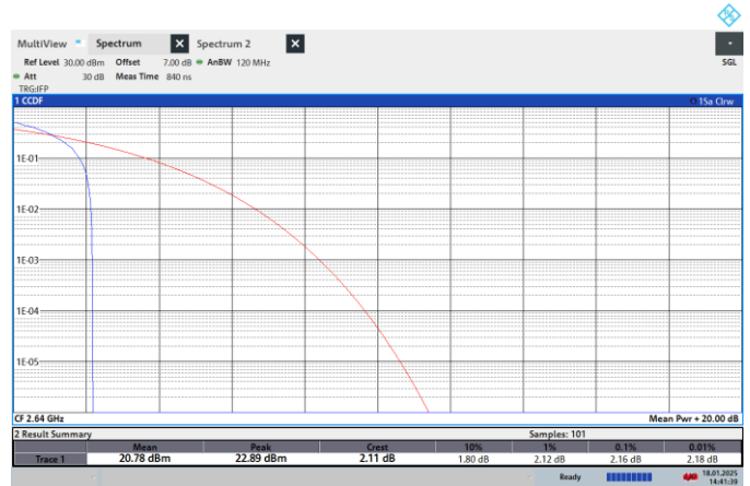
NTNV-N41-PC2-30-100-H-CP-16QPSK-Edge_1RB_Left-PASS
