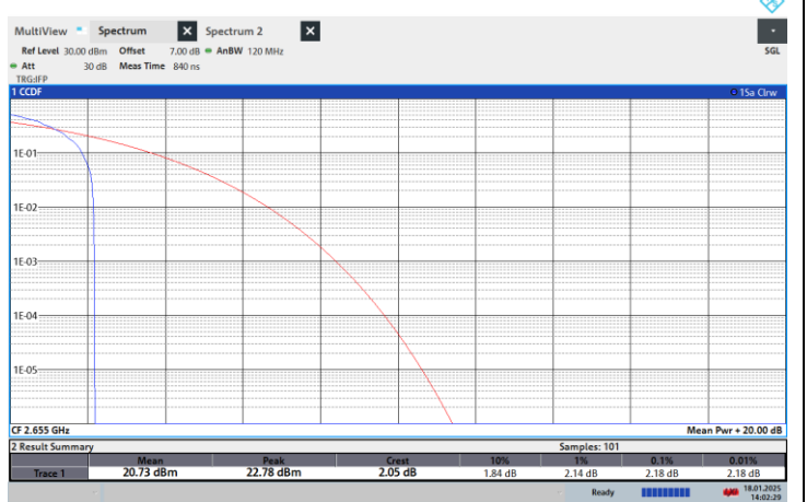
NTNV-N41-PC2-30-70-H-CP-16QPSK-Edge_1RB_Left-PASS
