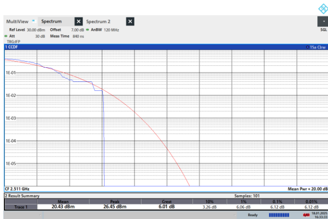
NTNV-N41-PC2-30-30-L-CP-QPSK-Outer_Full-PASS
