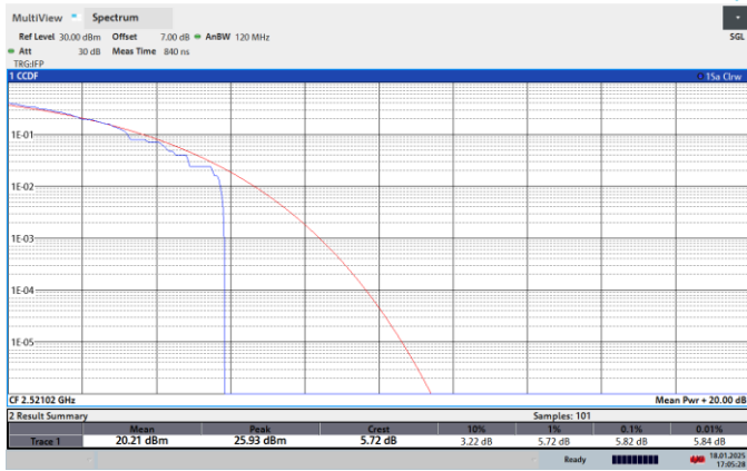
NTNV-N41-PC2-30-50-L-CP-QPSK-Outer_Full-PASS
