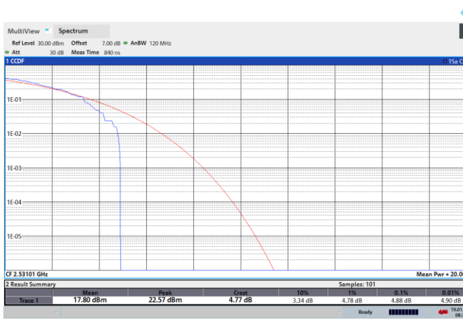
NTNV-N41-PC2-30-70-L-CP-QPSK-Outer_Full-PASS
