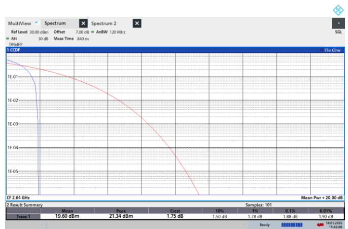
NTNV-N41-PC2-30-100-H-CP-64QPSK-Edge_1RB_Left-PASS
