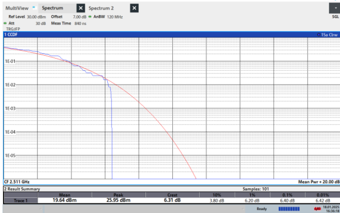
NTNV-N41-PC2-30-30-L-CP-64QPSK-Outer_Full-PASS
