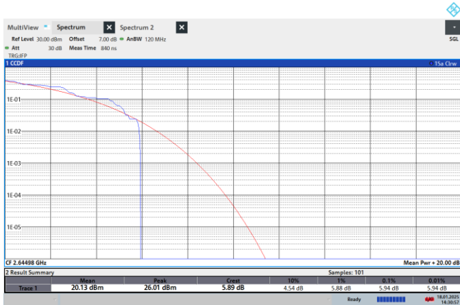
NTNV-N41-PC2-30-90-H-CP-64QPSK-Outer_Full-PASS
