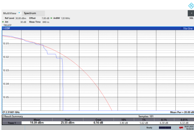
NTNV-N41-PC2-30-40-L-CP-64QPSK-Outer_Full-PASS
