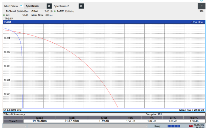
NTNV-N41-PC2-30-80-H-CP-64QPSK-Edge_1RB_Left-PASS
