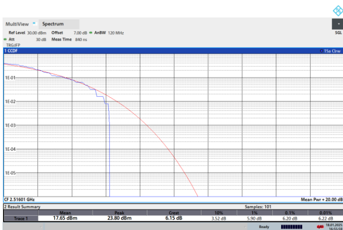
NTNV-N41-PC2-30-40-L-CP-256QPSK-Outer_Full-PASS
