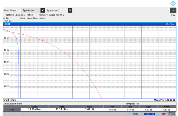
NTNV-N41-PC2-30-90-H-CP-64QPSK-Edge_1RB_Left-PASS
