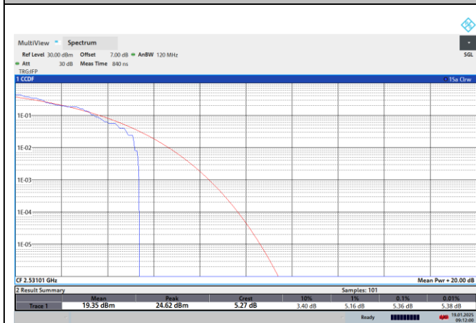
NTNV-N41-PC2-30-70-L-CP-64QPSK-Outer_Full-PASS
