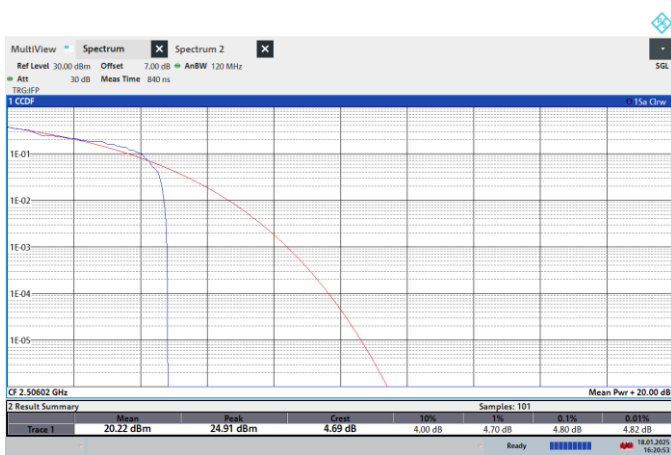
NTNV-N41-PC2-30-20-L-CP-16QPSK-Outer_Full-PASS
