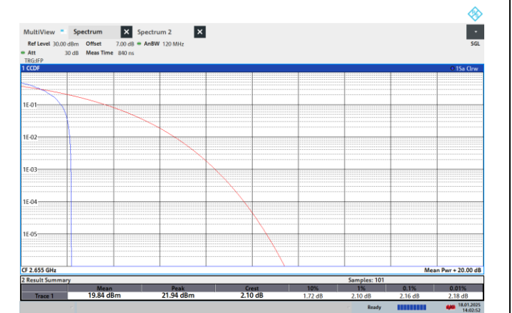
NTNV-N41-PC2-30-70-HM-CP-64QPSK-Edge_1RB_Left-PASS
