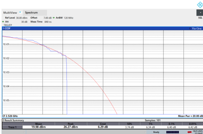
NTNV-N41-PC2-30-60-L-CP-16QPSK-Outer_Full-PASS
