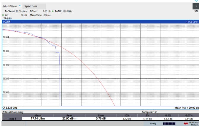
NTNV-N41-PC2-30-60-L-CP-256QPSK-Outer_Full-PASS
