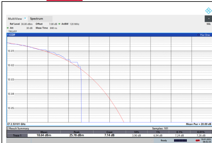
NTNV-N41-PC2-30-70-L-CP-16QPSK-Outer_Full-PASS
