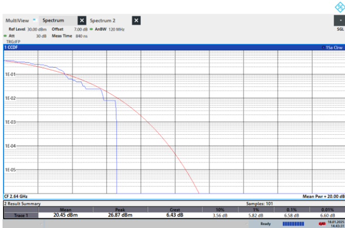
NTNV-N41-PC2-30-100-H-CP-16QPSK-Outer_Full-PASS
