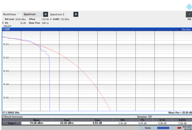
NTNV-N41-PC2-30-20-L-CP-64QPSK-Outer_Full-PASS
