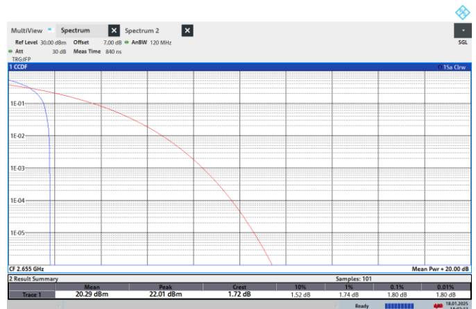
NTNV-N41-PC2-30-70-H-CP-QPSK-Edge_1RB_Left-PASS
