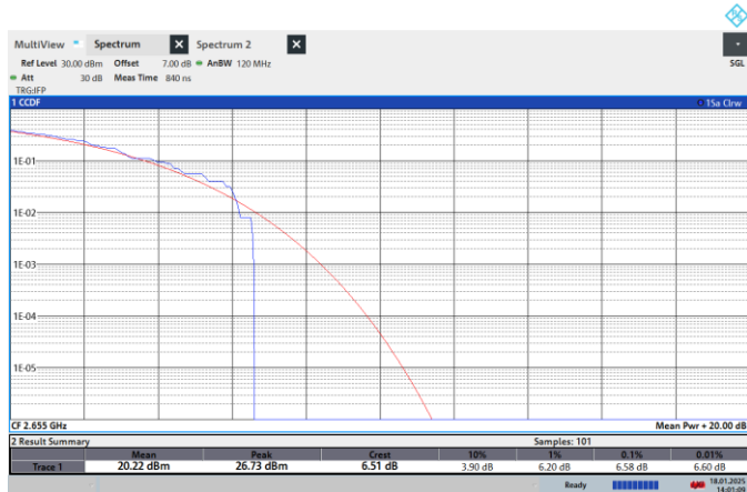
NTNV-N41-PC2-30-70-H-CP-16QPSK-Outer_Full-PASS
