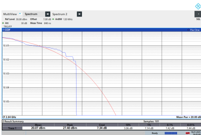
NTNV-N41-PC2-30-100-H-CP-QPSK-Outer_Full-PASS
