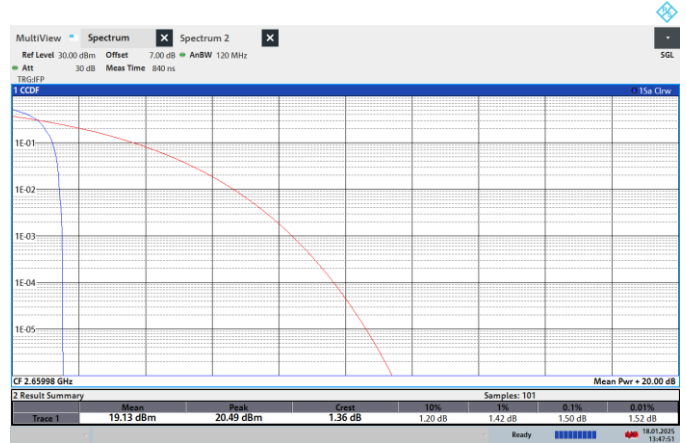
NTNV-N41-PC2-30-60-H-CP-64QPSK-Edge_1RB_Left-PASS
