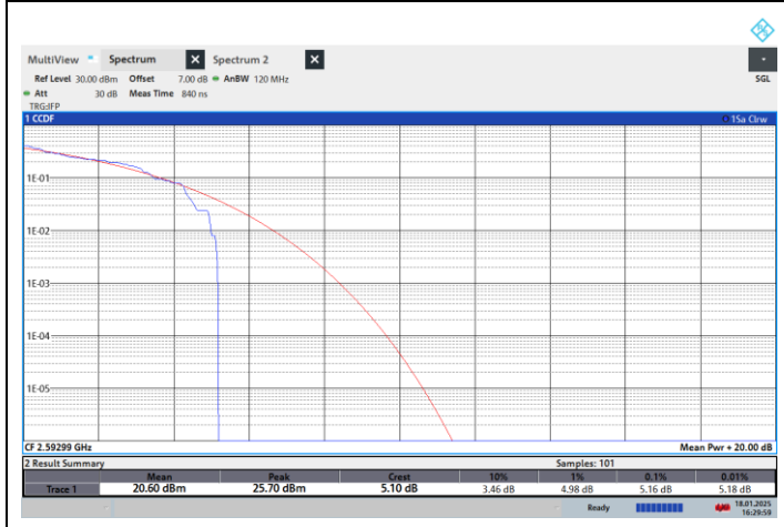
NTNV-N41-PC2-30-M-CP-QPSK-Outer_Full-PASS
