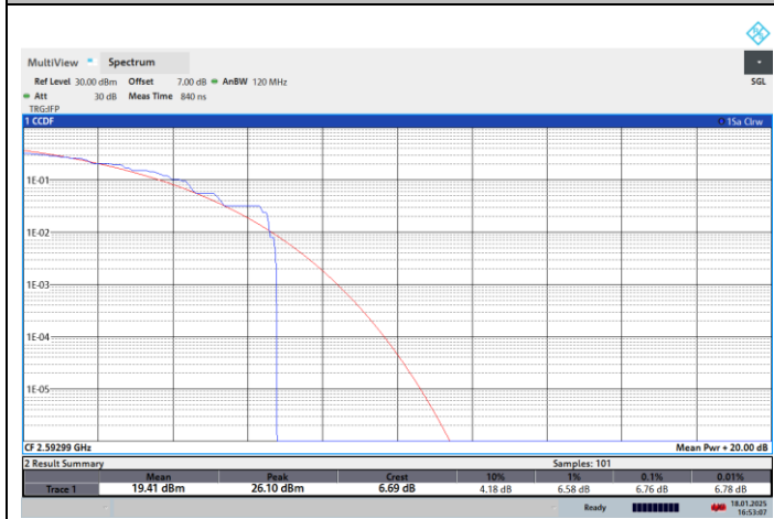
NTNV-N41-PC2-30-40-M-CP-64QPSK-Outer_Full-PASS
