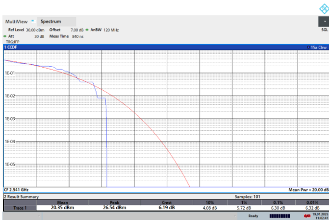
NTNV-N41-PC2-30-90-L-CP-QPSK-Outer_Full-PASS
