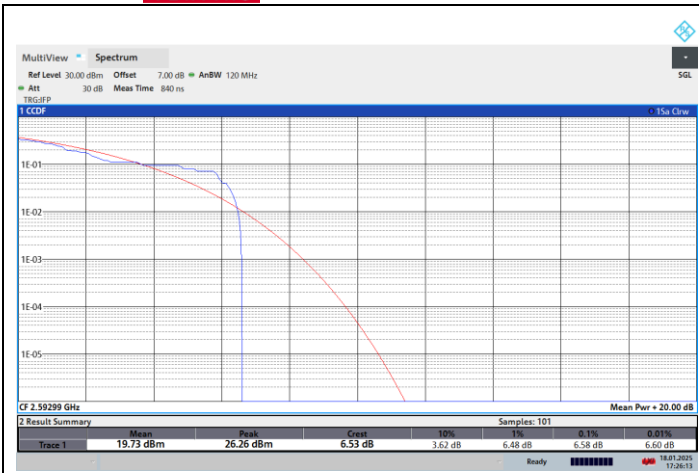
NTNV-N41-PC2-30-70-M-CP-16QPSK-Outer_Full-PASS
