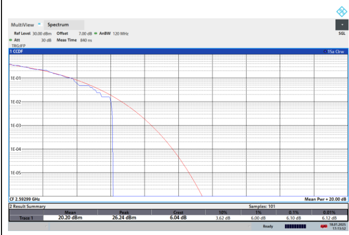
NTNV-N41-PC2-30-60-M-CP-QPSK-Outer_Full-PASS
