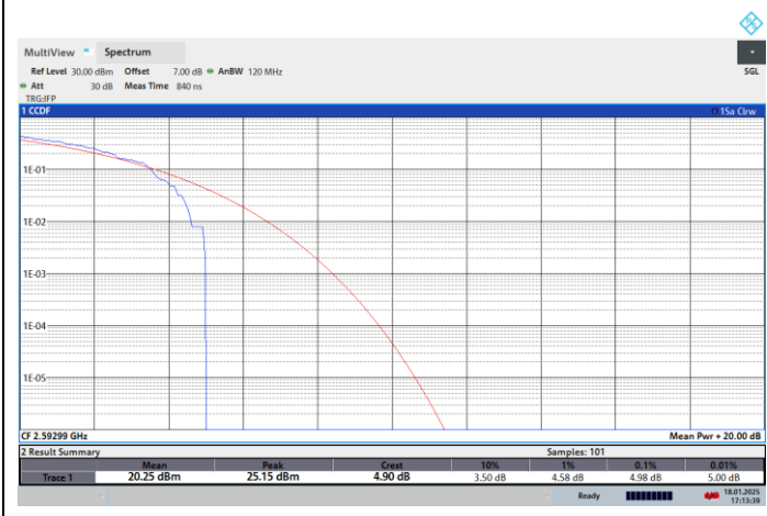
NTNV-N41-PC2-30-60-M-CP-16QPSK-Outer_Full-PASS
