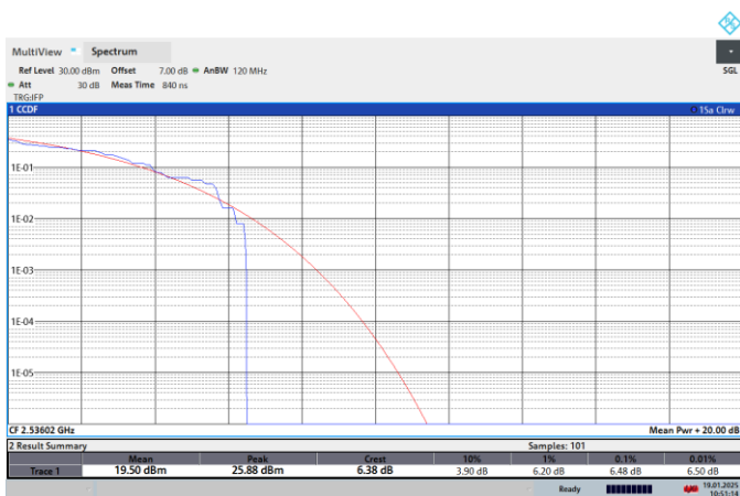
NTNV-N41-PC2-30-80-L-CP-64QPSK-Outer_Full-PASS
