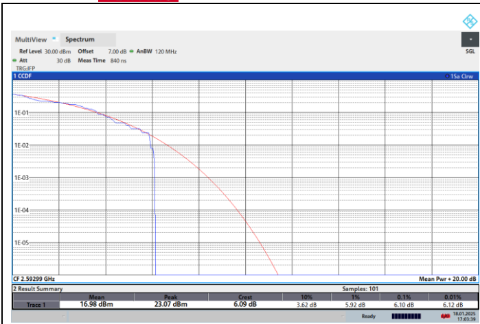
NTNV-N41-PC2-30-50-M-CP-256QPSK-Outer_Full-PASS
