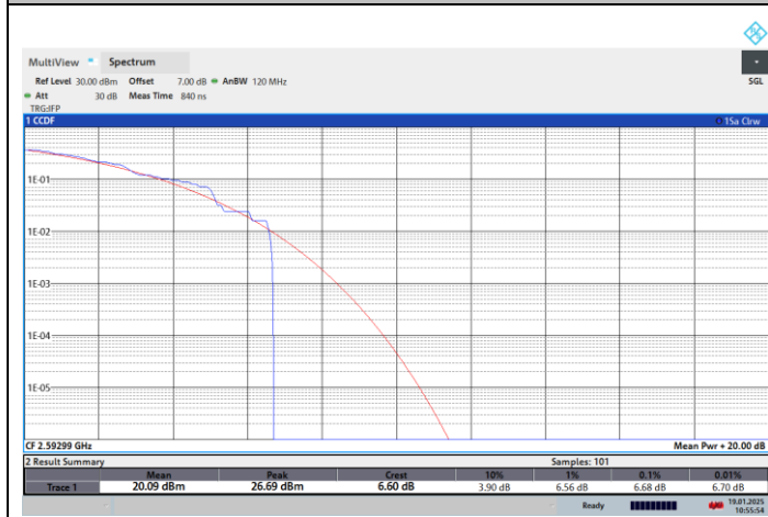
NTNV-N41-PC2-30-90-M-CP-QPSK-Outer_Full-PASS
