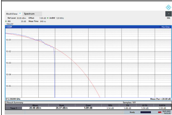
NTNV-N41-PC2-30-40-M-CP-QPSK-Outer_Full-PASS
