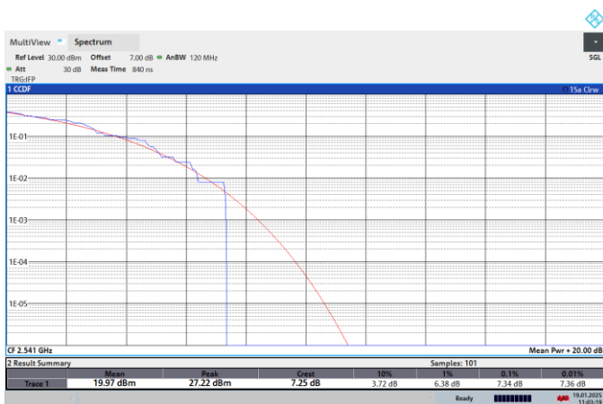
NTNV-N41-PC2-30-90-L-CP-16QPSK-Outer_Full-PASS
