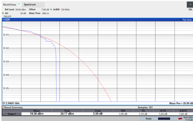
NTNV-N41-PC2-30-100-L-CP-16QPSK-Outer_Full-PASS
