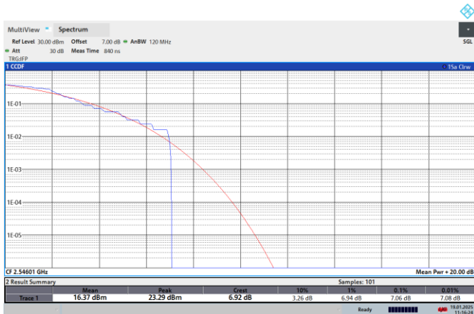
NTNV-N41-PC2-30-100-L-CP-256QPSK-Outer_Full-PASS
