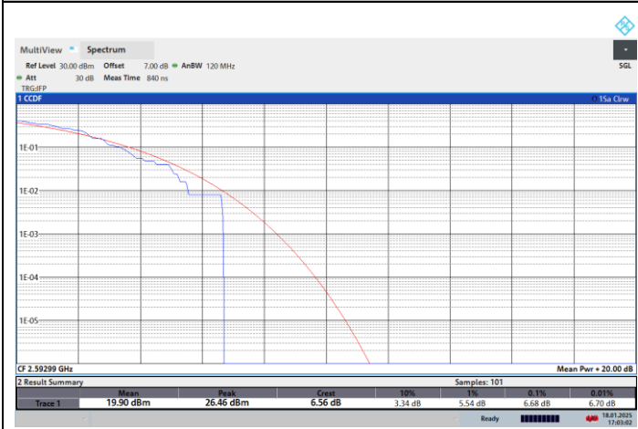
NTNV-N41-PC2-30-50-M-CP-64QPSK-Outer_Full-PASS
