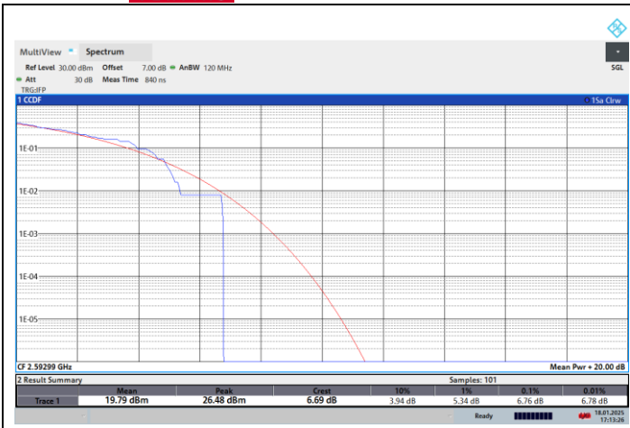
NTNV-N41-PC2-30-60-M-CP-64QPSK-Outer_Full-PASS
