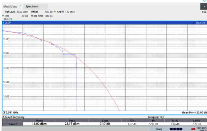
NTNV-N41-PC2-30-90-L-CP-256QPSK-Outer_Full-PASS
