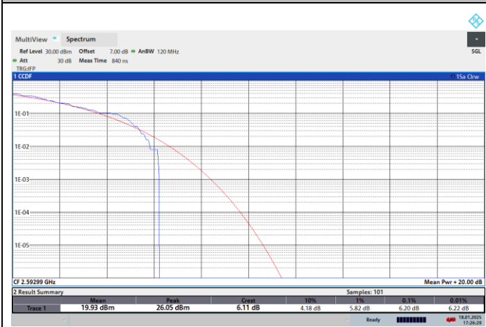
NTNV-N41-PC2-30-70-M-CP-64QPSK-Outer_Full-PASS
