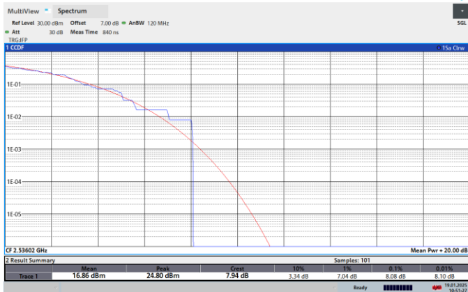
NTNV-N41-PC2-30-80-L-CP-256QPSK-Outer_Full-PASS
