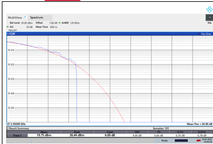
NTNV-N41-PC2-30-80-M-CP-256QPSK-Outer_Full-PASS
