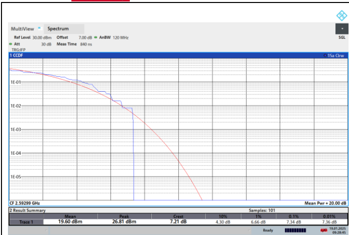
NTNV-N41-PC2-30-80-M-CP-QPSK-Outer_Full-PASS
