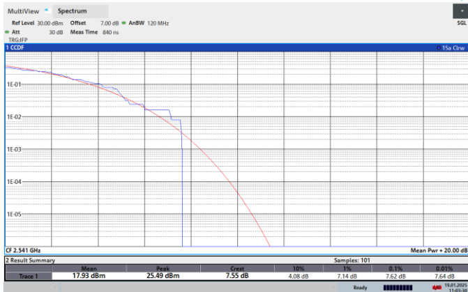
NTNV-N41-PC2-30-90-L-CP-64QPSK-Outer_Full-PASS
