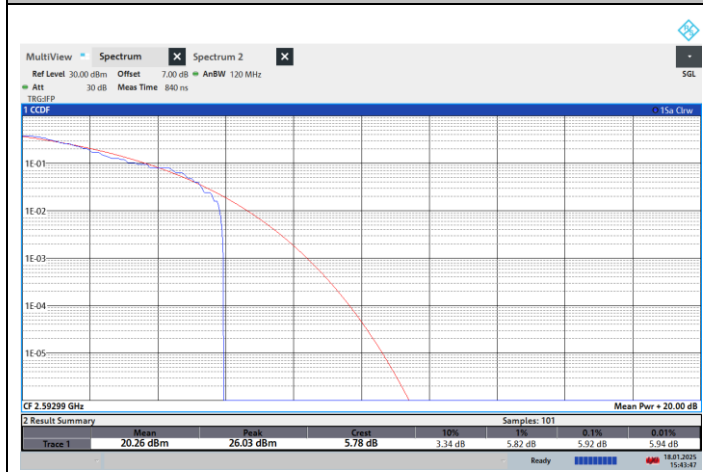
NTNV-N41-PC2-30-20-M-CP-64QPSK-Outer_Full-PASS
