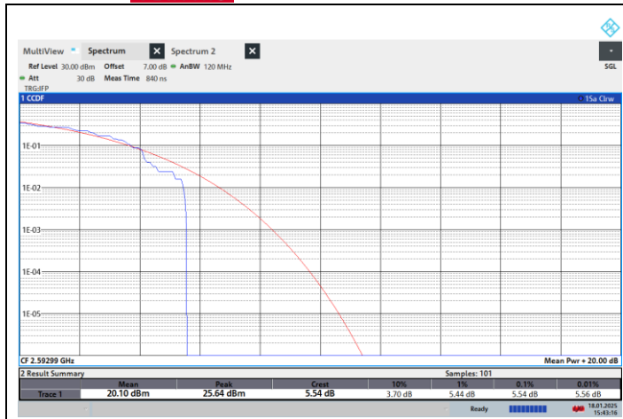
NTNV-N41-PC2-30-20-M-CP-QPSK-Outer_Full-PASS
