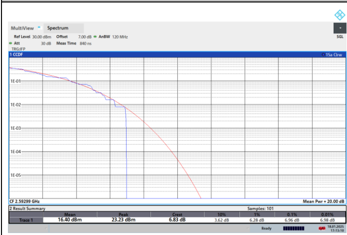
NTNV-N41-PC2-30-60-M-CP-256QPSK-Outer_Full-PASS
