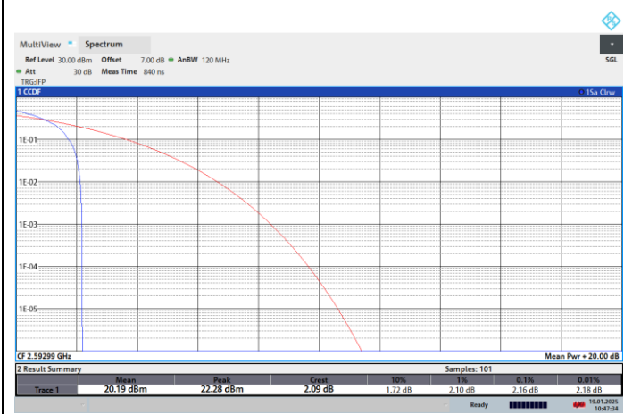
NTNV-N41-PC2-30-80-M-CP-16QPSK-Outer_Full-PASS
