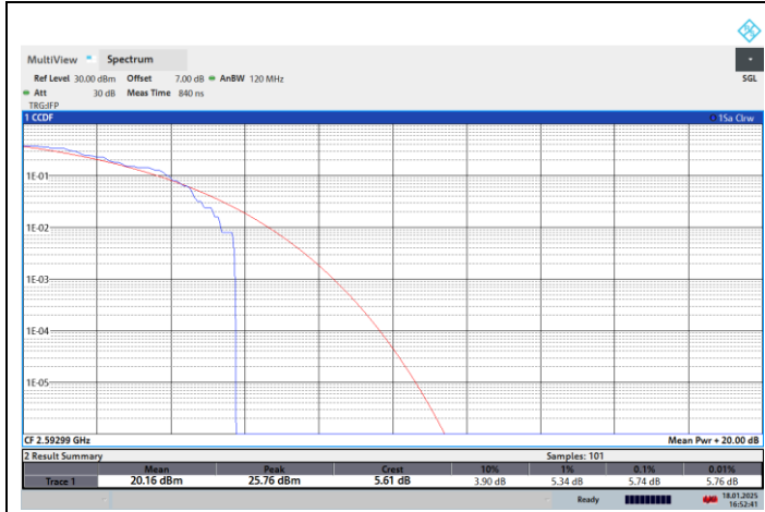
NTNV-N41-PC2-30-40-M-CP-16QPSK-Outer_Full-PASS
