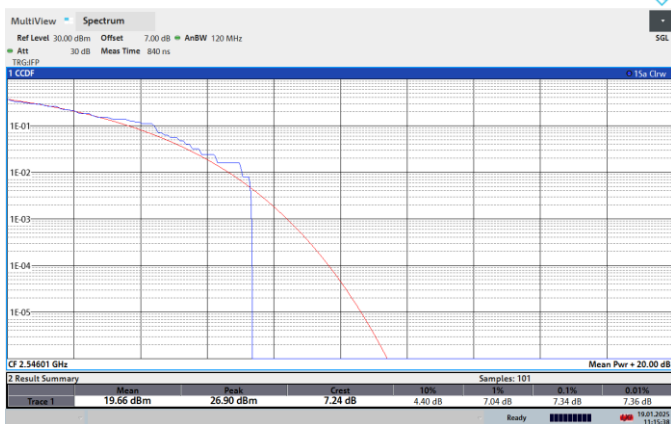
NTNV-N41-PC2-30-100-L-CP-64QPSK-Outer_Full-PASS
