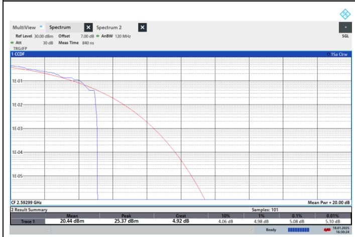
NTNV-N41-PC2-30-30-M-CP-16QPSK-Outer_Full-PASS
