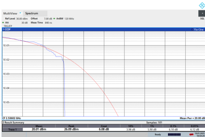
NTNV-N41-PC2-30-80-L-CP-16QPSK-Outer_Full-PASS
