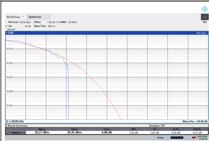
NTNV-N41-PC2-30-70-M-CP-QPSK-Outer_Full-PASS
