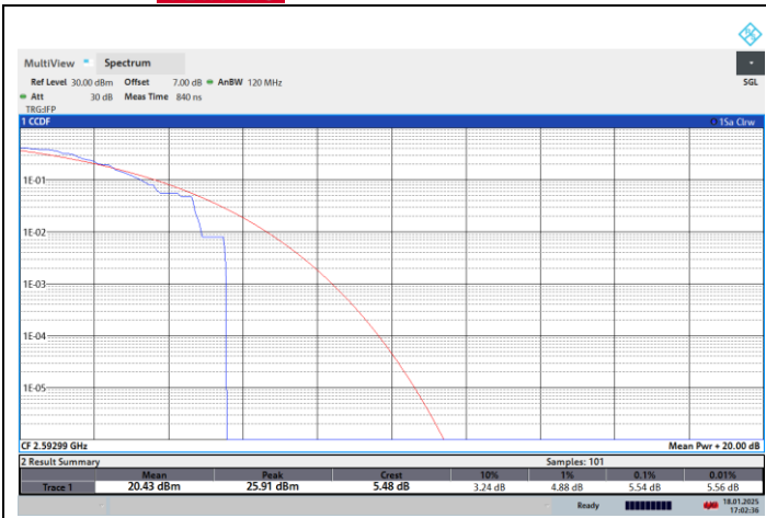
NTNV-N41-PC2-30-50-M-CP-QPSK-Outer_Full-PASS
