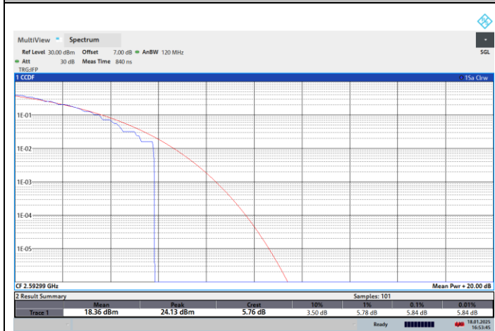
NTNV-N41-PC2-30-40-M-CP-256QPSK-Outer_Full-PASS
