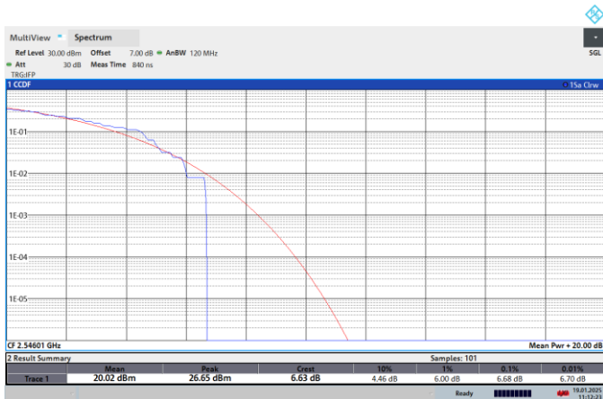
NTNV-N41-PC2-30-100-L-CP-QPSK-Outer_Full-PASS
