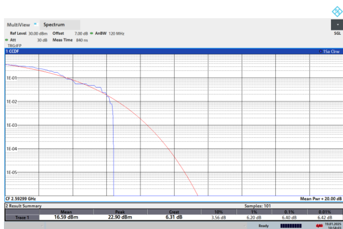
NTNV-N41-PC2-30-90-M-CP-256QPSK-Outer_Full-PASS
