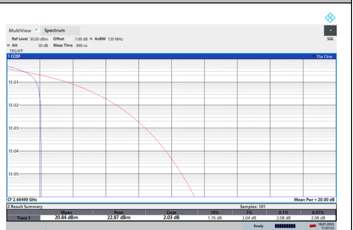
NTNV-N41-PC2-30-50-H-CP-16QPSK-Edge_1RB_Left-PASS
