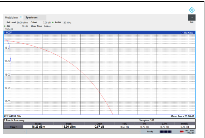
NTNV-N41-PC2-30-80-H-CP-QPSK-Edge_1RB_Left-PASS
