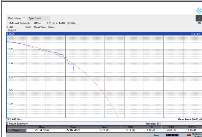
NTNV-N41-PC2-30-70-H-CP-64QPSK-Outer_Full-PASS
