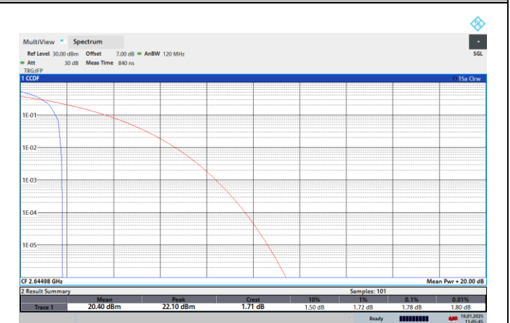
NTNV-N41-PC2-30-90-H-CP-16QPSK-Edge_1RB_Left-PASS
