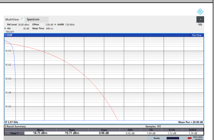
NTNV-N41-PC2-30-40-H-CP-256QPSK-Edge_1RB_Left-PASS
