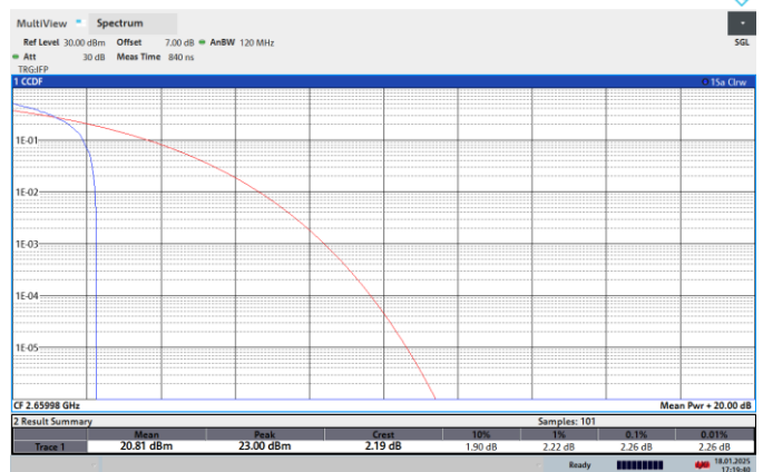
NTNV-N41-PC2-30-60-H-CP-QPSK-Edge_1RB_Left-PASS
