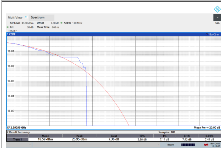
NTNV-N41-PC2-30-100-M-CP-64QPSK-Outer_Full-PASS
