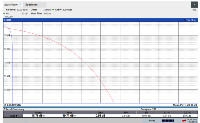
NTNV-N41-PC2-30-50-H-CP-256QPSK-Edge_1RB_Left-PASS
