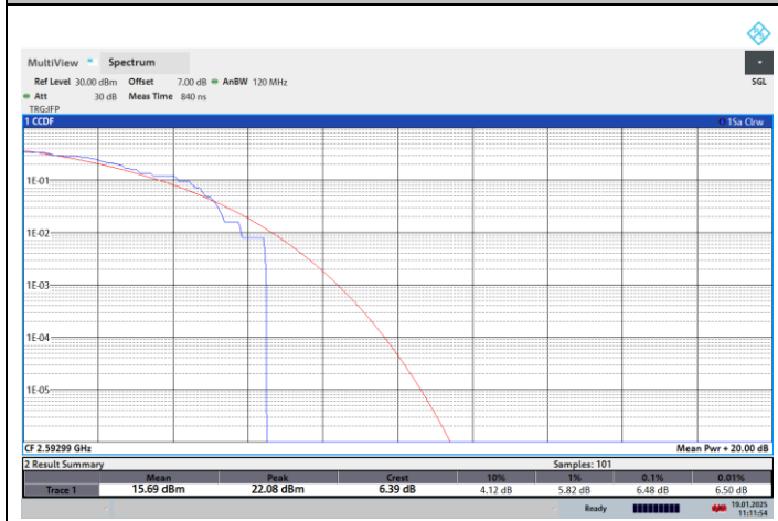
NTNV-N41-PC2-30-100-M-CP-256QPSK-Outer_Full-PASS
