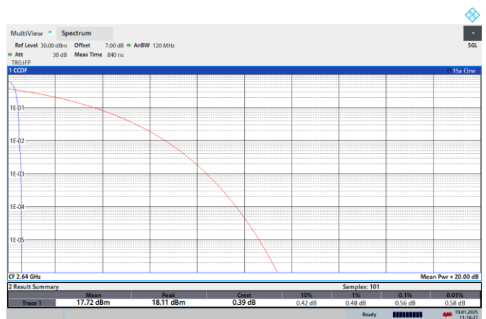
NTNV-N41-PC2-30-100-H-CP-256QPSK-Edge_1RB_Left-PASS
