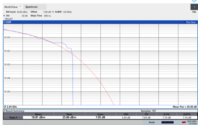
NTNV-N41-PC2-30-100-H-CP-64QPSK-Outer_Full-PASS
