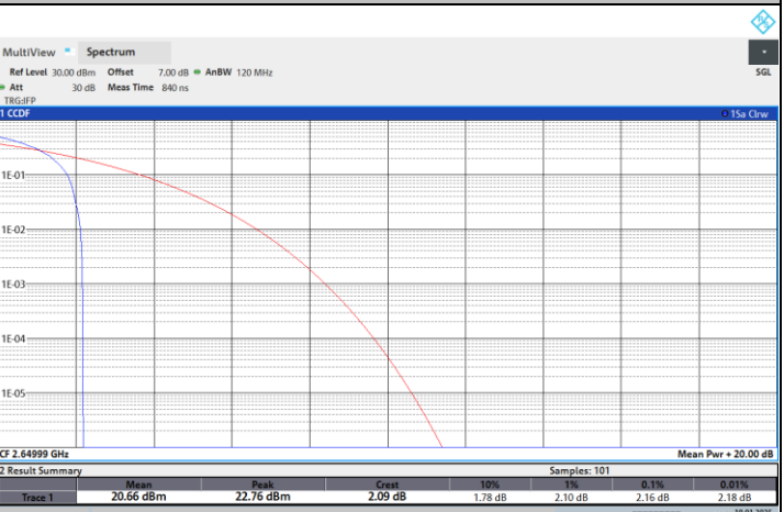
NTNV-N41-PC2-30-80-H-CP-64QPSK-Edge_1RB_Left-PASS
