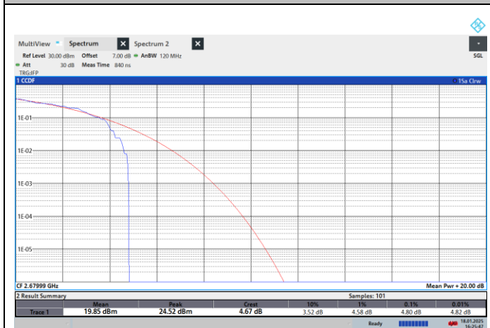
NTNV-N41-PC2-30-20-HM-CP-64QPSK-Outer_Full-PASS
