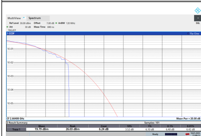
NTNV-N41-PC2-30-50-H-CP-64QPSK-Outer_Full-PASS
