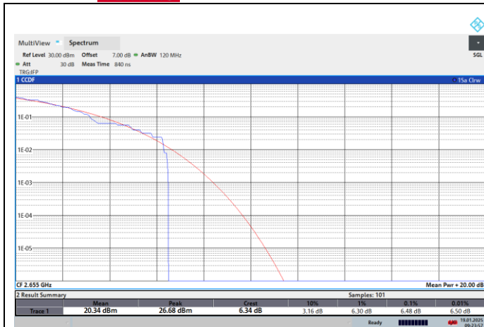
NTNV-N41-PC2-30-70-H-CP-16QPSK-Outer_Full-PASS
