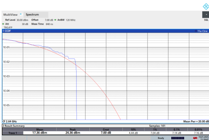
NTNV-N41-PC2-30-100-H-CP-256QPSK-Outer_Full-PASS
