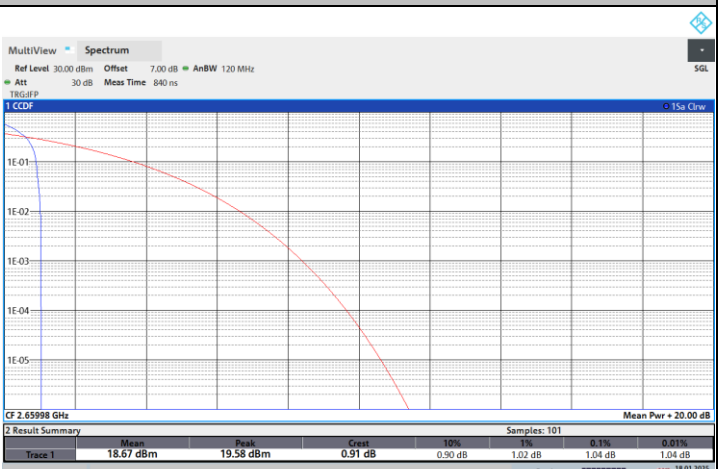
NTNV-N41-PC2-30-60-H-CP-256QPSK-Edge_1RB_Left-PASS
