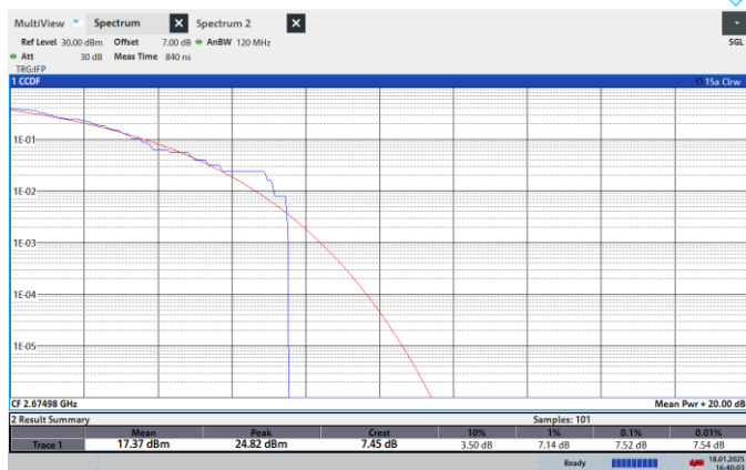
NTNV-N41-PC2-30-30-H-CP-256QPSK-Outer_Full-PASS
