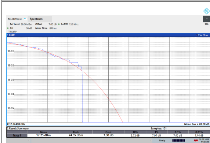
NTNV-N41-PC2-30-90-H-CP-256QPSK-Outer_Full-PASS
