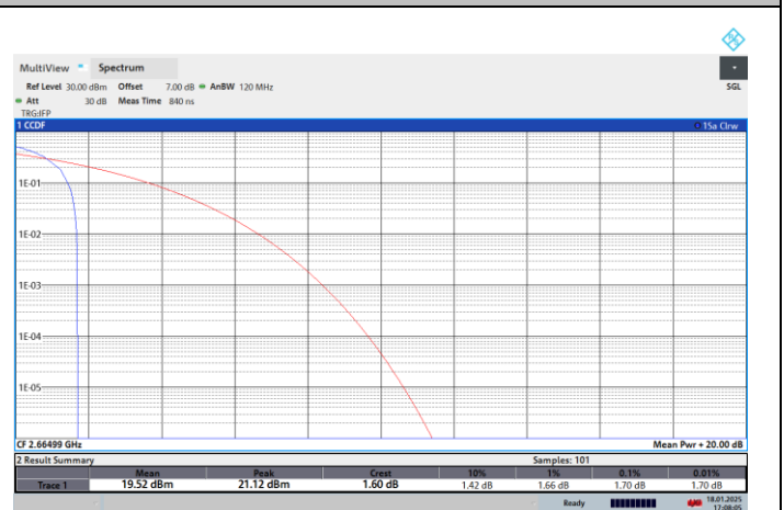
NTNV-N41-PC2-30-50-H-CP-64QPSK-Edge_1RB_Left-PASS
