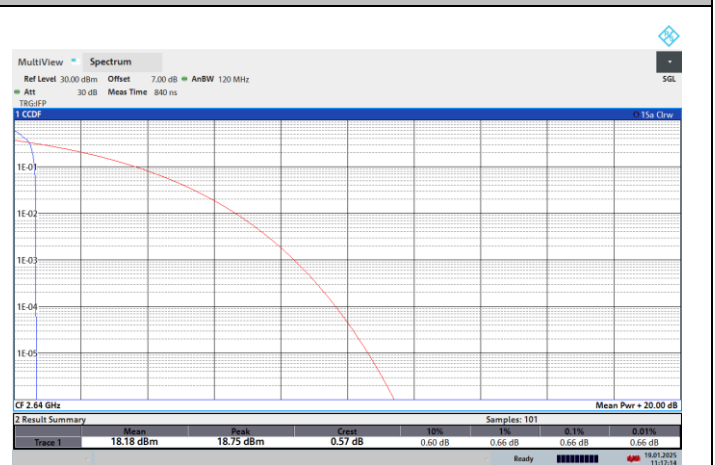
NTNV-N41-PC2-30-100-H-CP-QPSK-Edge_1RB_Left-PASS
