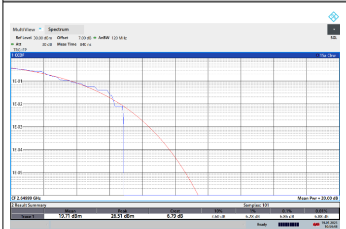
NTNV-N41-PC2-30-80-H-CP-64QPSK-Outer_Full-PASS
