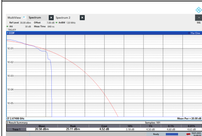
NTNV-N41-PC2-30-30-H-CP-16QPSK-Outer_Full-PASS
