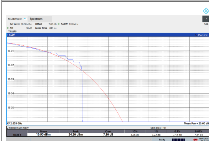
NTNV-N41-PC2-30-70-H-CP-256QPSK-Outer_Full-PASS
