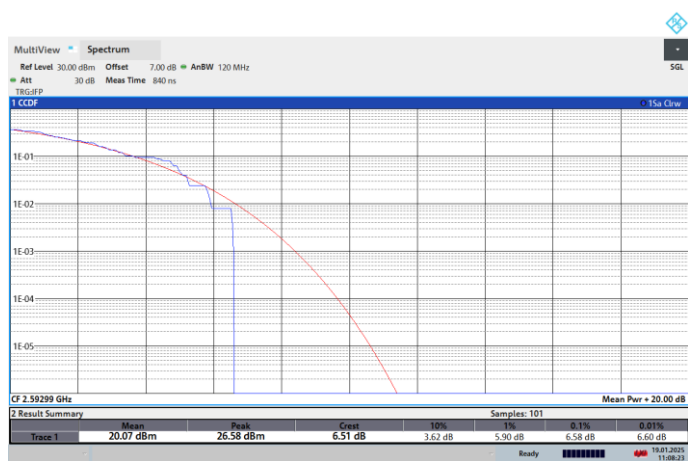
NTNV-N41-PC2-30-100-M-CP-QPSK-Outer_Full-PASS
