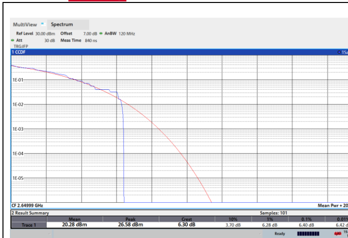
NTNV-N41-PC2-30-80-H-CP-QPSK-Outer_Full-PASS
