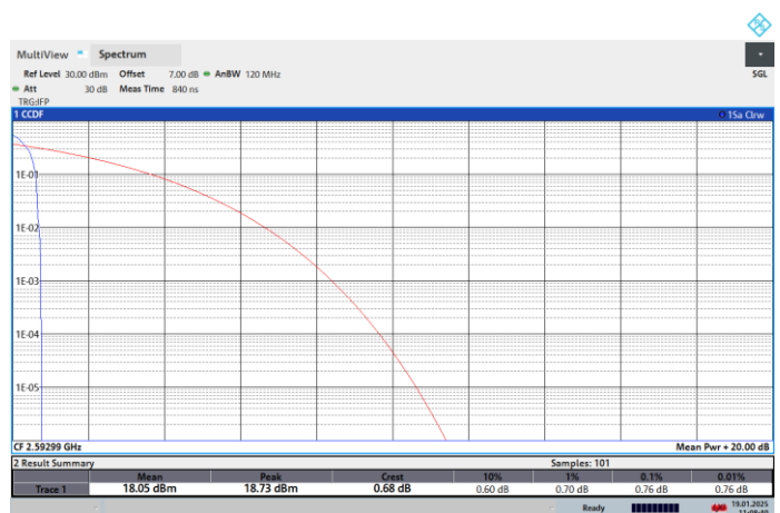
NTNV-N41-PC2-30-100-M-CP-QPSK-Edge_1RB_Left-PASS
