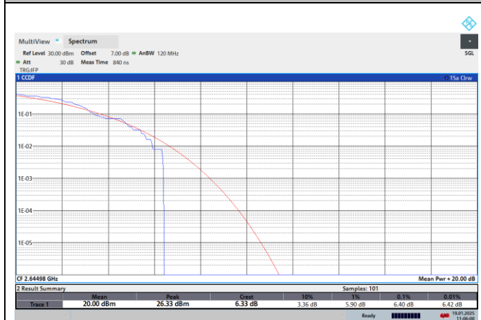
NTNV-N41-PC2-30-90-H-CP-16QPSK-Outer_Full-PASS
