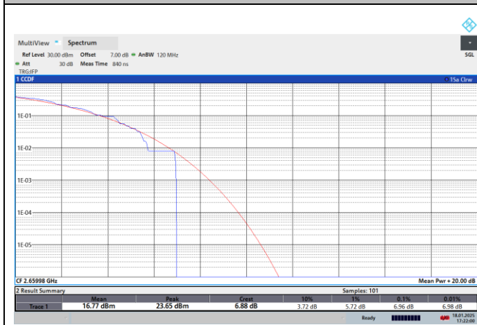
NTNV-N41-PC2-30-60-H-CP-256QPSK-Outer_Full-PASS
