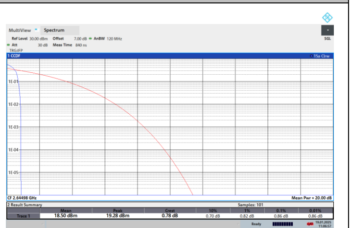
NTNV-N41-PC2-30-90-H-CP-256QPSK-Edge_1RB_Left-PASS
