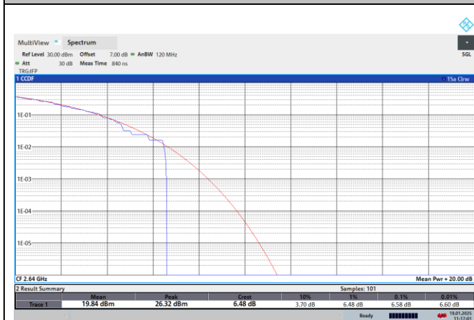
NTNV-N41-PC2-30-100-H-CP-QPSK-Outer_Full-PASS
