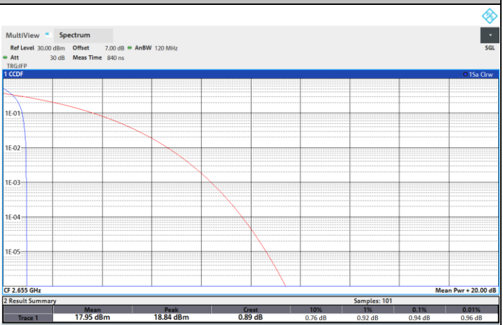
NTNV-N41-PC2-30-70-HM-CP-64QPSK-Edge_1RB_Left-PASS
