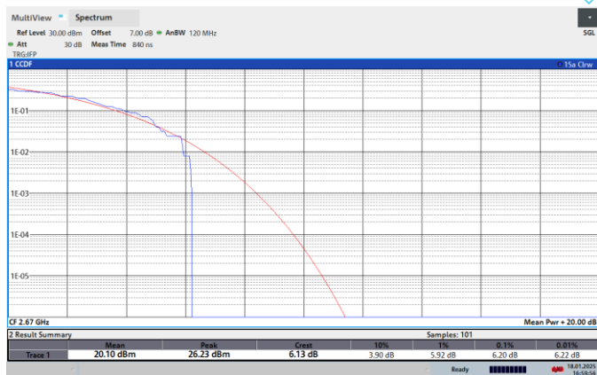
NTNV-N41-PC2-30-40-H-CP-QPSK-Outer_Full-PASS
