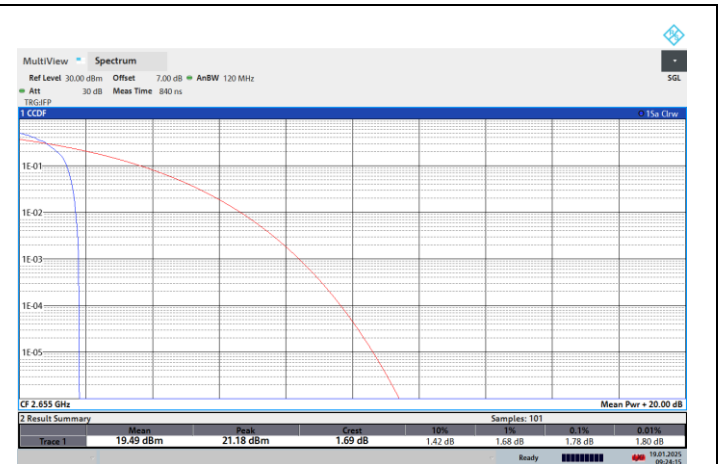
NTNV-N41-PC2-30-70-H-CP-16QPSK-Edge_1RB_Left-PASS
