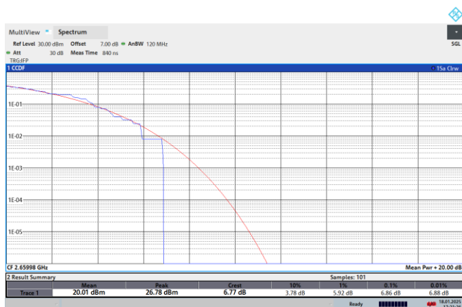
NTNV-N41-PC2-30-60-H-CP-16QPSK-Outer_Full-PASS
