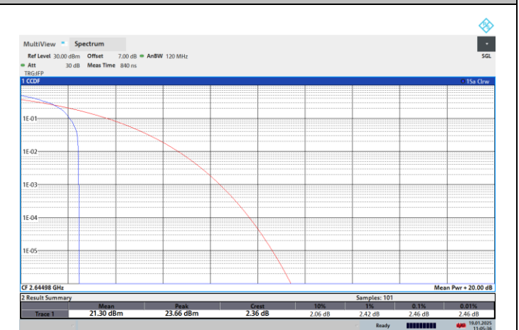
NTNV-N41-PC2-30-90-H-CP-QPSK-Edge_1RB_Left-PASS
