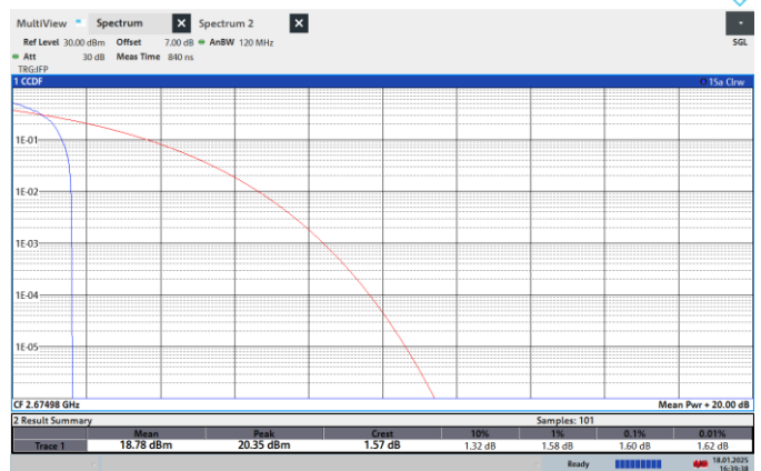
NTNV-N41-PC2-30-30-H-CP-256QPSK-Edge_1RB_Left-PASS
