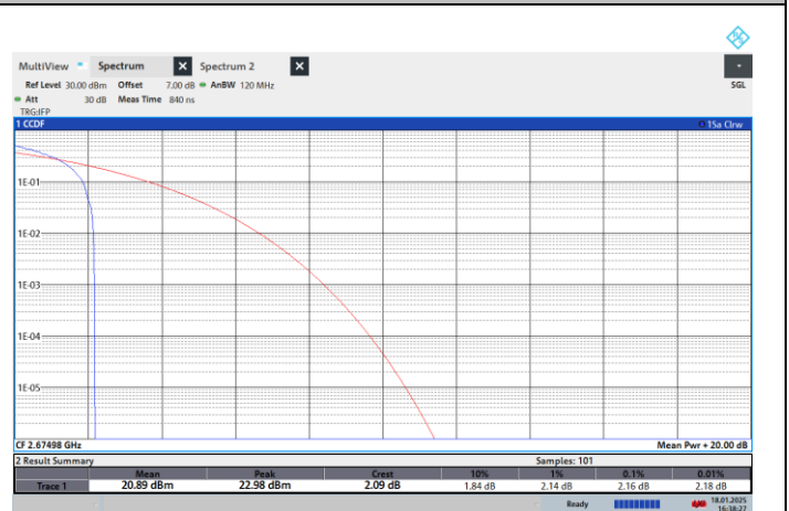
NTNV-N41-PC2-30-30-H-CP-16QPSK-Edge_1RB_Left-PASS
