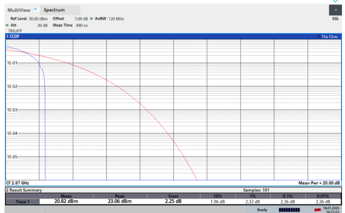
NTNV-N41-PC2-30-40-H-CP-QPSK-Edge_1RB_Left-PASS
