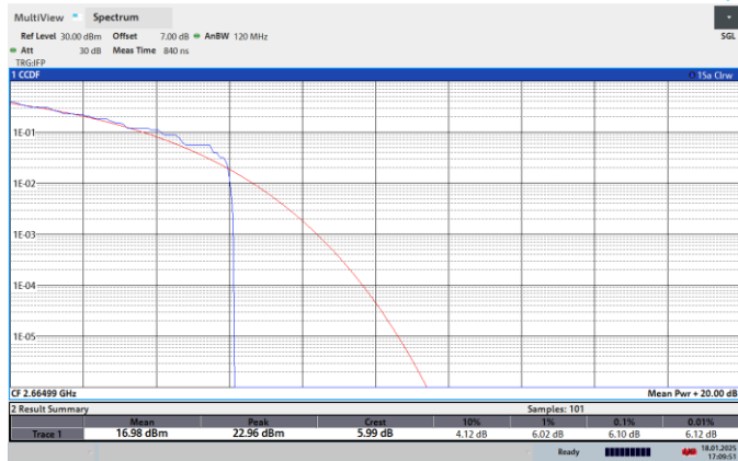
NTNV-N41-PC2-30-50-H-CP-256QPSK-Outer_Full-PASS
