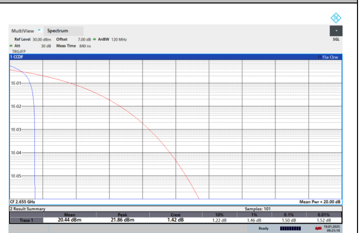
NTNV-N41-PC2-30-70-H-CP-QPSK-Edge_1RB_Left-PASS
