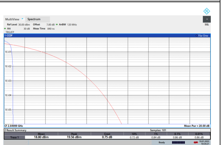
NTNV-N41-PC2-30-80-H-CP-16QPSK-Edge_1RB_Left-PASS
