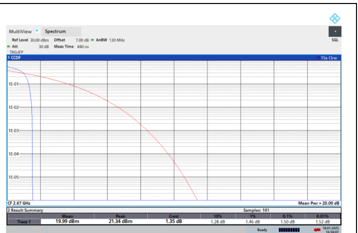
NTNV-N41-PC2-30-40-H-CP-16QPSK-Edge_1RB_Left-PASS
