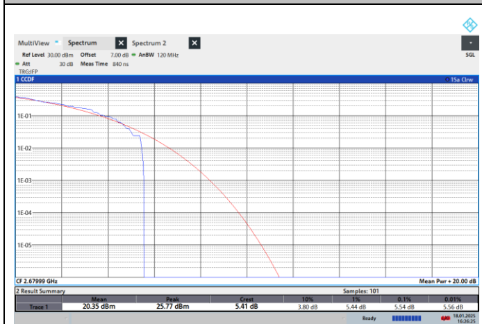
NTNV-N41-PC2-30-20-H-CP-16QPSK-Outer_Full-PASS
