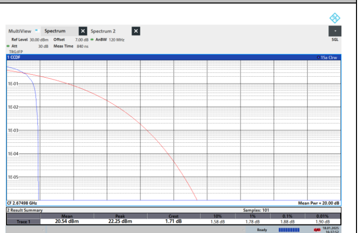
NTNV-N41-PC2-30-30-H-CP-QPSK-Edge_1RB_Left-PASS
