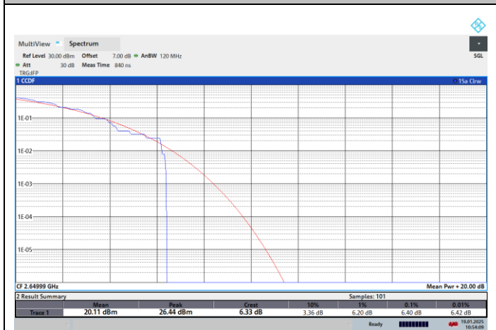
NTNV-N41-PC2-30-80-H-CP-16QPSK-Outer_Full-PASS
