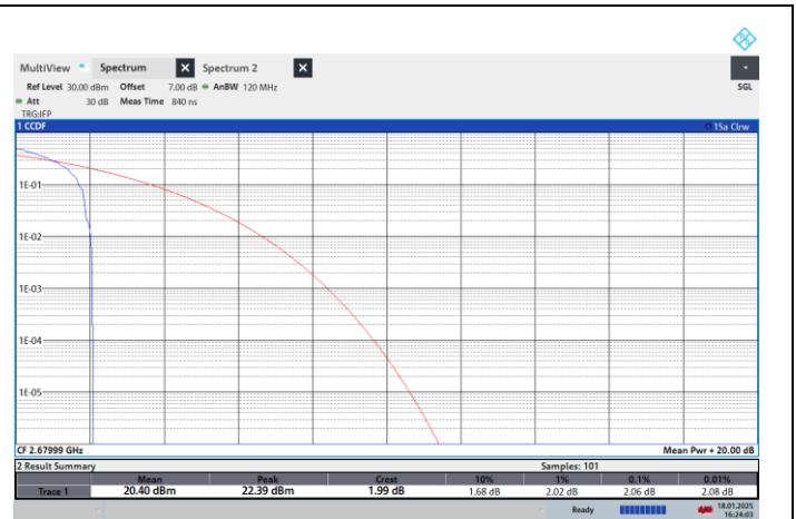
NTNV-N41-PC2-30-20-H-CP-QPSK-Edge_1RB_Left-PASS
