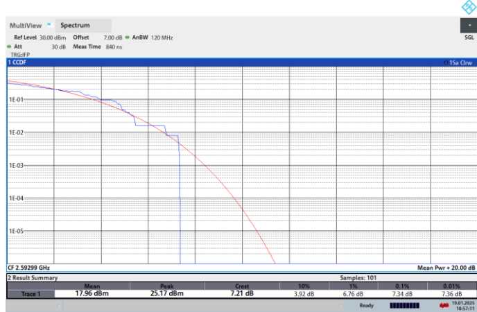
NTNV-N41-PC2-30-90-M-CP-64QPSK-Outer_Full-PASS
