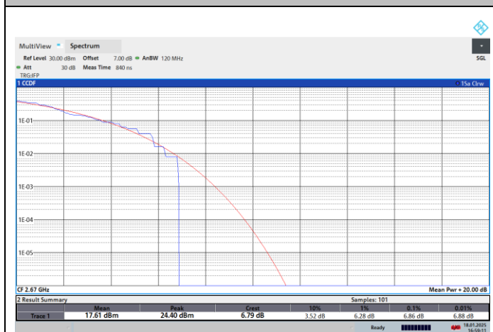
NTNV-N41-PC2-30-40-H-CP-256QPSK-Outer_Full-PASS
