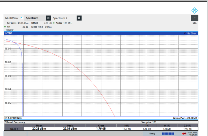
NTNV-N41-PC2-30-20-H-CP-16QPSK-Edge_1RB_Left-PASS
