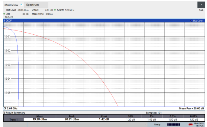
NTNV-N41-PC2-30-100-H-CP-16QPSK-Edge_1RB_Left-PASS
