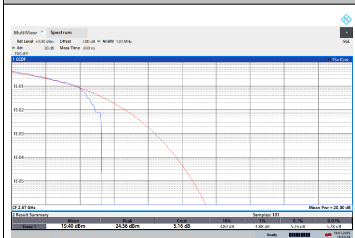
NTNV-N41-PC2-30-40-H-CP-64QPSK-Outer_Full-PASS
