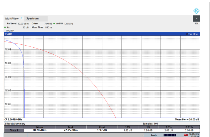
NTNV-N41-PC2-30-50-H-CP-QPSK-Edge_1RB_Left-PASS
