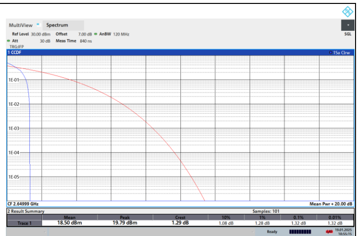
NTNV-N41-PC2-30-80-H-CP-256QPSK-Edge_1RB_Left-PASS
