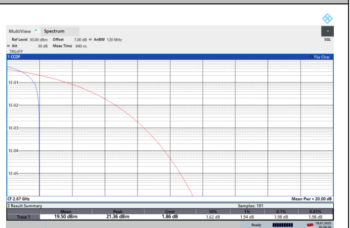
NTNV-N41-PC2-30-40-H-CP-64QPSK-Edge_1RB_Left-PASS
