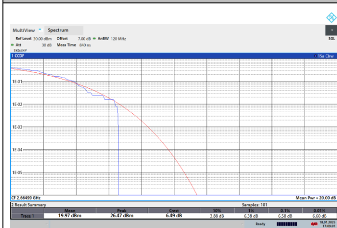
NTNV-N41-PC2-30-50-H-CP-16QPSK-Outer_Full-PASS
