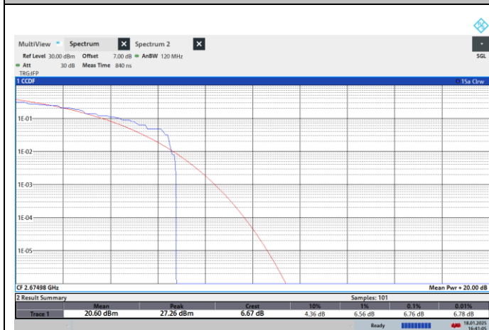
NTNV-N41-PC2-30-30-H-CP-QPSK-Outer_Full-PASS
