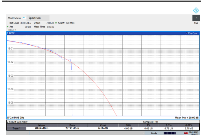
NTNV-N41-PC2-30-90-H-CP-QPSK-Outer_Full-PASS
