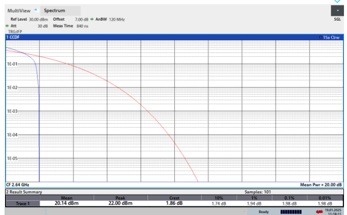
NTNV-N41-PC2-30-100-H-CP-64QPSK-Edge_1RB_Left-PASS
