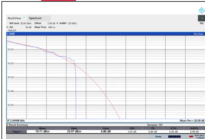
NTNV-N41-PC2-30-90-H-CP-64QPSK-Outer_Full-PASS
