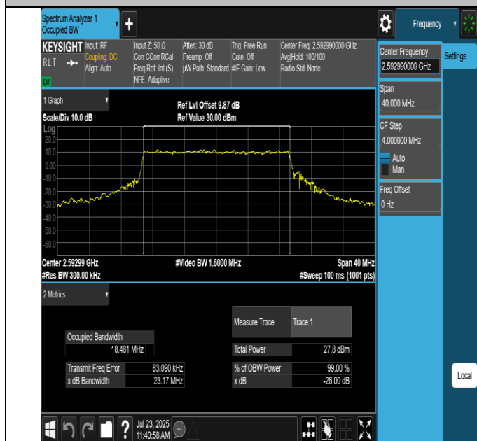
NTNV-n41-PC2-30-20-M-CP-64QAM-Outet_Full-Ant2-PASS
