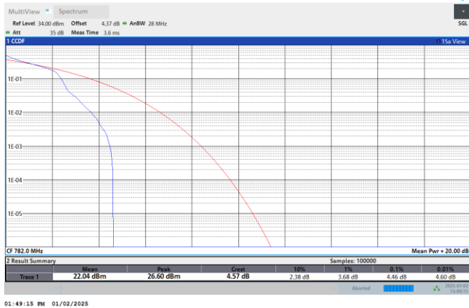
NTNV-N13-PC3-15-5-DFT-PI/2-BPSK-H- Edge_1RB_Left
