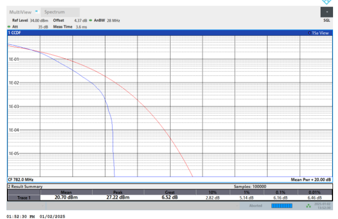
NTNV-N13-PC3-15-5-DFT-16QAM-H-Outer_Full
