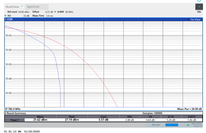
NTNV-N13-PC3-15-5-DFT-QPSK-H-Outer_Full
