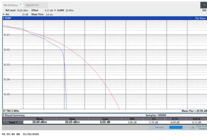
NTNV-N13-PC3-15-5-DFT-64QAM-L- Edge_1RB_Left
