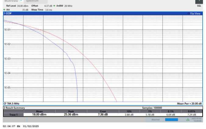
NTNV-N13-PC3-15-10-DFT-PI/2-BPSK-M-Edge_Outer_Full
