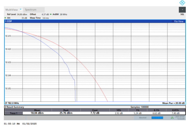
NTNV-N13-PC3-15-5-DFT-256QAM-H- Outer_Full
