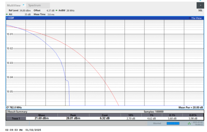
NTNV-N13-PC3-15-10-DFT-16QAM-M-Outer_Full
