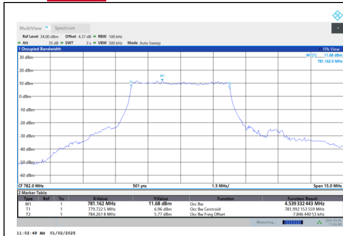
NTNV-N13-PC3-15-10-DFT-QPSK-M-Outer_Full
