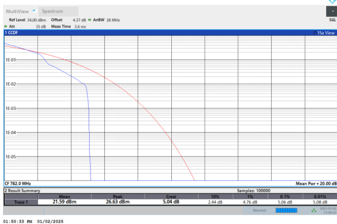
NTNV-N13-PC3-15-5-DFT-QPSK-H- Edge_1RB_Left
