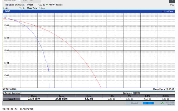
NTNV-N13-PC3-15-10-DFT-QPSK-M-Outer_Full
