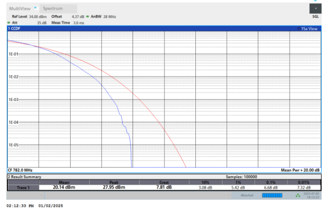
NTNV-N13-PC3-15-10-DFT-64QAM-M- Outer_Full
