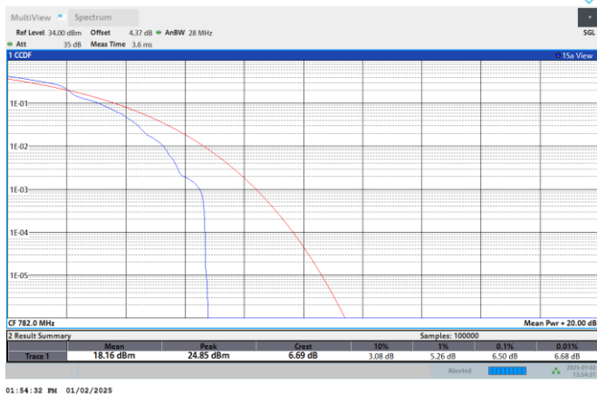
NTNV-N13-PC3-15-5-DFT-256QAM-H- Edge_1RB_Left
