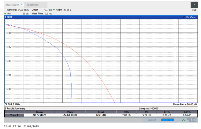
NTNV-N13-PC3-15-5-DFT-64QAM-L-Outer_Full
