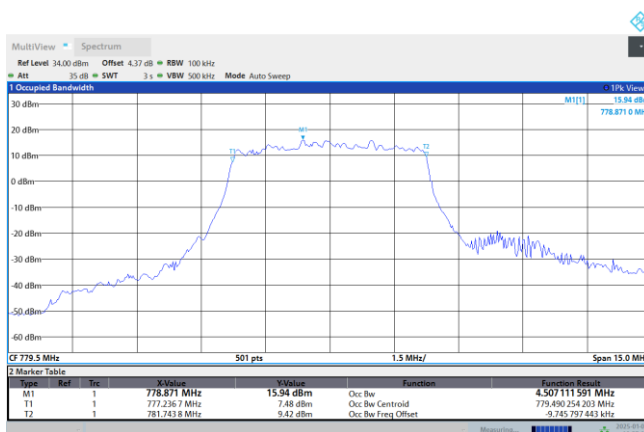
NTNV-N13-PC3-15-5-DFT-16QAM-L-Outer_Full
