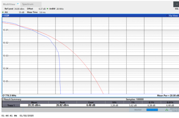
NTNV-N13-PC3-15-5-DFT-64QAM-M- Edge_1RB_Left
