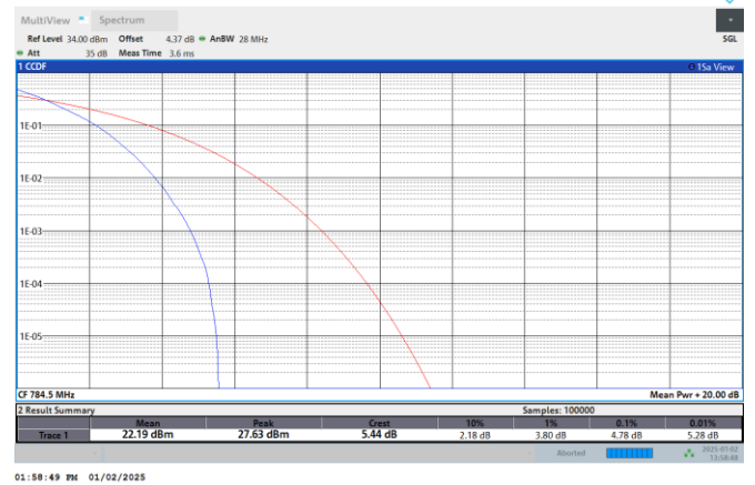
NTNV-N13-PC3-15-5-DFT-QPSK-L-Outer_Full
