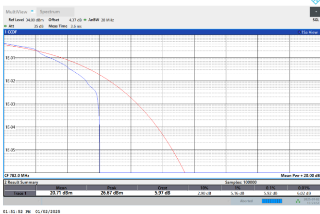
NTNV-N13-PC3-15-5-DFT-16QAM-H- Edge_1RB_Left
