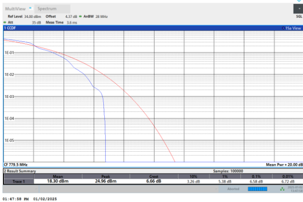
NTNV-N13-PC3-15-5-DFT-256QAM-M- Edge_1RB_Left
