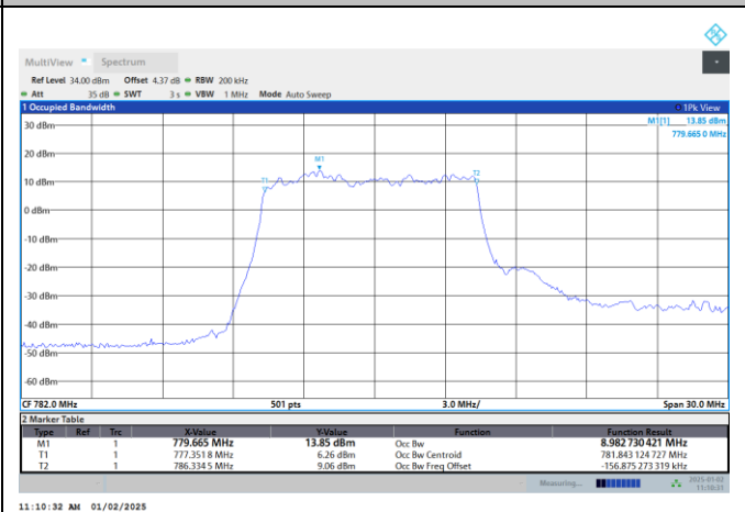
NTNV-N13-PC3-15-10-DFT-256QAM-M-Outer_Full
