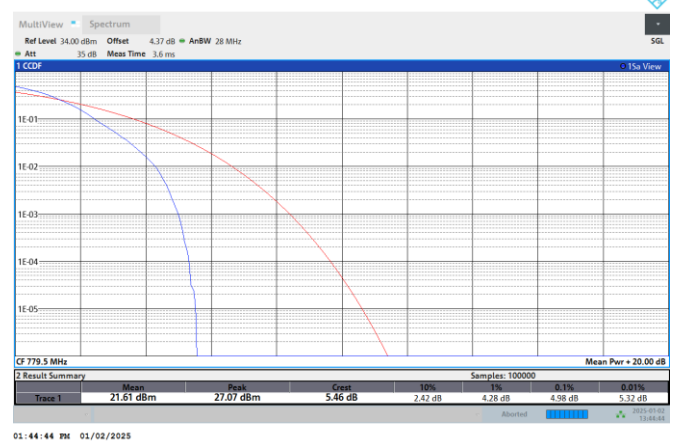
NTNV-N13-PC3-15-5-DFT-QPSK-M-Outer_Full
