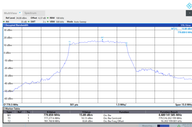
NTNV-N13-PC3-15-5-DFT-QPSK-L-Outer_Full
