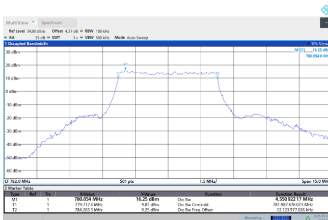
NTNV-N13-PC3-15-5-DFT-QPSK-M-Outer_Full
