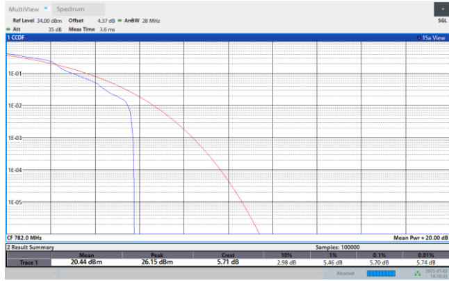
NTNV-N13-PC3-15-10-DFT-64QAM-M- Edge_1RB_Left
