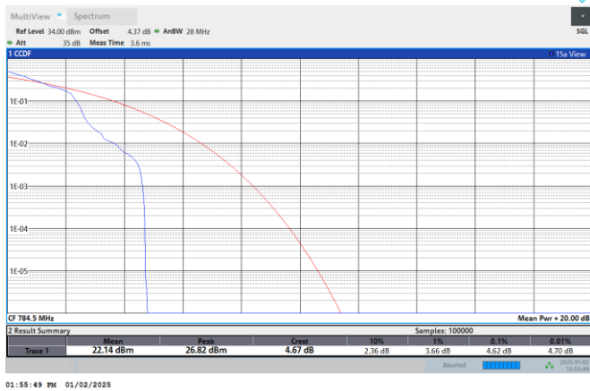
NTNV-N13-PC3-15-5-DFT-QPSK-L- Edge_1RB_Left
