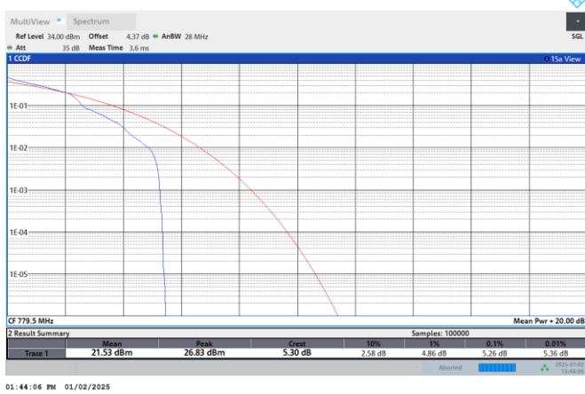
NTNV-N13-PC3-15-5-DFT-QPSK-M- Edge_1RB_Left
