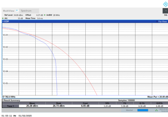
NTNV-N13-PC3-15-5-DFT-64QAM-H- Edge_1RB_Left
