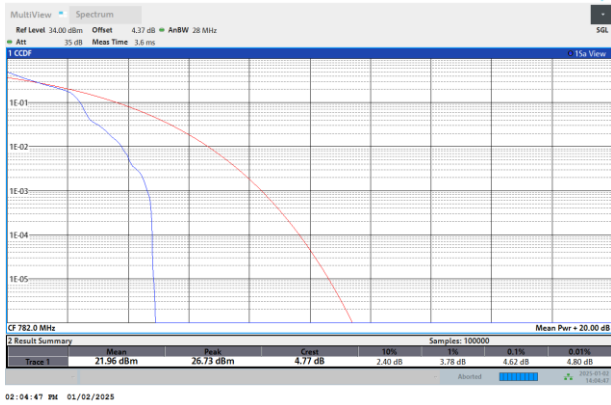
NTNV-N13-PC3-15-10-DFT-QPSK-M-Edge_1RB_Left
