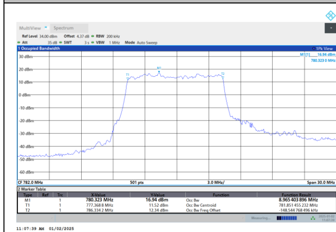
NTNV-N13-PC3-15-10-DFT-64QAM-M-Outer_Full
