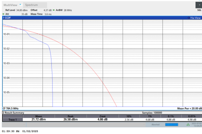
NTNV-N13-PC3-15-5-DFT-16QAM-L- Edge_1RB_Left
