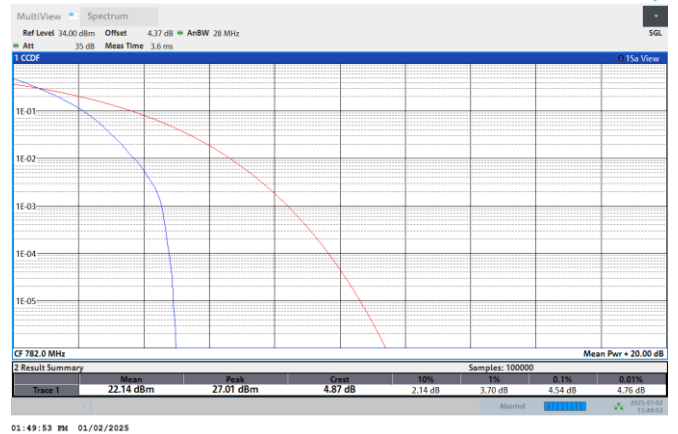
NTNV-N13-PC3-15-5-DFT-PI/2-BPSK-H- Edge_Outer_Full
