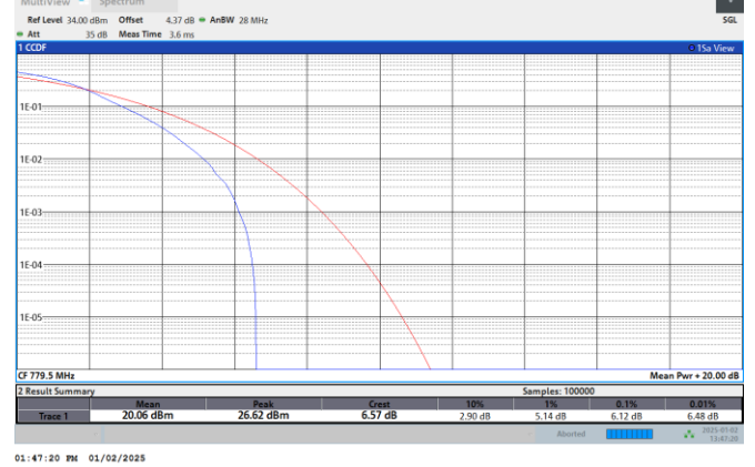
NTNV-N13-PC3-15-5-DFT-64QAM-M-Outer_Full
