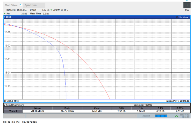
NTNV-N13-PC3-15-5-DFT-256QAM-L- Outer_Full
