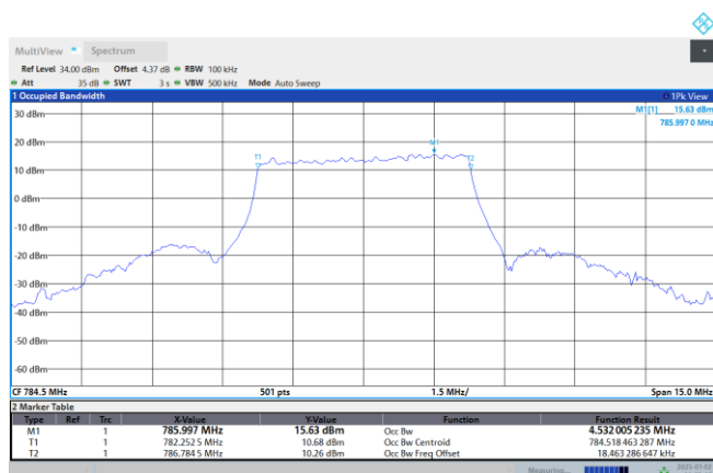
NTNV-N13-PC3-15-5-DFT-16QAM-M-Outer_Full
