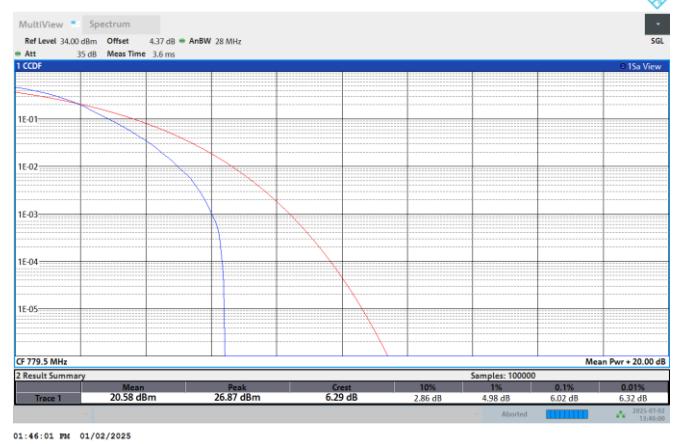
NTNV-N13-PC3-15-5-DFT-16QAM-M-Outer_Full
