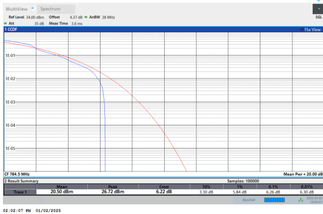
NTNV-N13-PC3-15-5-DFT-256QAM-L- Edge_1RB_Left
