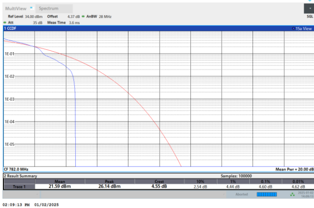
NTNV-N13-PC3-15-10-DFT-16QAM-M-Edge_1RB_Left
