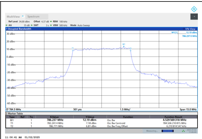
NTNV-N13-PC3-15-10-DFT-16QAM-M-Outer_Full
