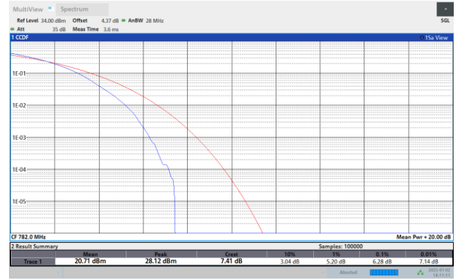
NTNV-N13-PC3-15-10-DFT-64QAM-M- Outer_Full
