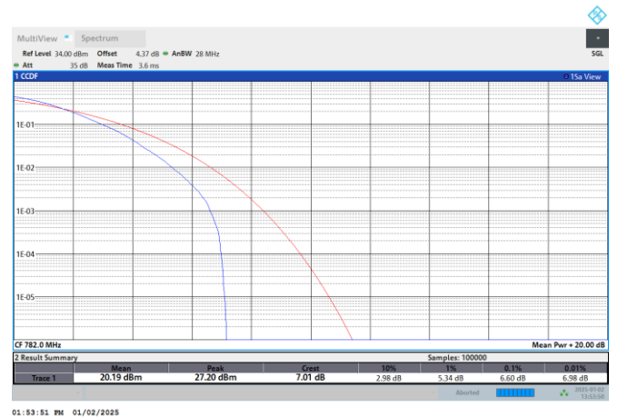
NTNV-N13-PC3-15-5-DFT-64QAM-H-Outer_Full
