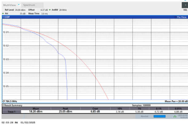
NTNV-N13-PC3-15-10-DFT-PI/2-BPSK-M-Edge_1RB_Left
