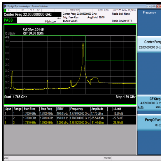
NTNV-N66-PC3-15-15-H-DFT-QPSK- Edge_1RB_Right-Ant1-PASS
