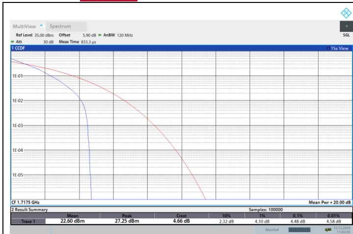
NTNV-N66-PC3-15-15-L-DFT-QPSK-Outer_Full-PASS
