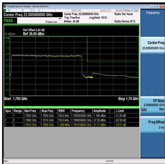
NTNV-N66-PC3-15-15-H-DFT-QPSK-Outer_Full- Ant1-PASS
