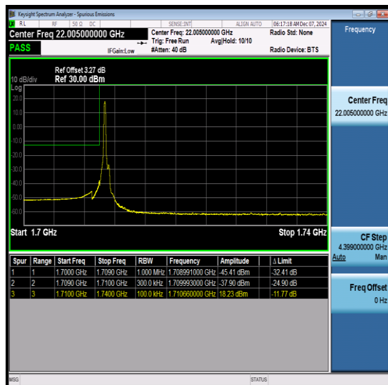
NTNV-N66-PC3-15-30-L-DFT-QPSK- Edge_1RB_Left-Ant1-PASS
