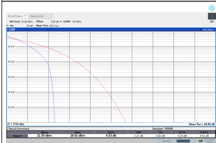
NTNV-N66-PC3-15-10-H-DFT-QPSK-Outer_Full-PASS
