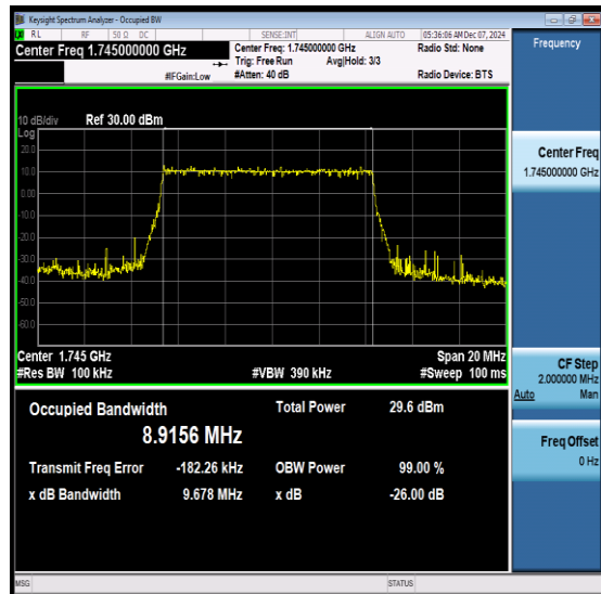
NTN-N66-PC3-15-10-M-DFT-PI2BPSK-Outer_Full-Ant1-PASS
