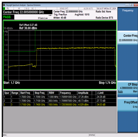
NTNV-N66-PC3-15-30-L-DFT-QPSK-Outer_Full- Ant1-PASS
