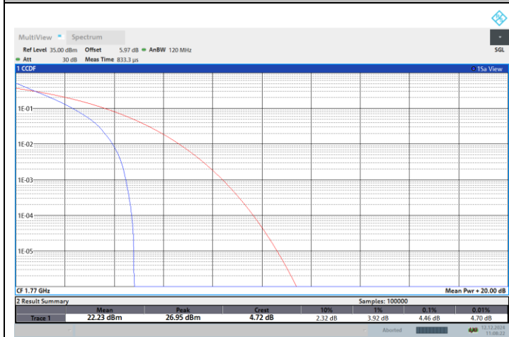
NTNV-N66-PC3-15-20-H-DFT-QPSK-Outer_Full-PASS
