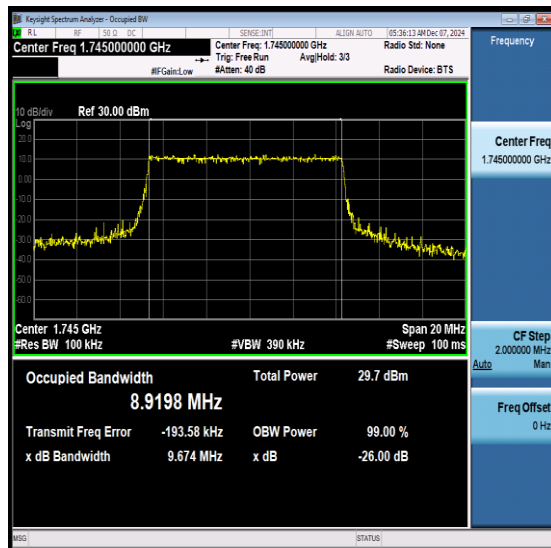
NTN-N66-PC3-15-10-M-DFT-QPSK-Outer_Full-Ant1-PASS
