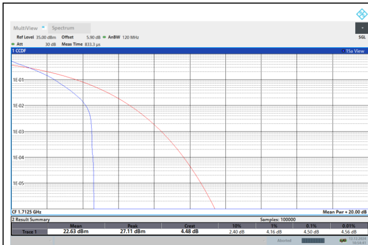
NTNV-N66-PC3-15-5-L-DFT-QPSK-Outer_Full-PASS
