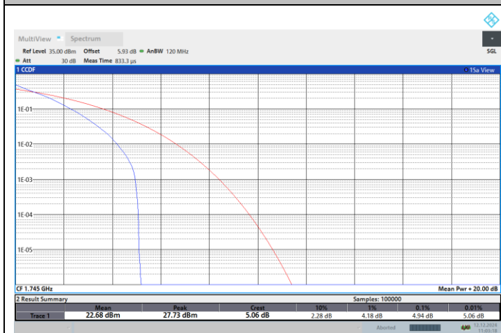
NTNV-N66-PC3-15-15-M-DFT-QPSK-Outer_Full-PASS
