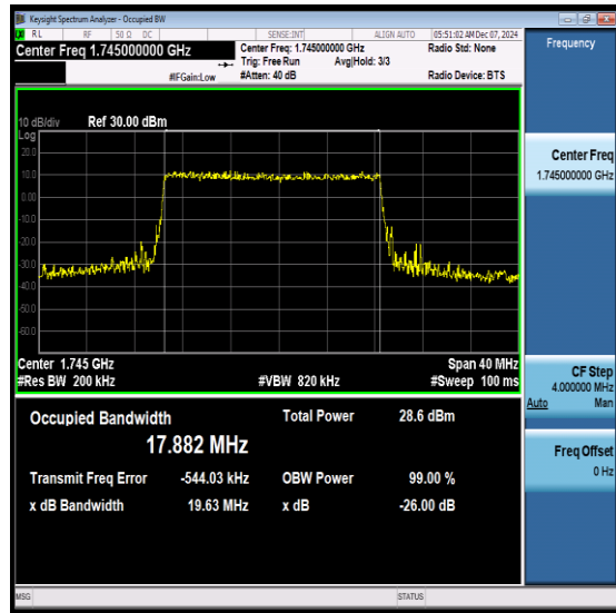
NTNV-N66-PC3-15-20-M-DFT-256QAM- Outer_Full-Ant1-PASS
