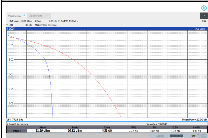
NTNV-N66-PC3-15-15-H-DFT-QPSK-Outer_Full-PASS
