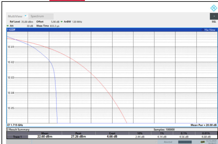
NTNV-N66-PC3-15-10-L-DFT-QPSK-Outer_Full-PASS
