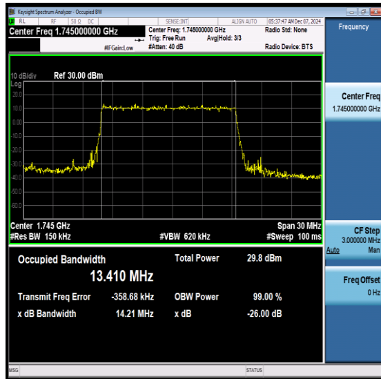
NTNV-N66-PC3-15-15-M-DFT-PI2BPSK-Outer_Full-Ant1-PASS
