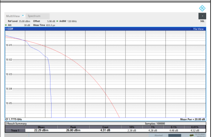
NTNV-N66-PC3-15-5-H-DFT-QPSK-Edge_1RB_Left-PASS
