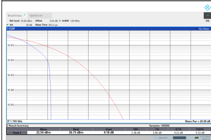
NTNV-N66-PC3-15-5-M-DFT-QPSK-Outer_Full-PASS
