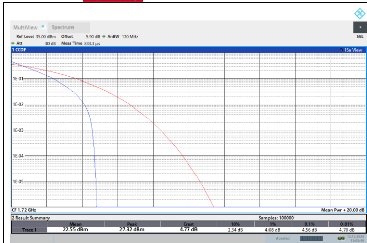
NTNV-N66-PC3-15-20-L-DFT-QPSK-Outer_Full-PASS
