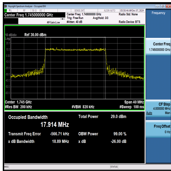
NTNV-N66-PC3-15-20-M-DFT-16QAM-Outer_Full- Ant1-PASS
