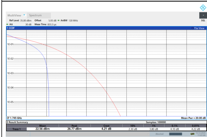
NTNV-N66-PC3-15-20-M-DFT-QPSK-Outer_Full-PASS
