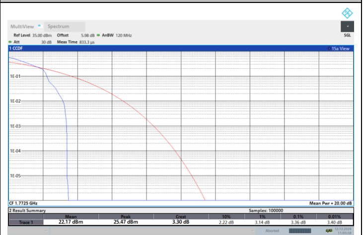
NTNV-N66-PC3-15-10-H-DFT-QPSK-Edge_1RB_Left-PASS
