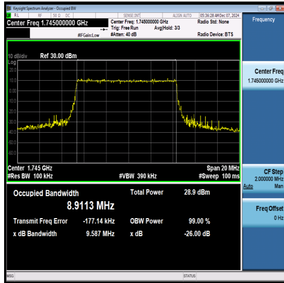
NTNV-N66-PC3-15-10-M-DFT-64QAM-Outer_Full-Ant1-PASS
