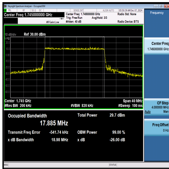
NTNV-N66-PC3-15-20-M-DFT-QPSK-Outer_Full- Ant1-PASS
