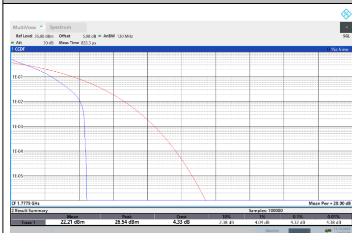
NTNV-N66-PC3-15-5-H-DFT-QPSK-Outer_Full-PASS
