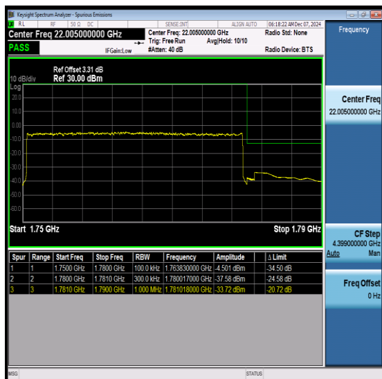
NTNV-N66-PC3-15-30-H-DFT-QPSK-Outer_Full- Ant1-PASS
