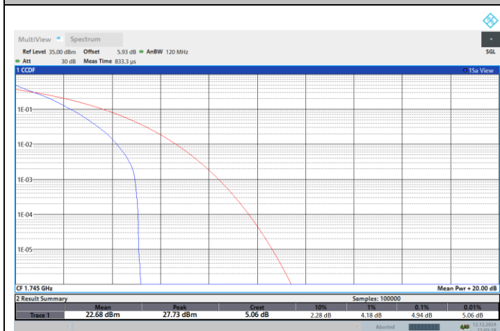
NTNV-N66-PC3-15-10-M-DFT-QPSK-Outer_Full-PASS
