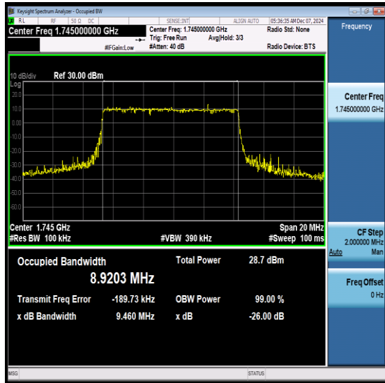
NTNV-N66-PC3-15-10-M-DFT-256QAM-Outer_Full-Ant1-PASS
