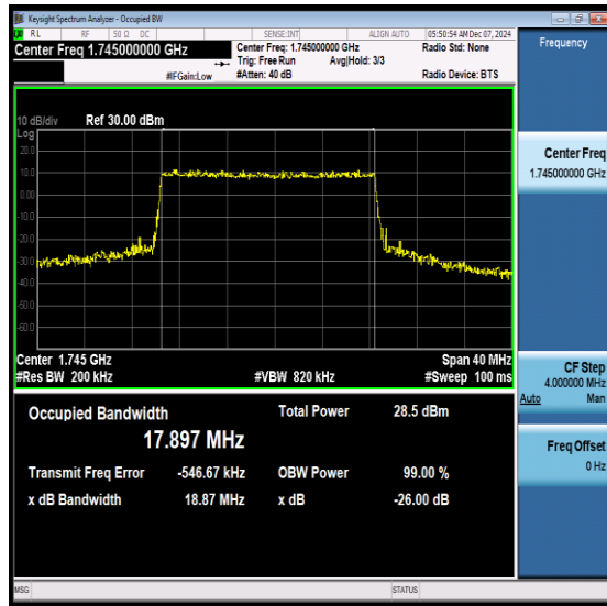
NTNV-N66-PC3-15-20-M-DFT-64QAM-Outer_Full- Ant1-PASS
