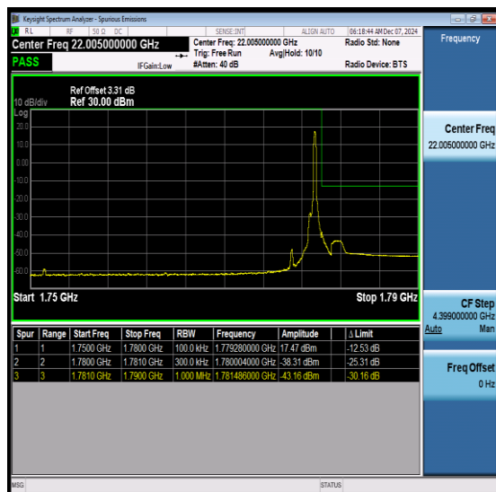
NTNV-N66-PC3-15-30-H-DFT-QPSK- Edge_1RB_Right-Ant1-PASS
