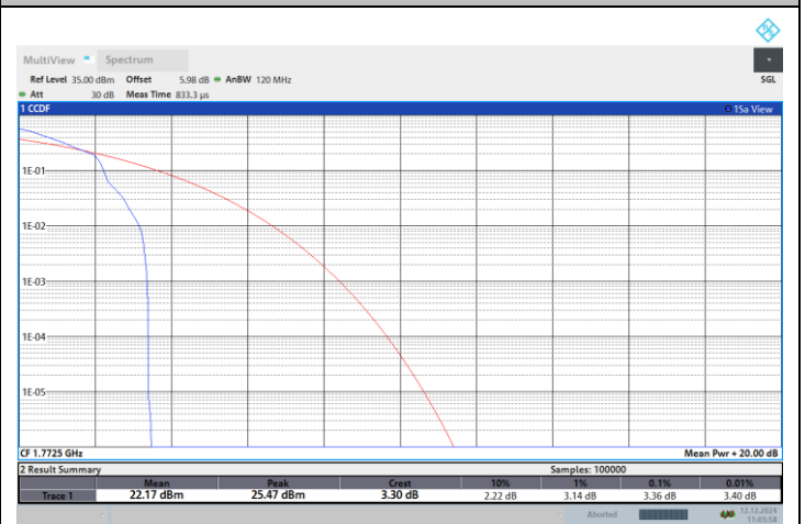
NTNV-N66-PC3-15-15-H-DFT-QPSK-Edge_1RB_Left-PASS
