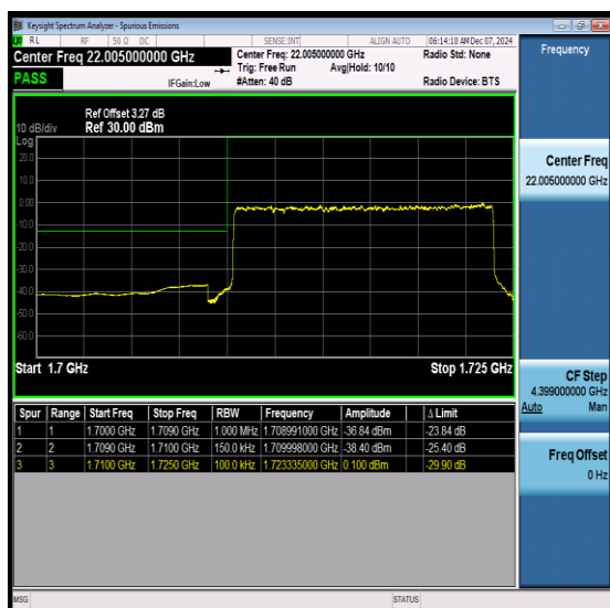
NTNV-N66-PC3-15-15-L-DFT-QPSK-Outer_Full- Ant1-PASS
