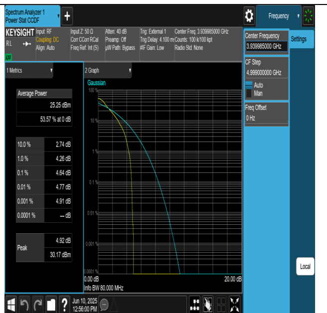
NTNV-N77-3700-3980-PC2-30-80-H-DFT-QPSK-Outer_Full- PASS
