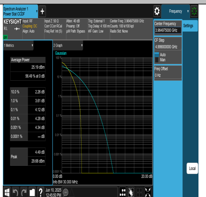
NTNV-N77-3700-3980-PC2-30-30-H-DFT-QPSK-Outer_Full-
