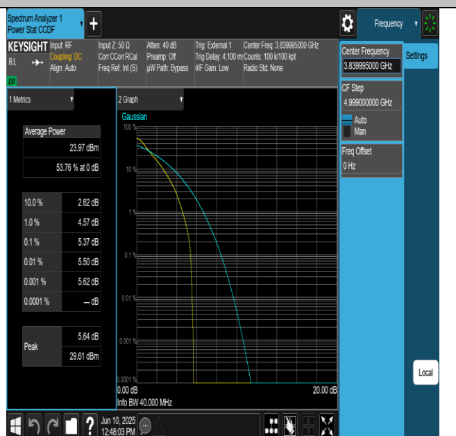
NTNV-N77-3700-3980-PC2-30-40-M-DFT-QPSK-Outer_Full- PASS
