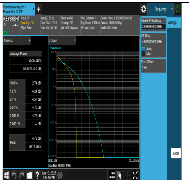
NTNV-N77-3700-3980-PC2-30-80-H-DFT-QPSK-Outer_Full- PASS
