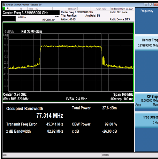
NTNV-N77-3700-3980-PC2-30-80-M-CP-QPSK- Outer_Full-Ant1-PASS
