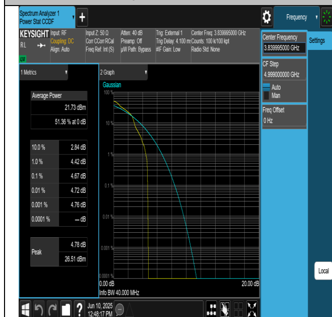
NTNV-N77-3700-3980-PC2-30-40-M-DFT-QPSK- Edge_1RB_Left-PASS
