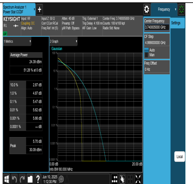
NTNV-N77-3700-3980-PC2-30-80-L-DFT-QPSK-Outer_Full- PASS
