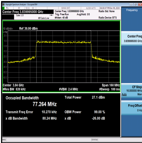
NTNV-N77-3700-3980-PC2-30-80-M-CP-64QAM- Outer_Full-Ant1-PASS
