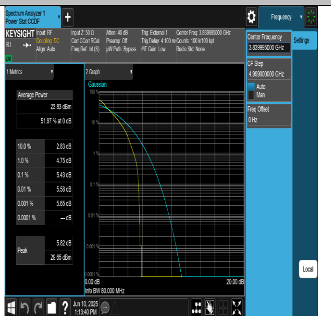
NTNV-N77-3700-3980-PC2-30-80-M-DFT-QPSK-Outer_Full- PASS
