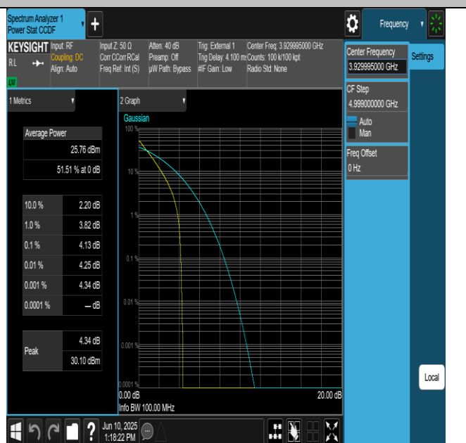
NTNV-N77-3700-3980-PC2-30-100-H-DFT-QPSK-Outer_Full-
