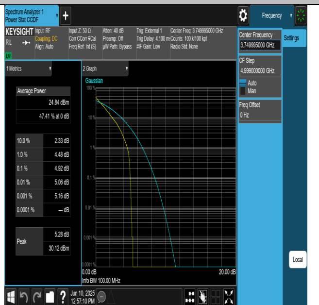
NTNV-N77-3700-3980-PC2-30-100-L-DFT-QPSK-Outer_Full- PASS
