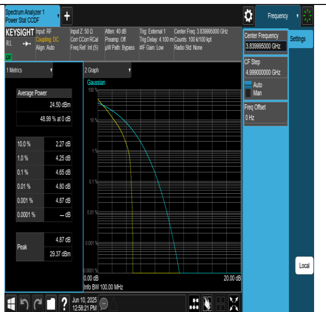
NTNV-N77-3700-3980-PC2-30-100-M-DFT-QPSK-Outer_Full-PASS
