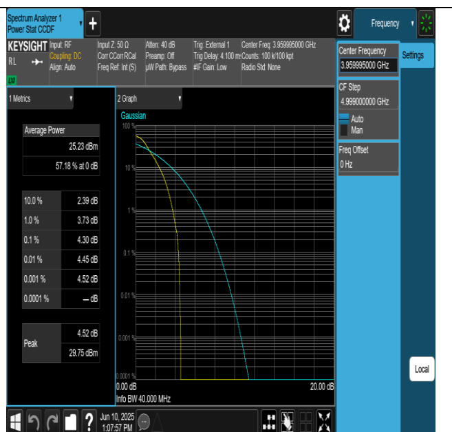
NTNV-N77-3700-3980-PC2-30-40-H-DFT-QPSK-Outer_Full- PASS
