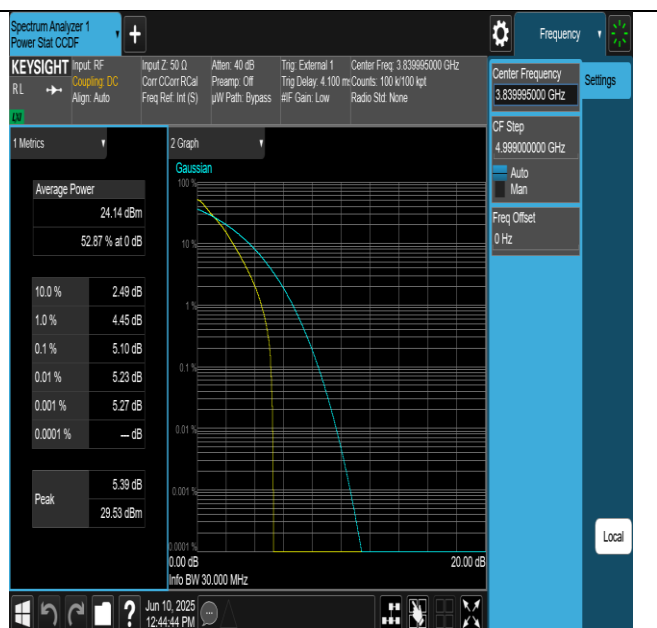
NTNV-N77-3700-3980-PC2-30-30-M-DFT-QPSK-Outer_Full-
