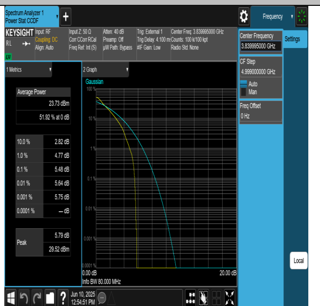
NTNV-N77-3700-3980-PC2-30-80-M-DFT-QPSK-Outer_Full- PASS
