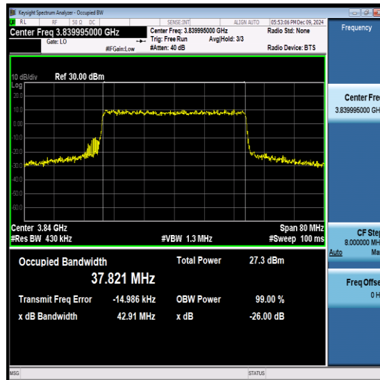
NTNV-N77-3700-3980-PC2-30-40-M-CP-16QAM- Outer_Full-Ant1-PASS
