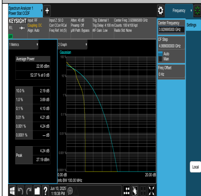
NTNV-N77-3700-3980-PC2-30-100-H-DFT-QPSK-
