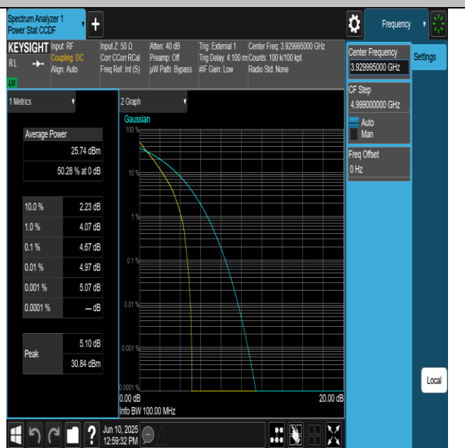
NTNV-N77-3700-3980-PC2-30-100-H-DFT-QPSK-Outer_Full-PASS
