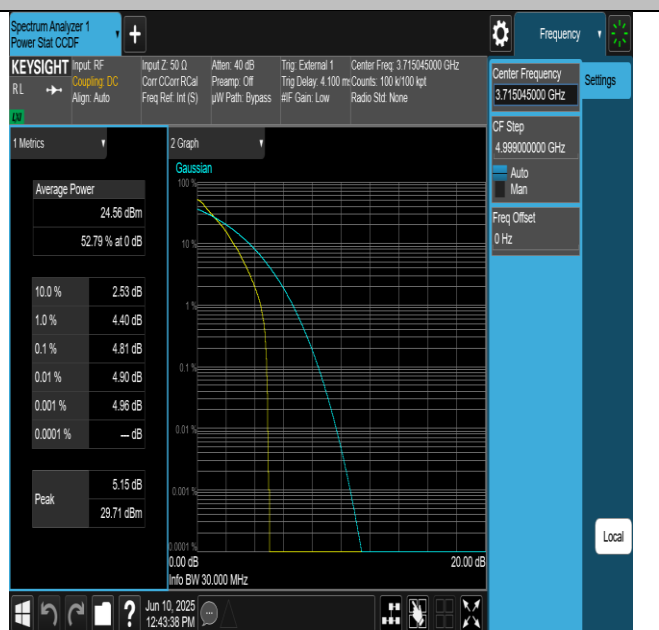
NTNV-N77-3700-3980-PC2-30-30-L-DFT-QPSK-Outer_Full- PASS
