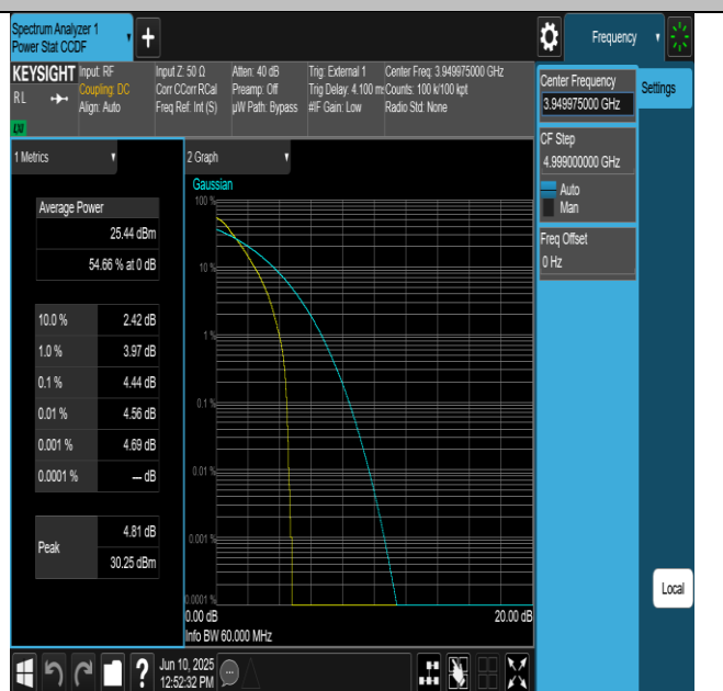
NTNV-N77-3700-3980-PC2-30-60-H-DFT-QPSK-Outer_Full-
