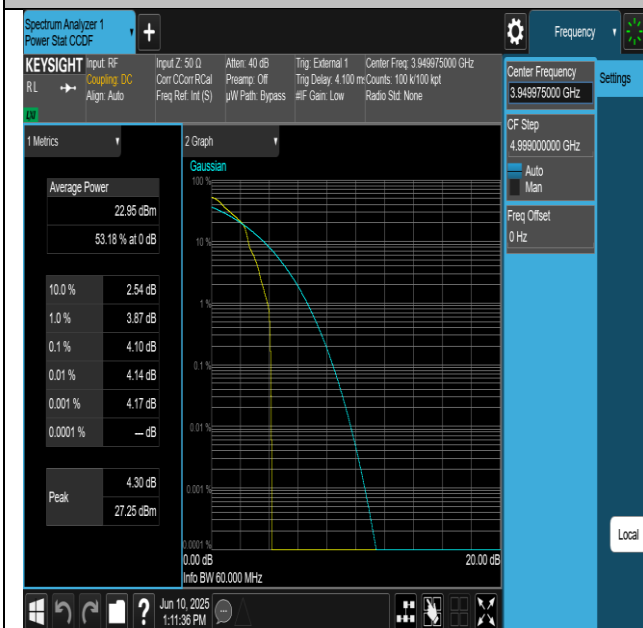
NTNV-N77-3700-3980-PC2-30-60-H-DFT-QPSK- Edge_1RB_Left-PASS
