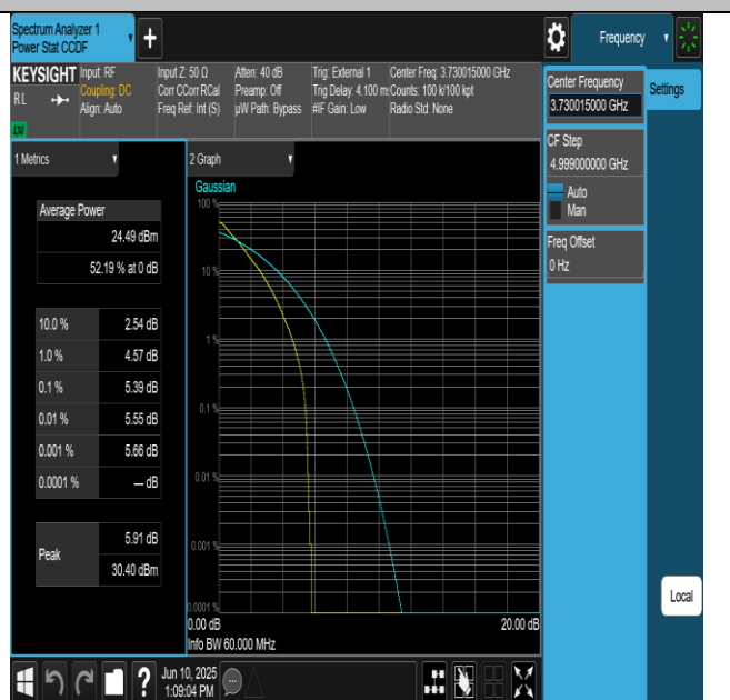
NTNV-N77-3700-3980-PC2-30-60-L-DFT-QPSK-Outer_Full- PASS
