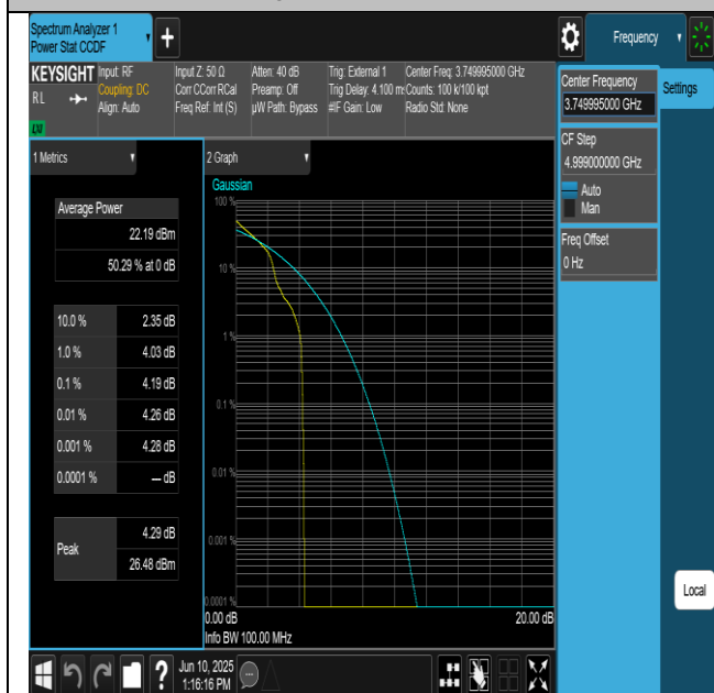
NTNV-N77-3700-3980-PC2-30-100-L-DFT-QPSK- Edge_1RB_Left-PASS
