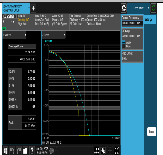
NTNV-N77-3700-3980-PC2-30-20-M-DFT-QPSK-Outer_Full-
