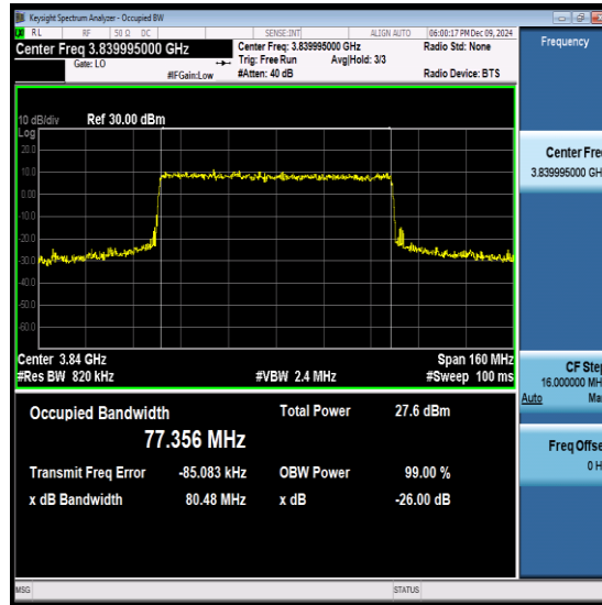
NTNV-N77-3700-3980-PC2-30-80-M-CP-16QAM- Outer_Full-Ant1-PASS
