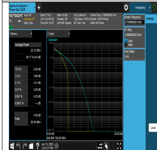
NTNV-N77-3700-3980-PC2-30-100-L-DFT-QPSK- Edge_1RB_Left-PASS
