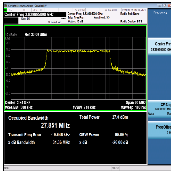
NTNV-N77-3700-3980-PC2-30-30-M-CP-16QAM- Outer_Full-Ant1-PASS
