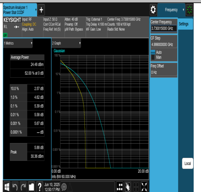
NTNV-N77-3700-3980-PC2-30-60-L-DFT-QPSK-Outer_Full- PASS
