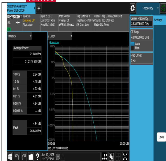
NTNV-N77-3700-3980-PC2-30-100-M-DFT-QPSK-
