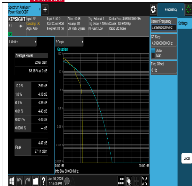
NTNV-N77-3700-3980-PC2-30-80-H-DFT-QPSK- Edge_1RB_Left-PASS
