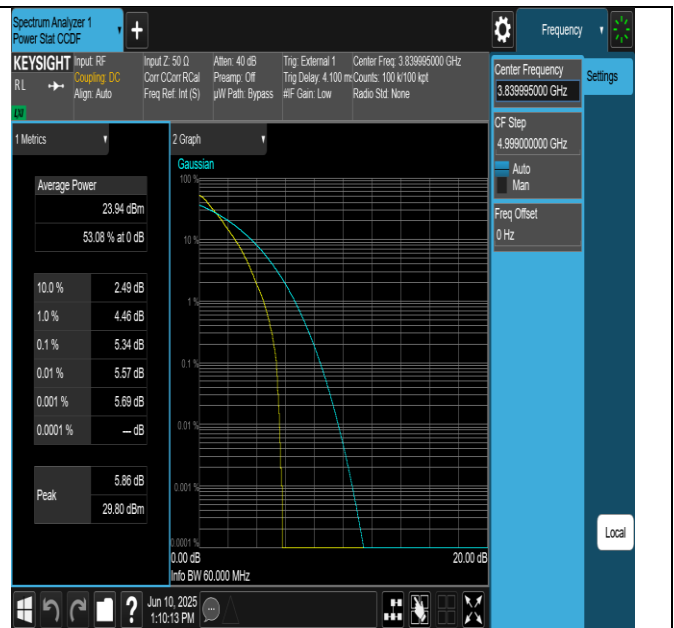
NTNV-N77-3700-3980-PC2-30-60-M-DFT-QPSK-Outer_Full- PASS
