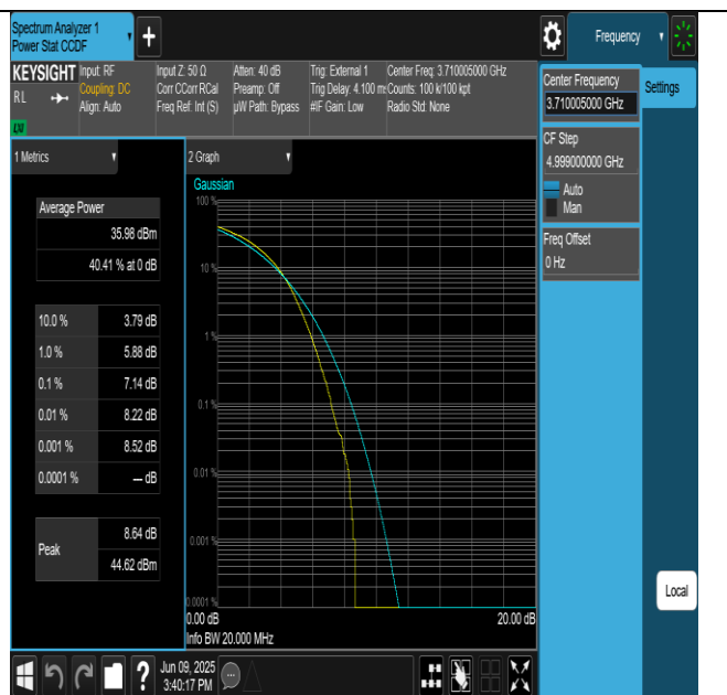
NTNV-N77-3700-3980-PC2-30-20-L-DFT-QPSK-Outer_Full-
