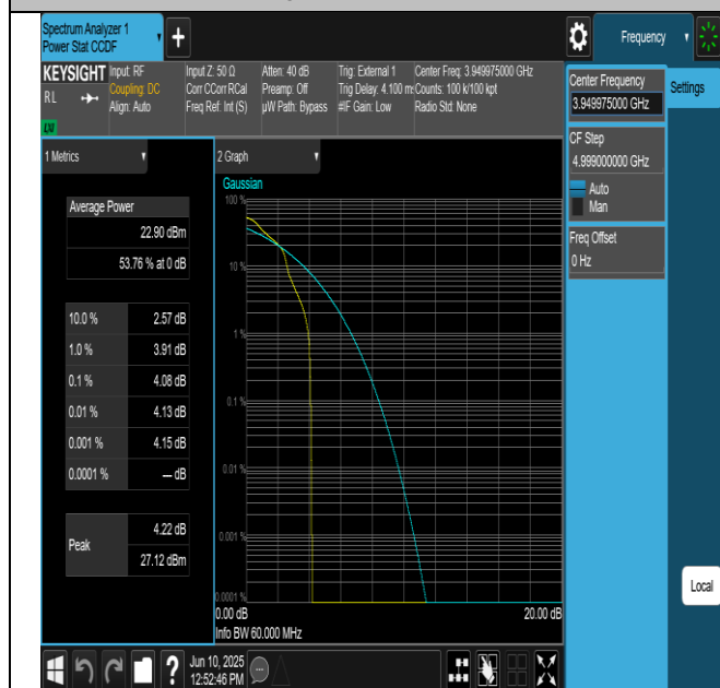
NTNV-N77-3700-3980-PC2-30-60-H-DFT-QPSK-
