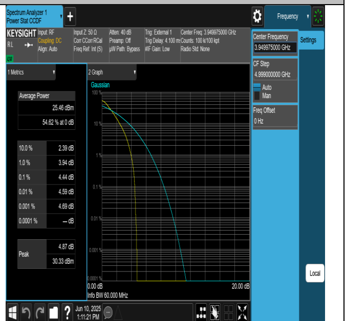
NTNV-N77-3700-3980-PC2-30-60-H-DFT-QPSK-Outer_Full- PASS
