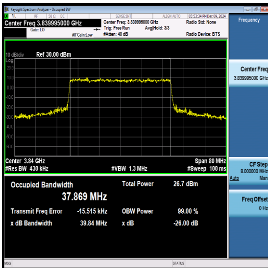
NTNV-N77-3700-3980-PC2-30-40-M-CP-64QAM- Outer_Full-Ant1-PASS
