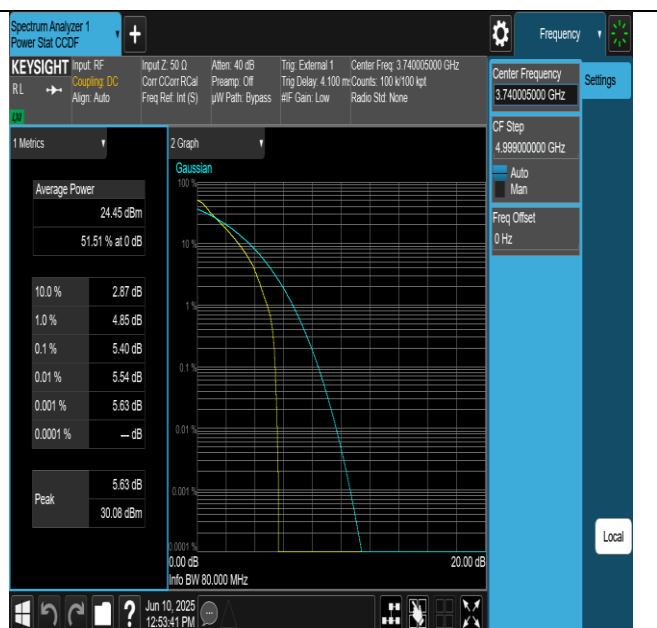
NTNV-N77-3700-3980-PC2-30-80-L-DFT-QPSK-Outer_Full- PASS
