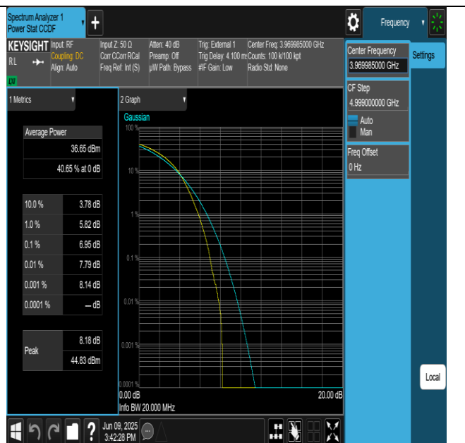
NTNV-N77-3700-3980-PC2-30-20-H-DFT-QPSK-Outer_Full- PASS
