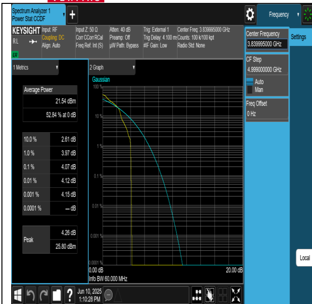
NTNV-N77-3700-3980-PC2-30-60-M-DFT-QPSK- Edge_1RB_Left-PASS
