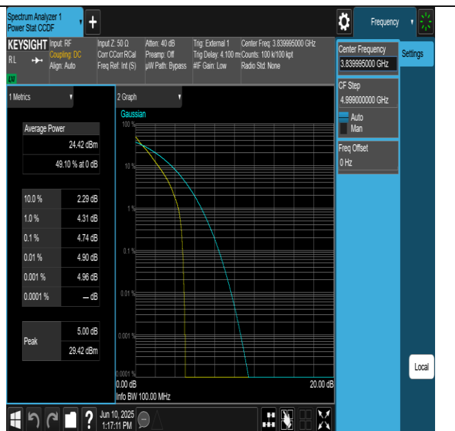
NTNV-N77-3700-3980-PC2-30-100-M-DFT-QPSK-Outer_Full-
