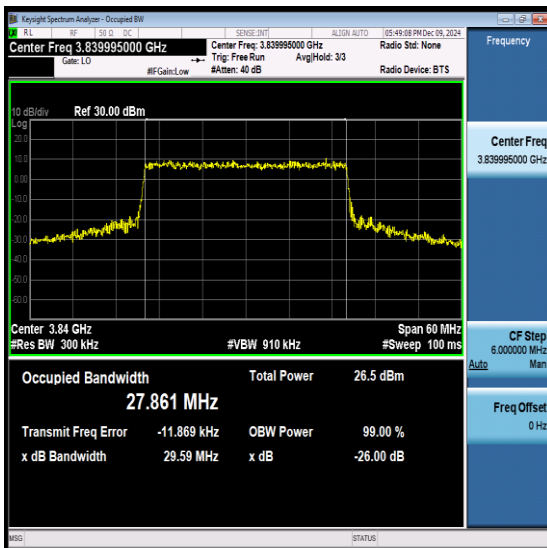
NTNV-N77-3700-3980-PC2-30-30-M-CP-64QAM- Outer_Full-Ant1-PASS
