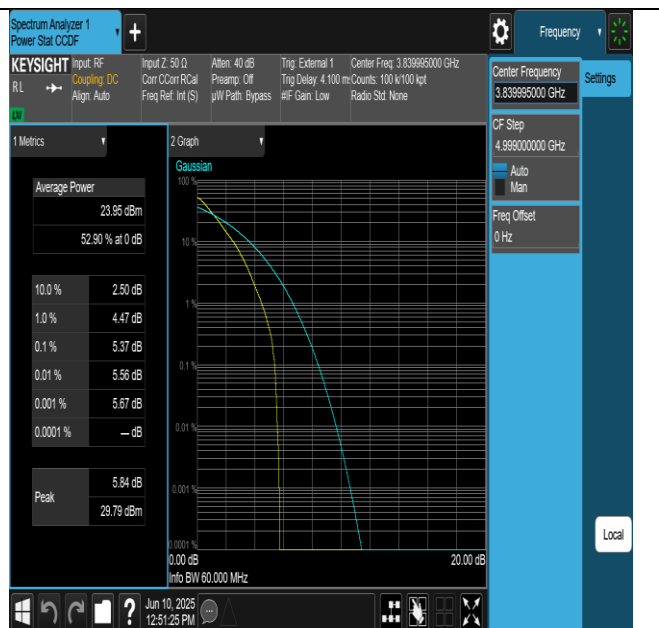
NTNV-N77-3700-3980-PC2-30-60-M-DFT-QPSK-Outer_Full-
