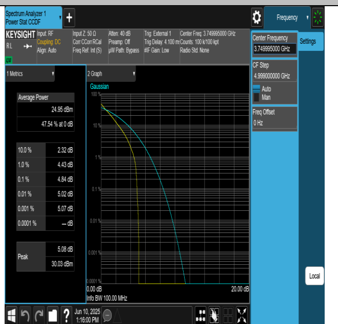
NTNV-N77-3700-3980-PC2-30-100-L-DFT-QPSK-Outer_Full- PASS
