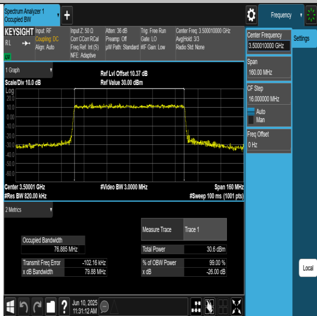
NTNV-N77-3450-3550-PC2-30-80-M-DFT-16QAM-Outer_Full- Ant1-PASS
