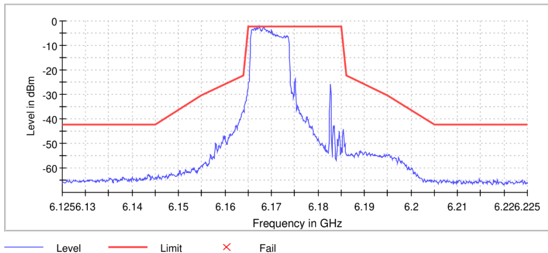
11AX20MIMO Ant8 6175 RU106/53
