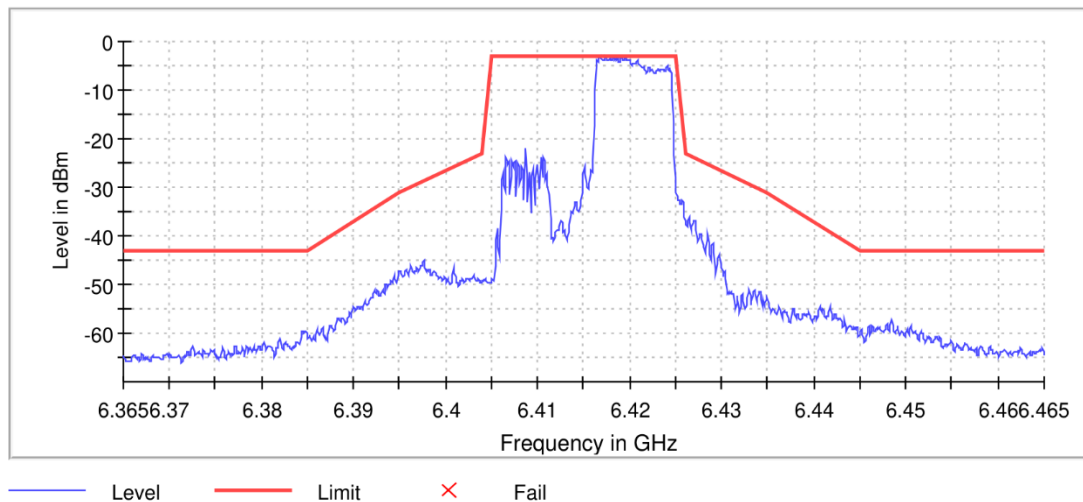
11AX20MIMO Ant8 6415 RU106/54
