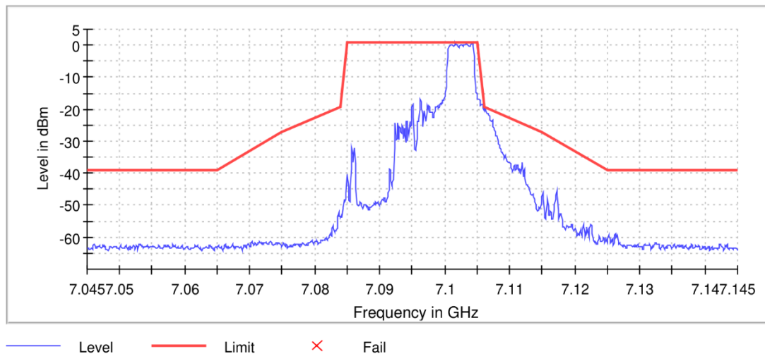
11AX20MIMO Ant8 7095 RU52/40
