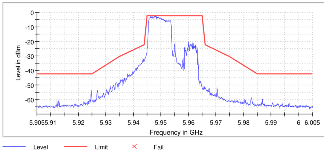
11AX20MIMO Ant8 5955 RU106/53
