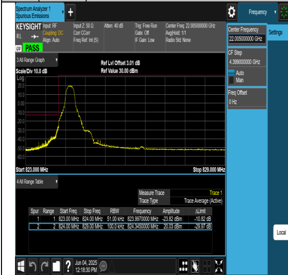
26(824-849)-5MHz-64QAM-27015-1RB#24-PASS
