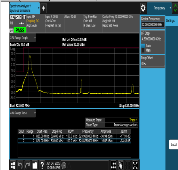
26(824-849)-15MHz-256QAM-26965-1RB#74-PASS
