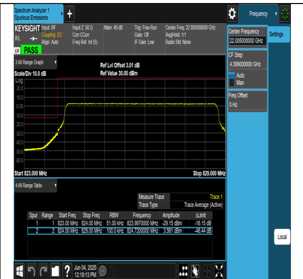
26(824-849)-5MHz-256QAM-27015-25RB#0-PASS
