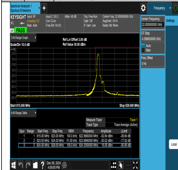
26(824-849)-5MHz-16QAM-27015-1RB#24-PASS
