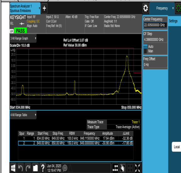
26(824-849)-15MHz-16QAM-26865-1RB#0-PASS
