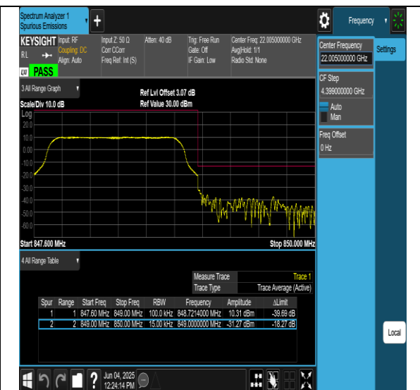
26(824-849)-1.4MHz-16QAM-26797-6RB#0-PASS
