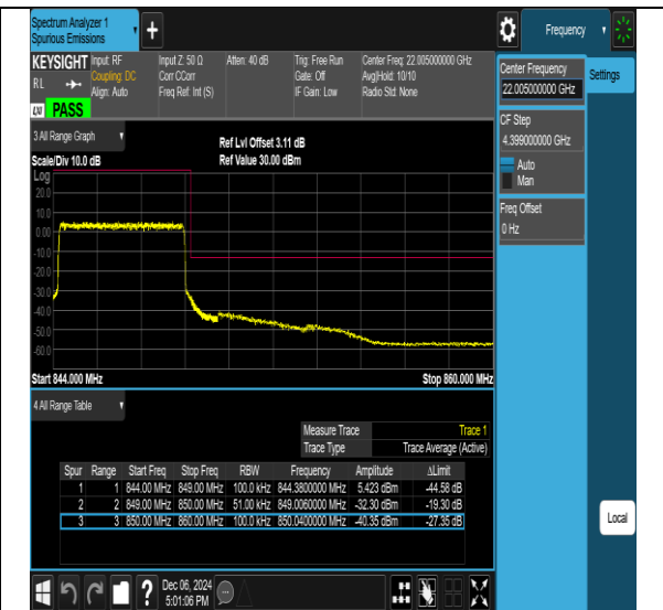
26(824-849)-5MHz-64QAM-26815-25RB#0-PASS
