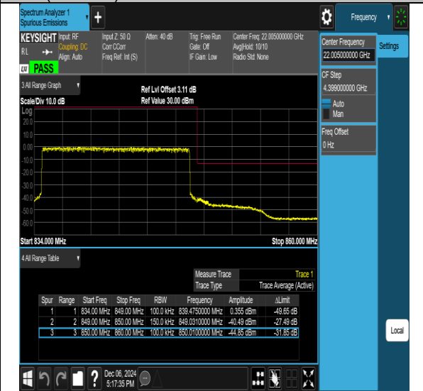
26(824-849)-15MHz-64QAM-26865-75RB#0-PASS
