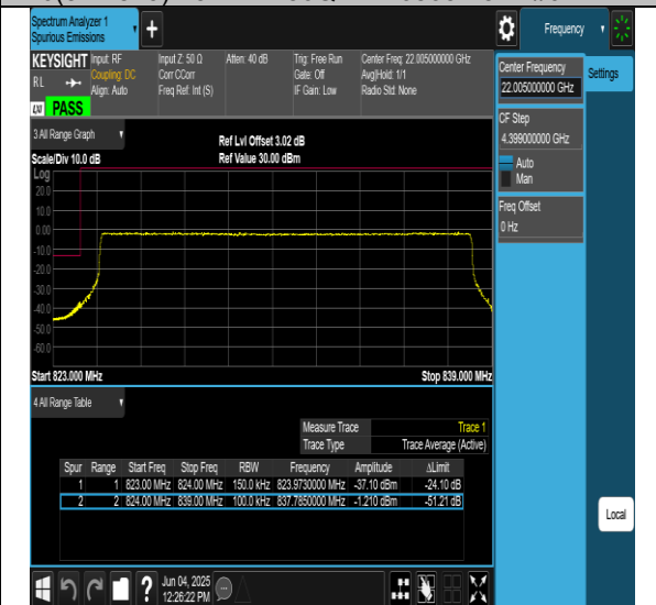
26(824-849)-15MHz-256QAM-26965-75RB#0-PASS
