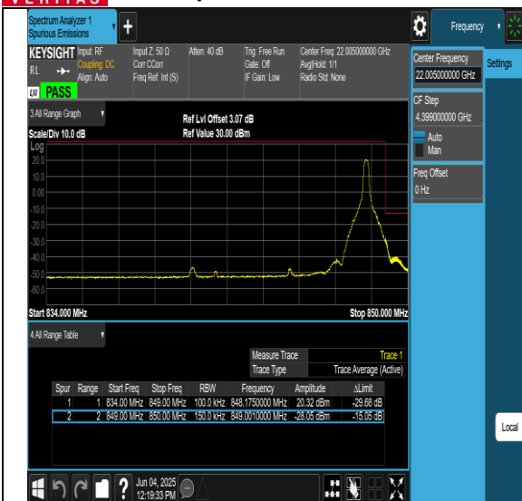
26(824-849)-15MHz-256QAM-26865-1RB#0-PASS
