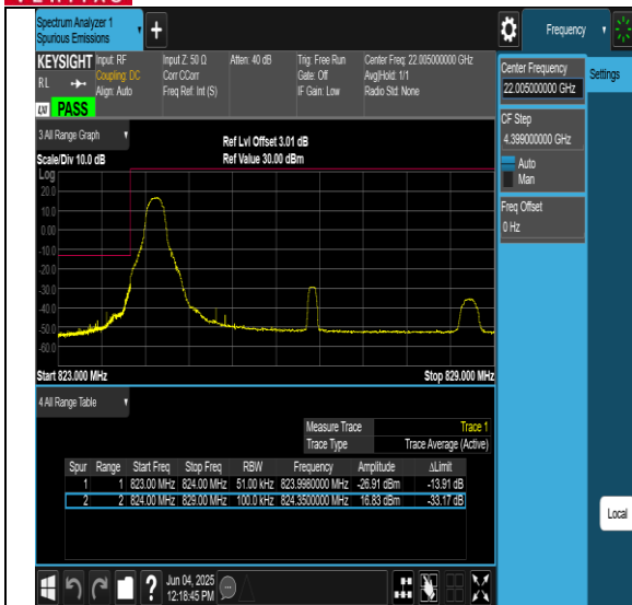
26(824-849)-5MHz-256QAM-27015-1RB#24-PASS
