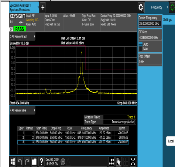
26(824-849)-15MHz-64QAM-26865-1RB#0-PASS
