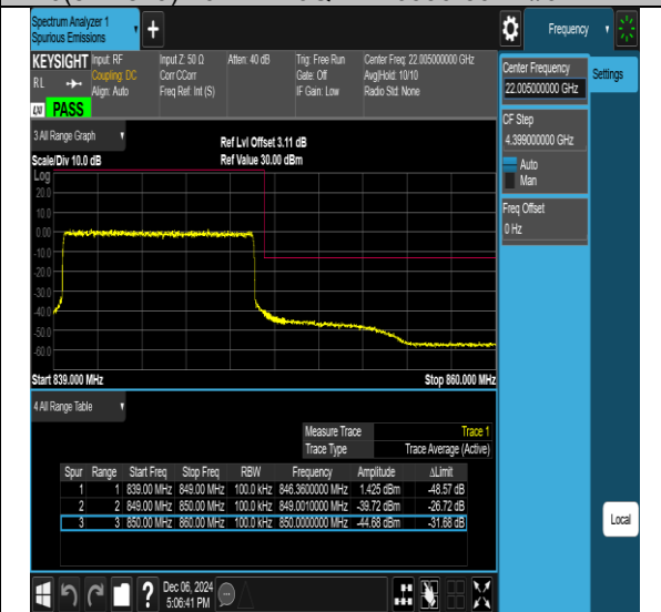
26(824-849)-15MHz-QPSK-26865-75RB#0-PASS
