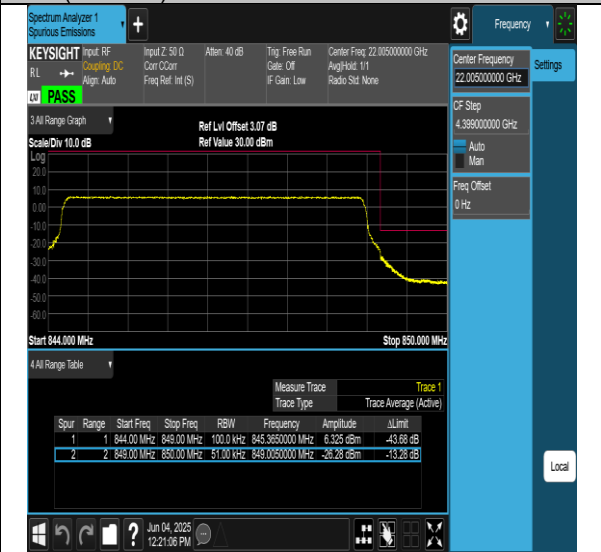
26(824-849)-5MHz-256QAM-26815-25RB#0-PASS
