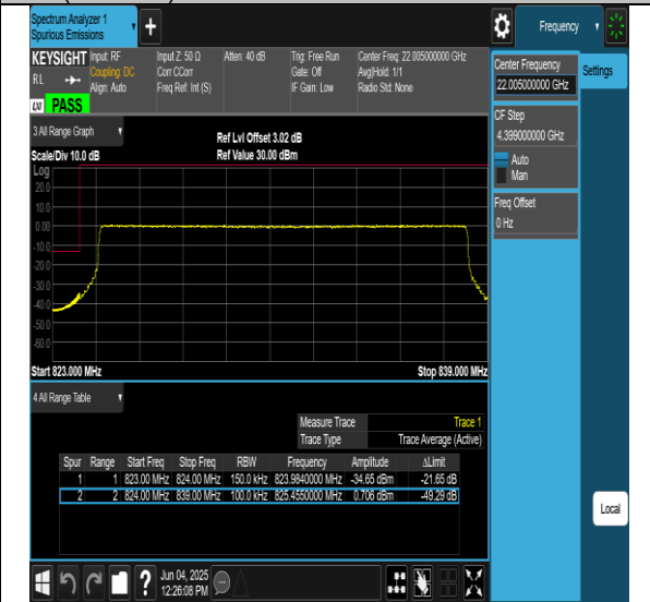
26(824-849)-15MHz-64QAM-26965-75RB#0-PASS
