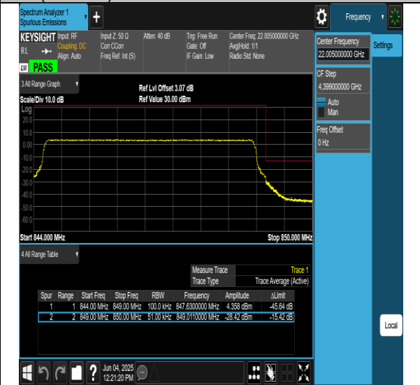
26(824-849)-5MHz-16QAM-26815-25RB#0-PASS
