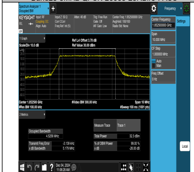
Band25-5MHz-QPSK-26065-25RB#0-PASS
