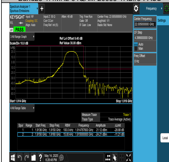
Band25-1.4MHz-256QAM-26047-1RB#0-PASS
