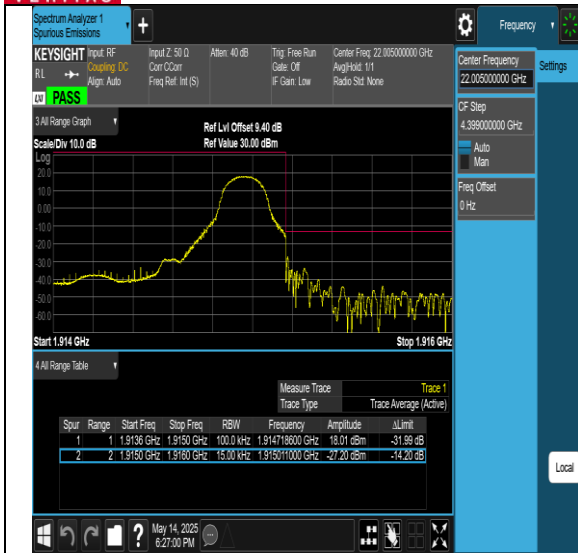
Band25-1.4MHz-16QAM-26047-1RB#0-PASS
