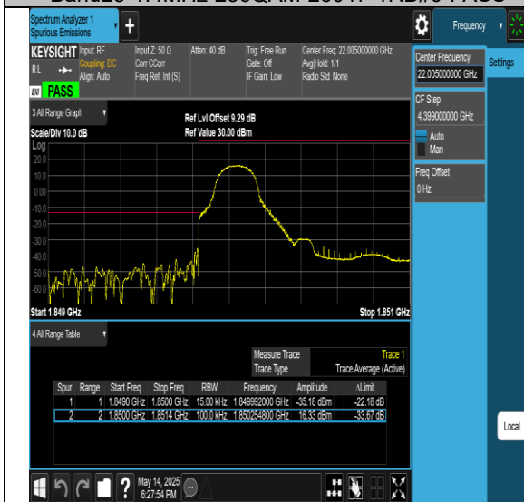
Band25-1.4MHz-256QAM-26683-1RB#5-PASS
