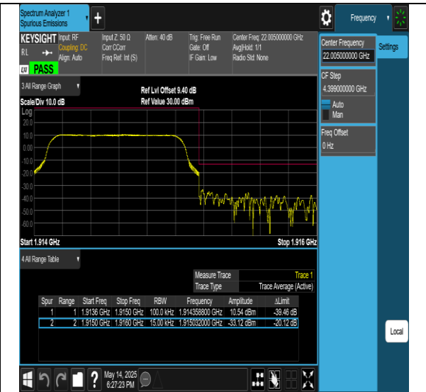
Band25-1.4MHz-16QAM-26047-6RB#0-PASS
