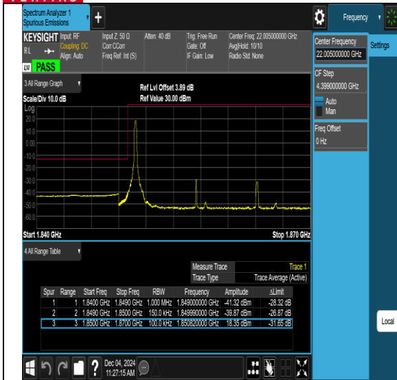
Band25-15MHz-16QAM-26615-1RB#74-PASS
