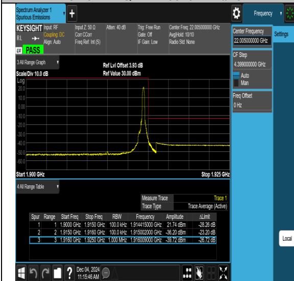
Band25-10MHz-64QAM-26090-1RB#0-PASS
