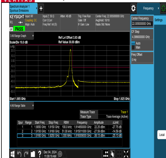
Band25-5MHz-64QAM-26065-1RB#0-PASS
