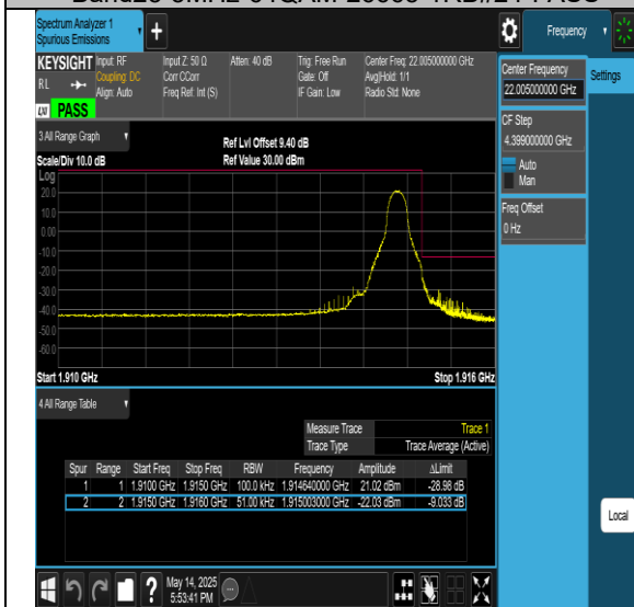
Band25-5MHz-256QAM-26065-1RB#0-PASS
