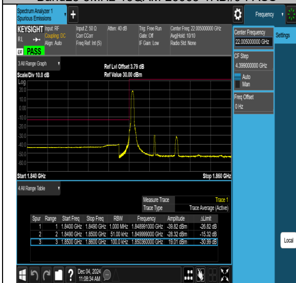
Band25-5MHz-16QAM-26665-1RB#24-PASS
