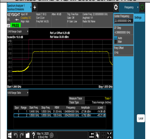
Band25-5MHz-64QAM-26665-25RB#0-PASS
