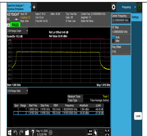
Band25-15MHz-256QAM-26115-75RB#0-PASS
