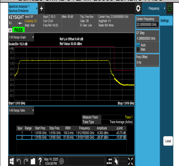
Band25-5MHz-256QAM-26065-25RB#0-PASS
