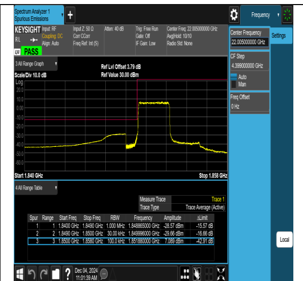
Band25-3MHz-QPSK-26675-15RB#0-PASS
