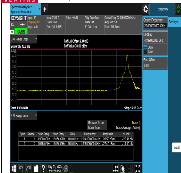
Band25-15MHz-256QAM-26115-1RB#0-PASS
