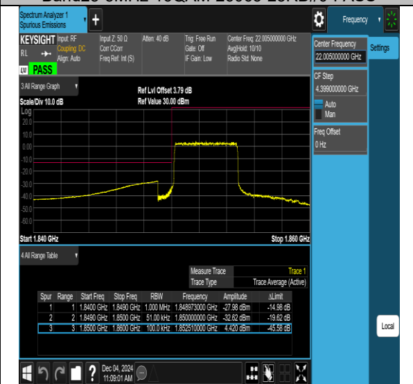
Band25-5MHz-16QAM-26665-25RB#0-PASS
