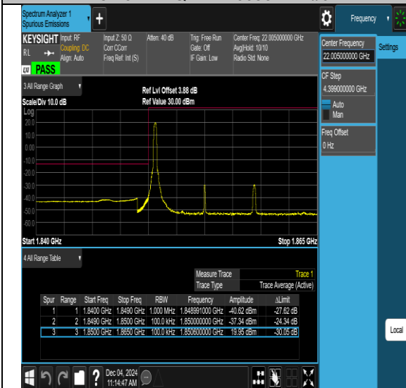
Band25-10MHz-QPSK-26640-1RB#49-PASS
