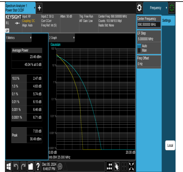
Band71-15MHz-64QAM-133197-75RB#0-PASS
