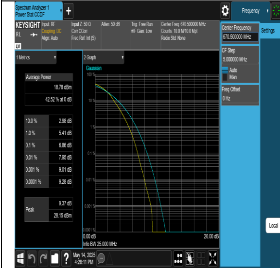
Band71-15MHz-256QAM-133297-1RB#0-PASS
