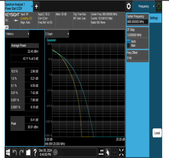
Band71-10MHz-16QAM-133297-50RB#0-PASS
