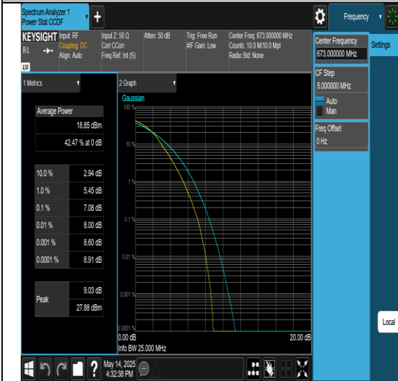
Band71-20MHz-256QAM-133322-1RB#0-PASS
