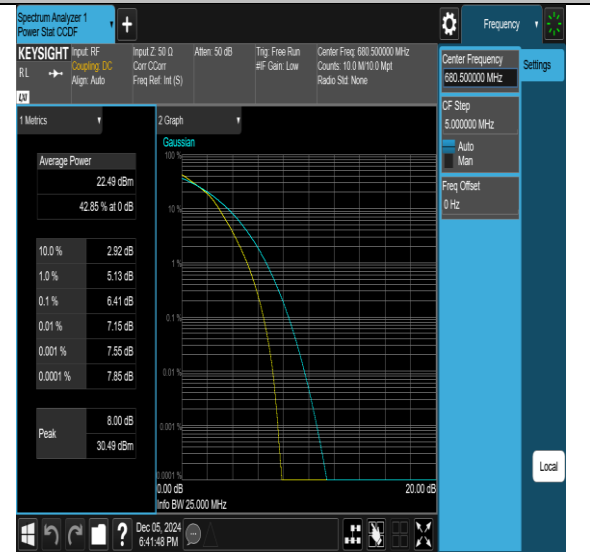
Band71-10MHz-16QAM-133422-50RB#0-PASS
