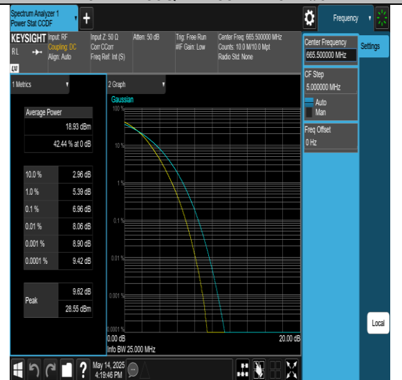
Band71-5MHz-256QAM-133297-25RB#0-PASS
