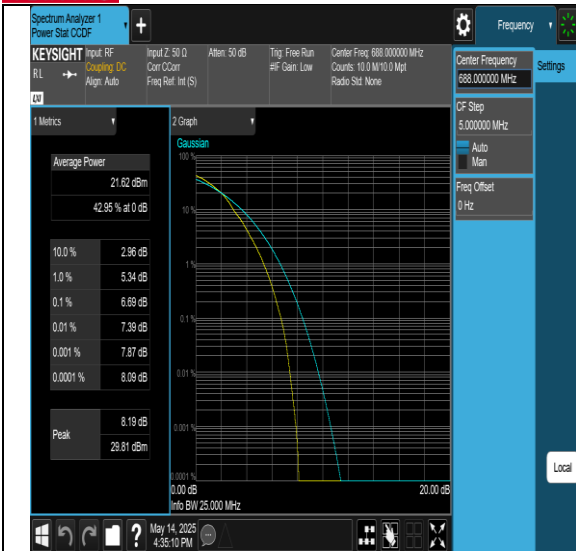
Band71-20MHz-256QAM-133222-1RB#0-PASS
