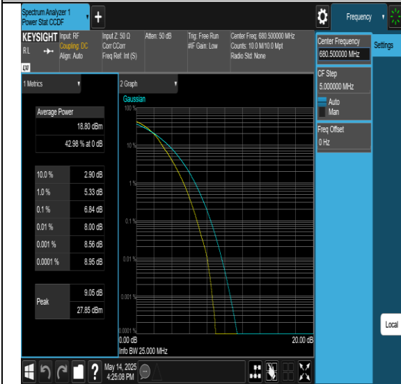
Band71-10MHz-256QAM-133422-1RB#0-PASS
