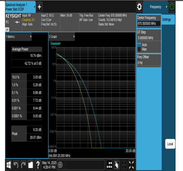
Band71-15MHz-256QAM-133297-75RB#0-PASS
