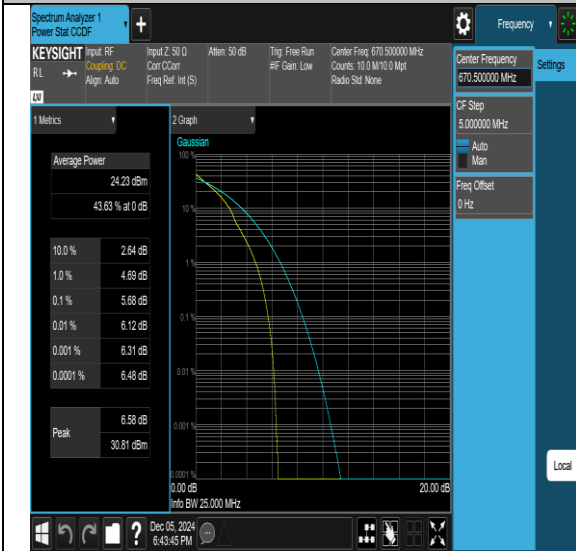
Band71-15MHz-QPSK-133297-1RB#0-PASS
