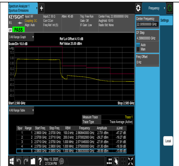
Band7-10MHz-256QAM-20800-50RB#0-PASS
