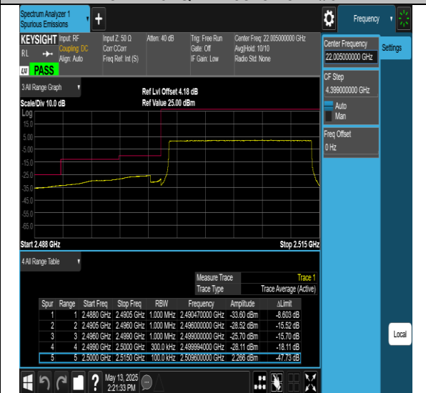
Band7-15MHz-64QAM-21375-75RB#0-PASS
