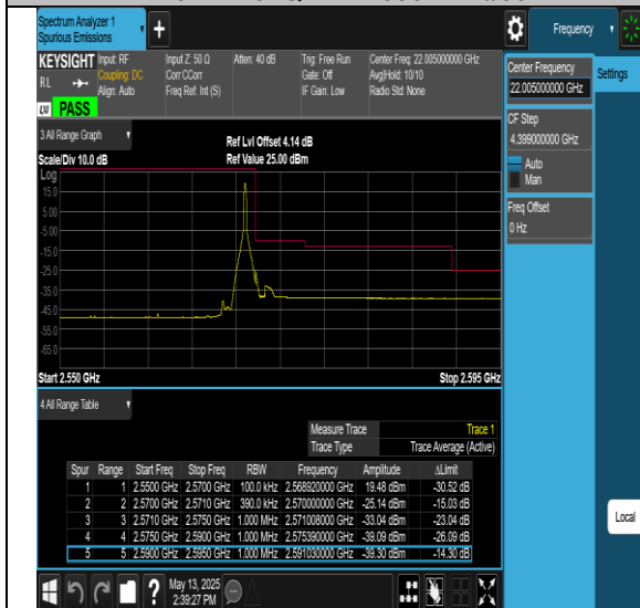
Band7-20MHz-256QAM-20850-1RB#0-PASS
