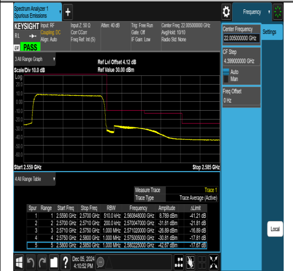
Band7-15MHz-QPSK-20825-75RB#0-PASS
