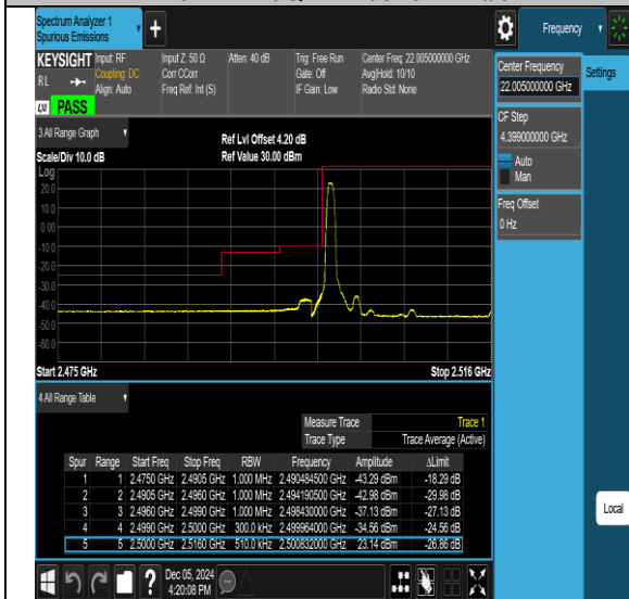
Band7-15MHz-16QAM-21375-1RB#74-PASS
