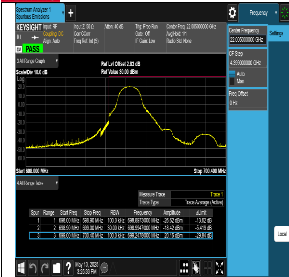
Band12-1.4MHz-64QAM-23173-1RB#5-PASS
