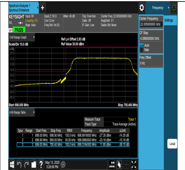
Band12-1.4MHz-64QAM-23173-6RB#0-PASS
