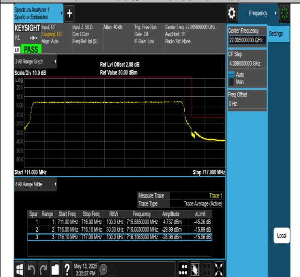
Band12-5MHz-16QAM-23035-25RB#0-PASS
