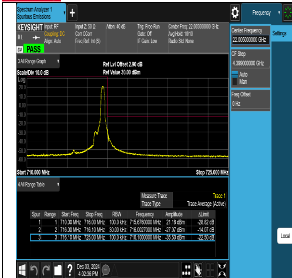
Band12-5MHz-64QAM-23035-1RB#0-PASS
