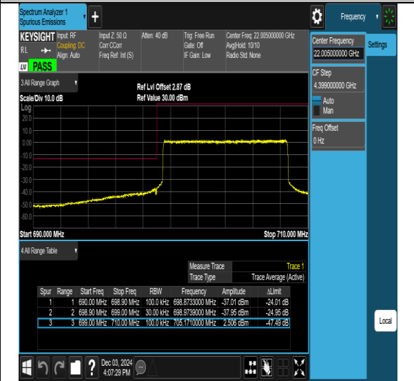
Band12-10MHz-QPSK-23130-50RB#0-PASS
