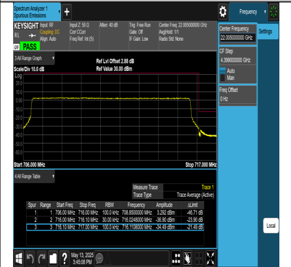
Band12-10MHz-256QAM-23060-50RB#0-PASS
