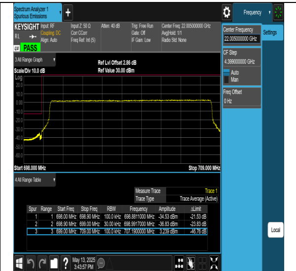
Band12-10MHz-64QAM-23130-50RB#0-PASS
