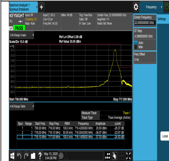
Band12-10MHz-256QAM-23060-1RB#0-PASS
