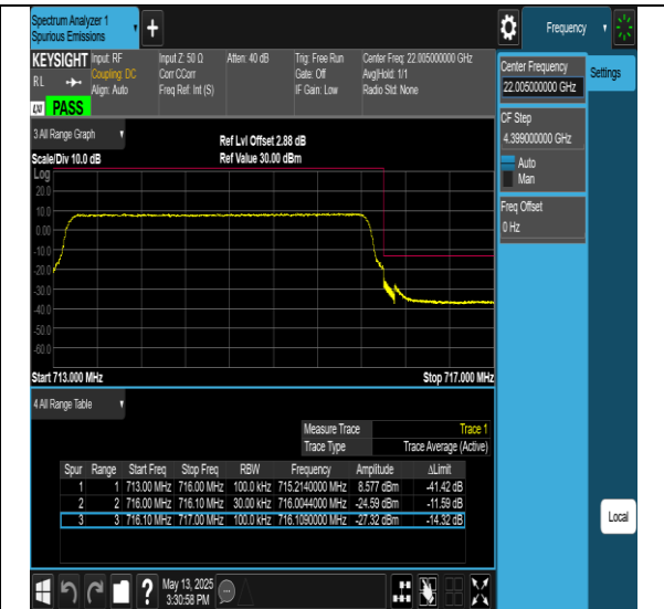
Band12-3MHz-256QAM-23025-15RB#0-PASS
