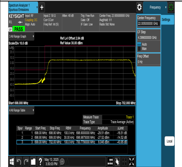
Band12-3MHz-256QAM-23165-15RB#0-PASS
