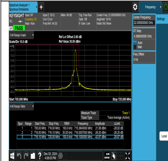
Band12-10MHz-64QAM-23060-1RB#0-PASS
