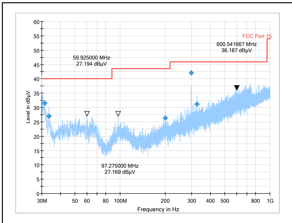
Plot: Above 30MHz – Active RFID
