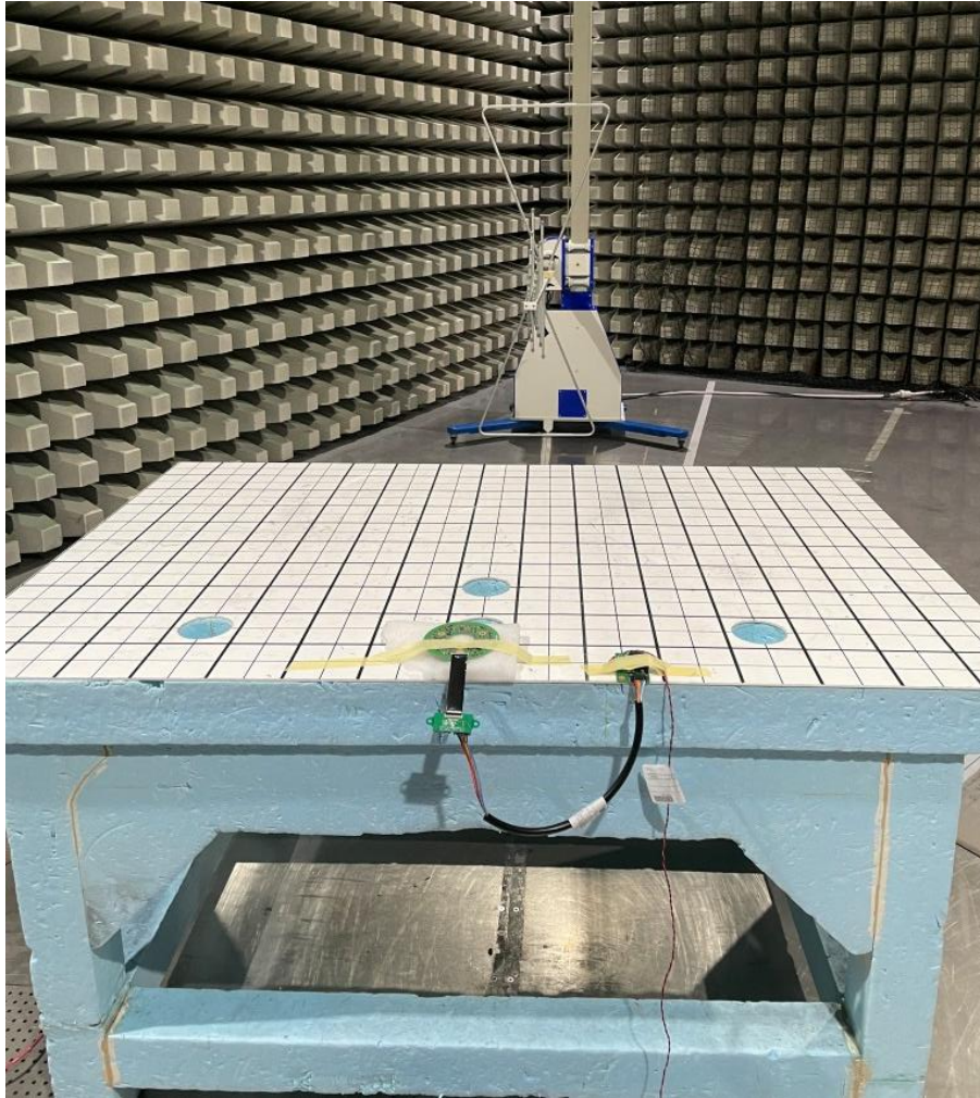
Photo 3 Radiated Test Setup from 30 MHz to 1 GHz
