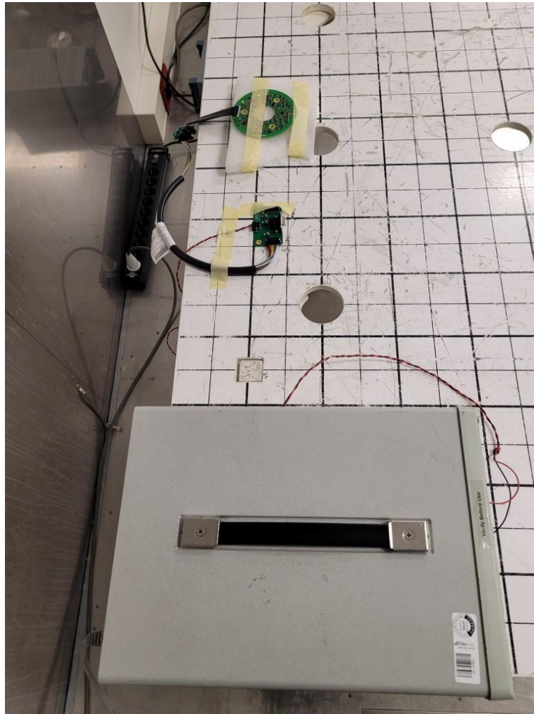
Photo 7 AC conducted emission
