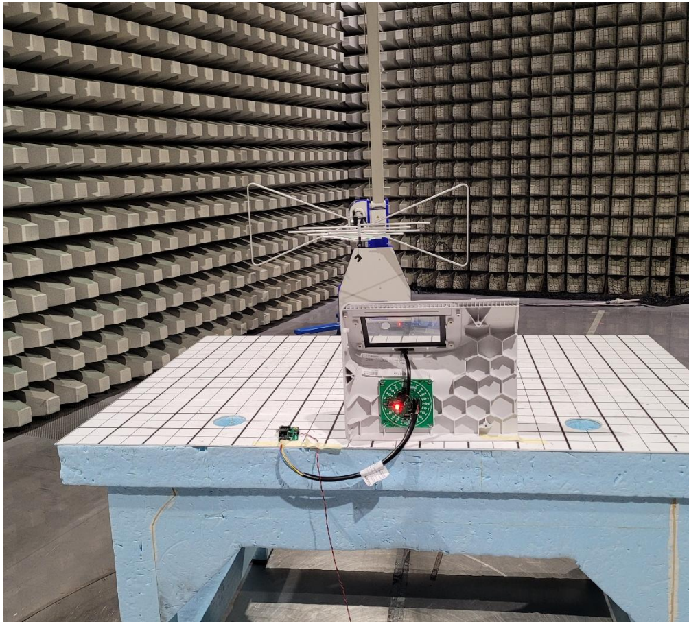
Photo 3 Radiated Test Setup from 30 MHz to 1 GHz
