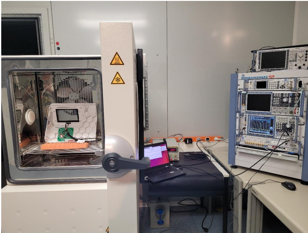
Photo 4 Bench test set up for (99% / 20 dB Bandwidth and Frequency Stability) (@ Ambient + Extreme Temperature, as required)
