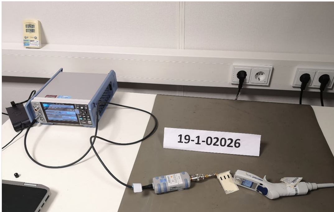
Photograph 7: Conducted Test Setup in the Radio Lab
