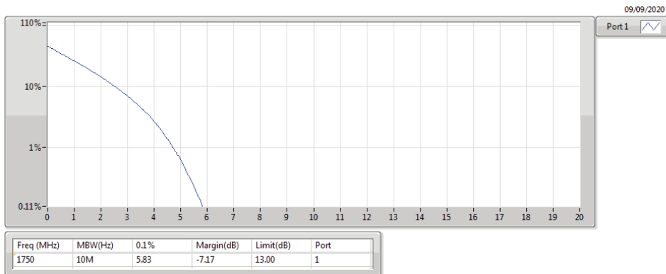
Band 4_LTE_10MHz_Nss1,QPSK_1TX 1750MHz_QPSK_RB 25,#RB M
