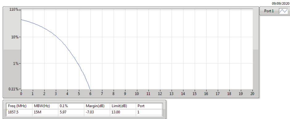
Band 2_LTE_15MHz_Nss1,16QAM_1TX 1857.5MHz_16QAM_RB 75,#RB 0
