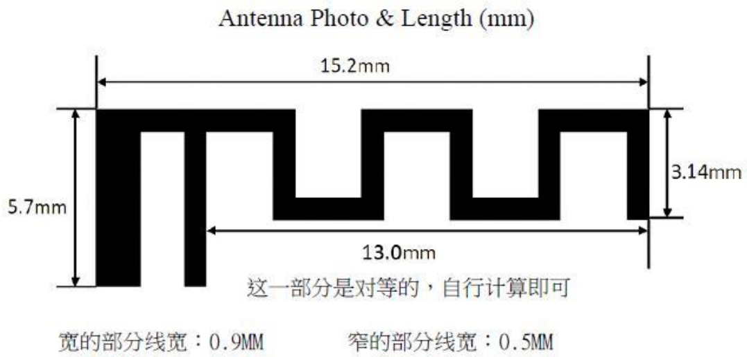
Figure 4: Antenna Dimensions
