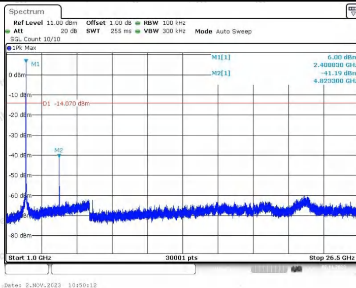
11B_Ant2_2412_0~Reference
