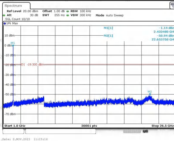
11N20SISO_Ant2_2437_0~Reference
