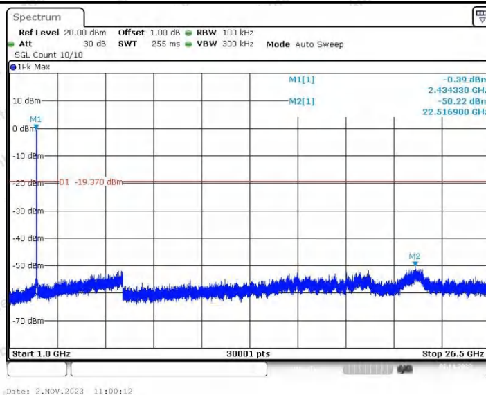
11G_Ant2_2437_0~Reference
