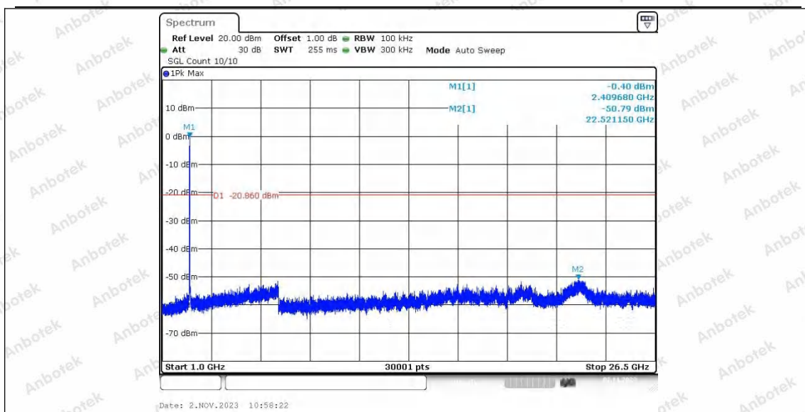
11G_Ant2_2412_0~Reference
