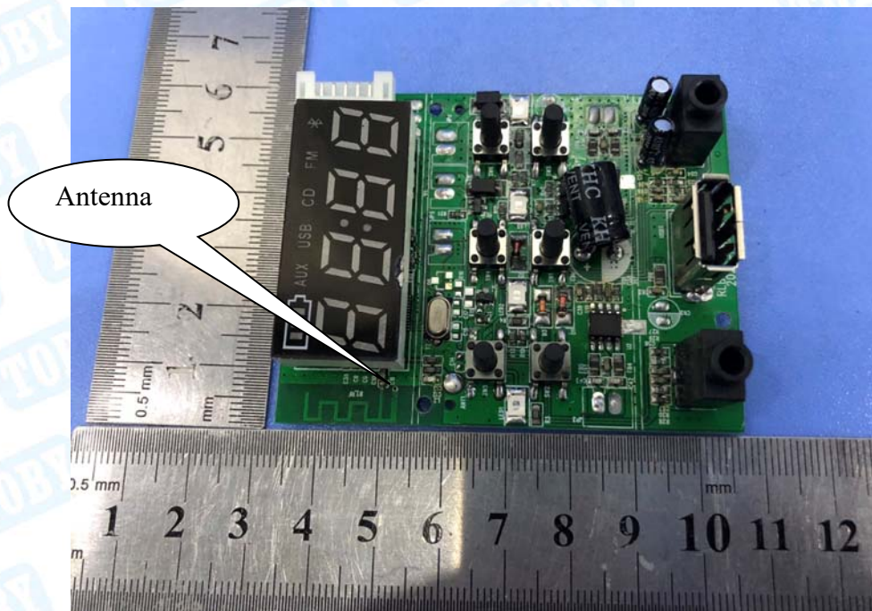
Photo 13 Internal of PCB
