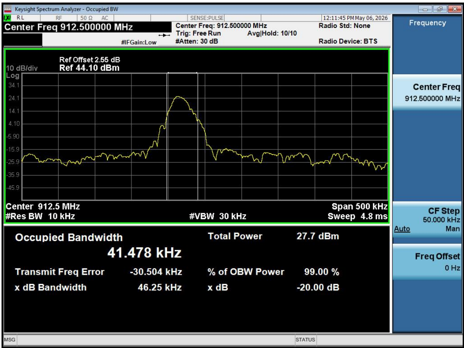
-20dB_Bandwidth_NVNT_ANT1_GFSK_912_50
