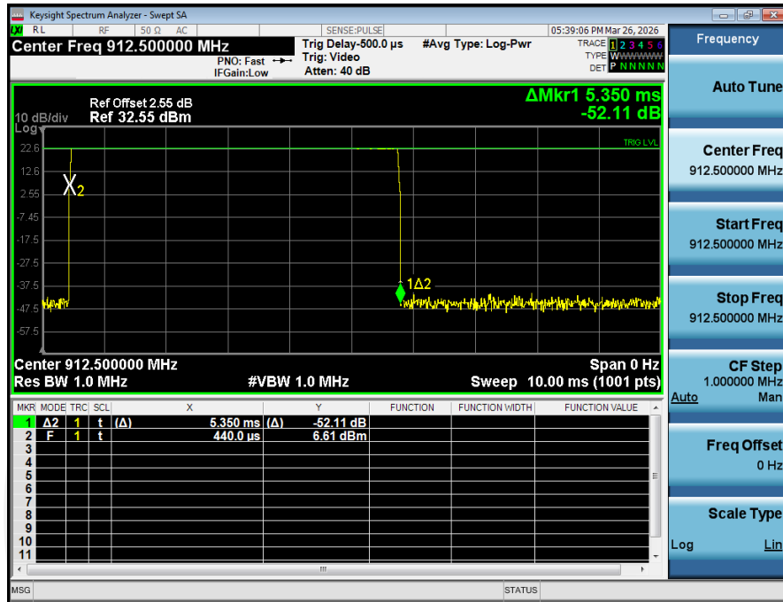
Dwell_Time_(Hopping)_NVNT_ANT1_GFSK_912_50_Accumulated
