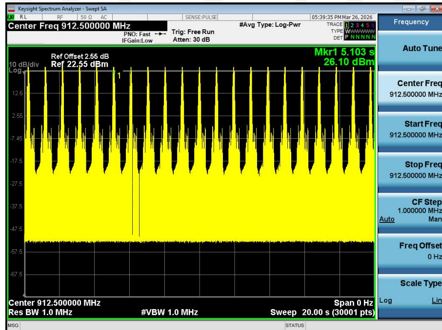
Dwell_Time_(Hopping)_NVNT_ANT1_GFSK_912_50_Accumulated
