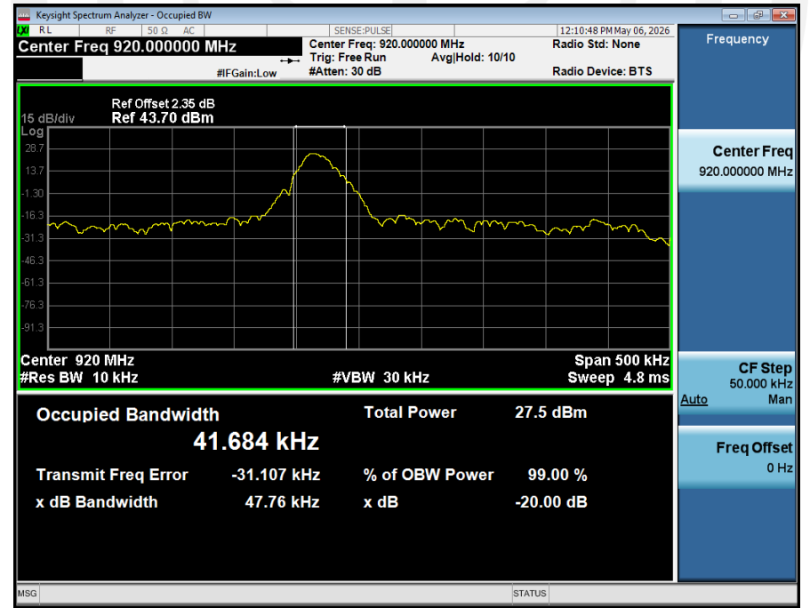
-20dB_Bandwidth_NVNT_ANT1_GFSK_920_00
