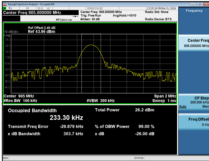
99% Occupied Bandwidth_NVNT_ANT1_GFSK_905_00
