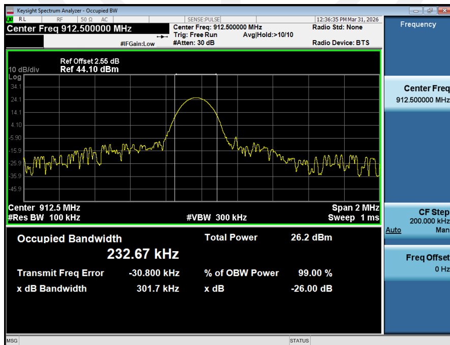
99% Occupied Bandwidth_NVNT_ANT1_GFSK_912_50
