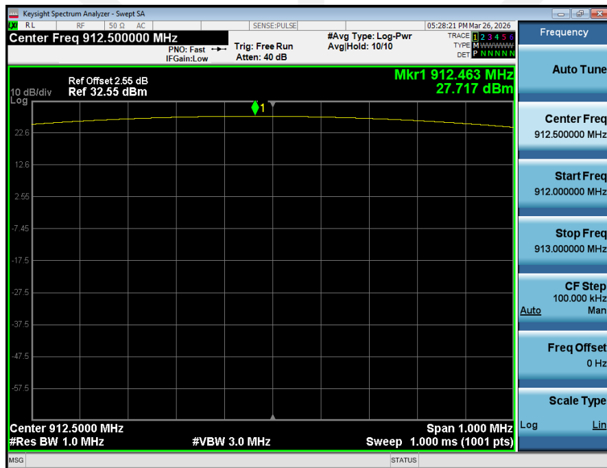
Peak_Output_Power_NVNT_ANT1_GFSK_912_50
