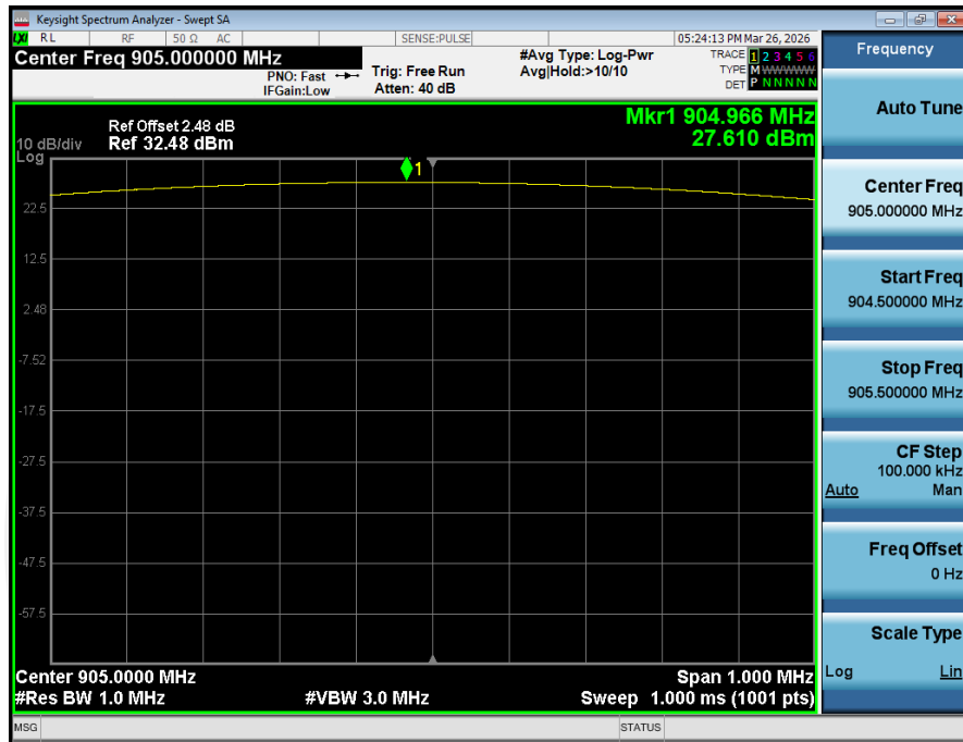
Peak_Output_Power_NVNT_ANT1_GFSK_905_00
